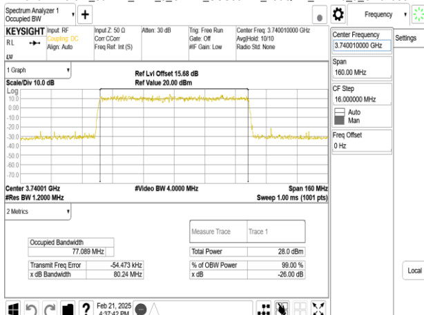
Band77-Part27_80MHz_DFT_s_OFDM_SCS30kHz_256QAM_RB216_0_CH649334
