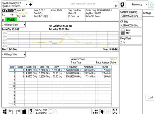
Band2_5MHz_DFT_s_OFDM_SCS15kHz_BPSK_RB1_0_CH370500
