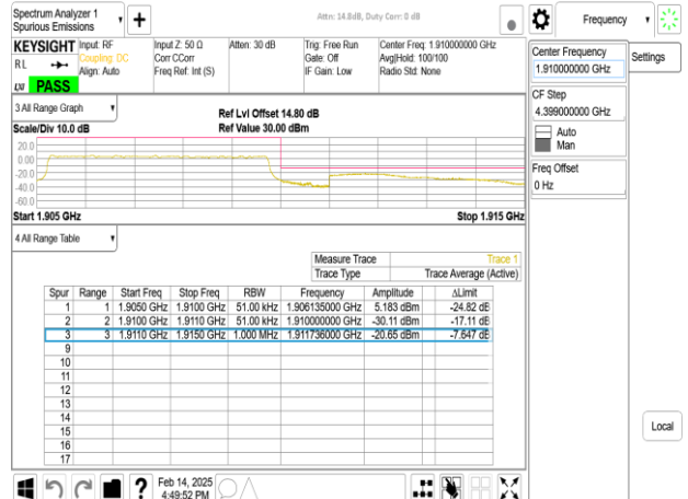
Band2_5MHz_DFT_s_OFDM_SCS15kHz_BPSK_RB25_0_CH381500
