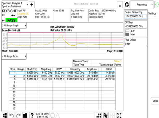
Band2_5MHz_CP_OFDM_SCS15kHz_QPSK_RB1_24_CH381500
