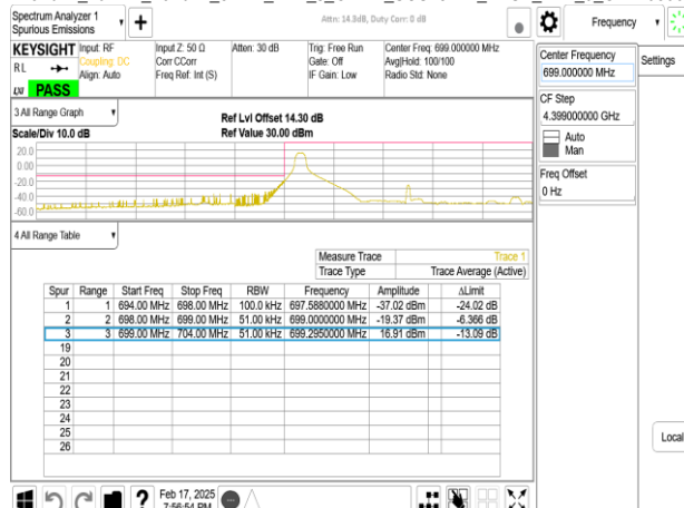
Band12_10MHz_Band12_5MHz_DFT_s_OFDM_SCS15kHz_BPSK_RB1_24_CH142700
