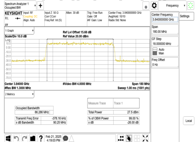
Band77-Part27_90MHz_DFT_s_OFDM_SCS30kHz_256QAM_RB243_0_CH662332
