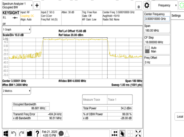
Band77-Part27_90MHz_DFT_s_OFDM_SCS30kHz_BPSK_RB243_0_CH633332
