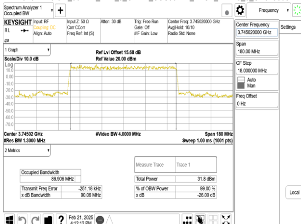
Band77-Part27_90MHz_DFT_s_OFDM_SCS30kHz_BPSK_RB243_0_CH649668
