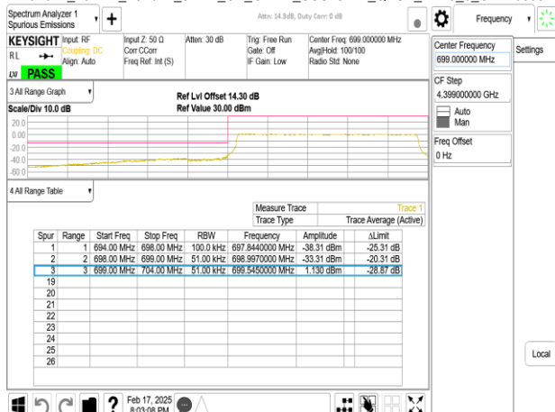
Band12_10MHz_Band12_5MHz_CP_OFDM_SCS15kHz_QPSK_RB25_0_CH140300
