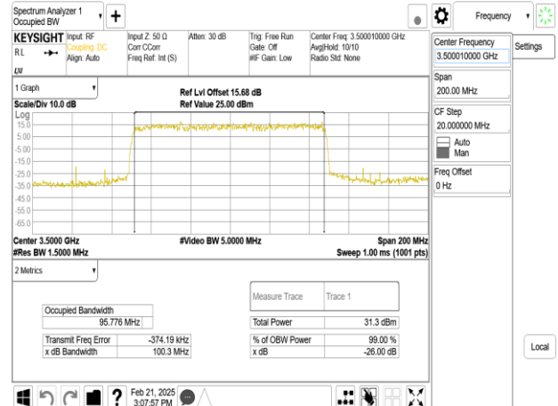
Band77-Part27_100MHz_DFT_s_OFDM_SCS30kHz_BPSK_RB270_0_CH633334
