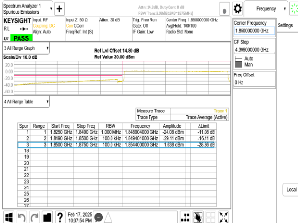
Band25_25MHz_CP_OFDM_SCS15kHz_QPSK_RB1_0_CH372500
