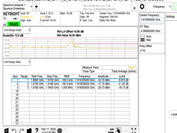
Band25_25MHz_DFT_s_OFDM_SCS15kHz_BPSK_RB1_132_CH380500
