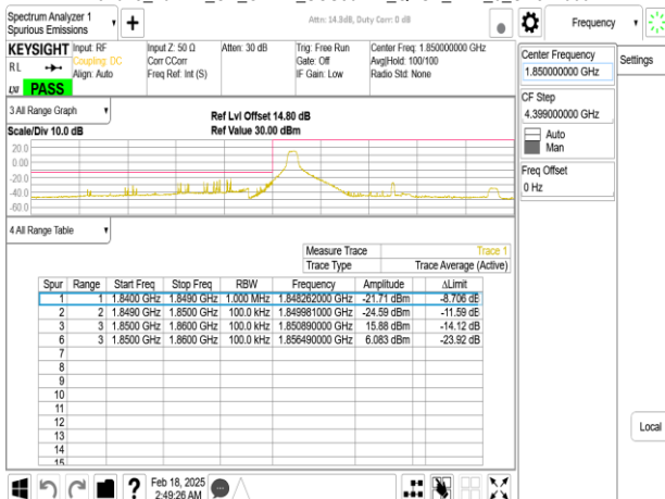
Band25_10MHz_CP_OFDM_SCS30kHz_QPSK_RB1_0_CH371000
