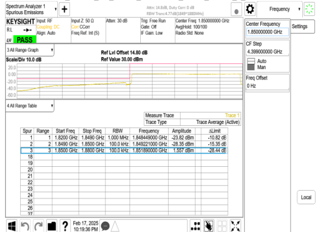
Band25_30MHz_CP_OFDM_SCS15kHz_QPSK_RB1_0_CH373000
