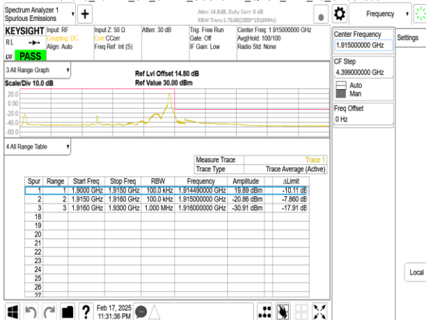
Band25_15MHz_CP_OFDM_SCS15kHz_QPSK_RB79_0_CH381500
