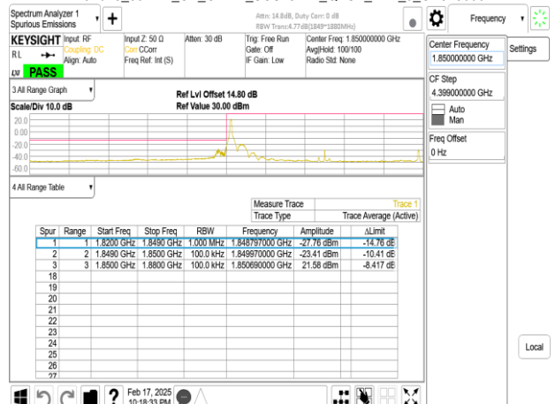
Band25_30MHz_CP_OFDM_SCS15kHz_QPSK_RB1_0_CH373000
