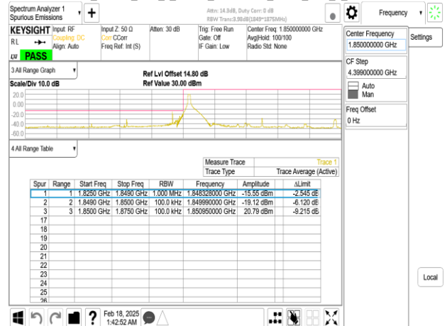
Band25_25MHz_DFT_s_OFDM_SCS30kHz_BPSK_RB64_0_CH372500
