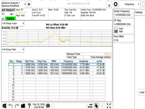
Band25_10MHz_DFT_s_OFDM_SCS30kHz_BPSK_RB24_0_CH382000
