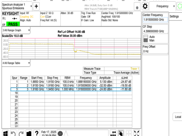
Band25_30MHz_DFT_s_OFDM_SCS15kHz_BPSK_RB160_0_CH380000
