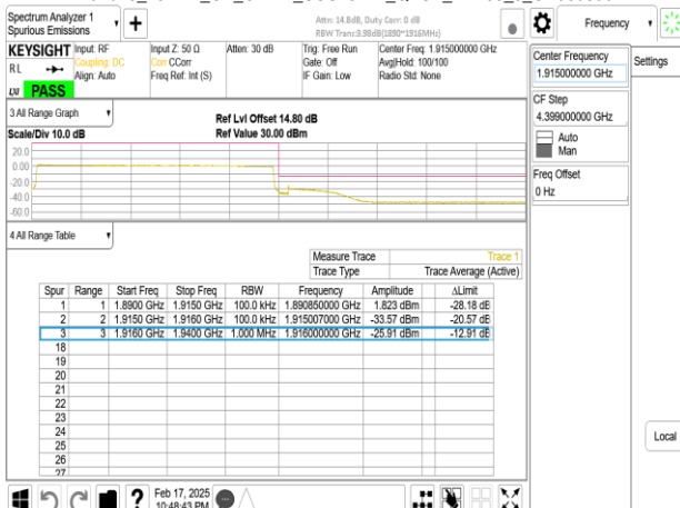
Band25_25MHz_CP_OFDM_SCS15kHz_QPSK_RB133_0_CH380500
