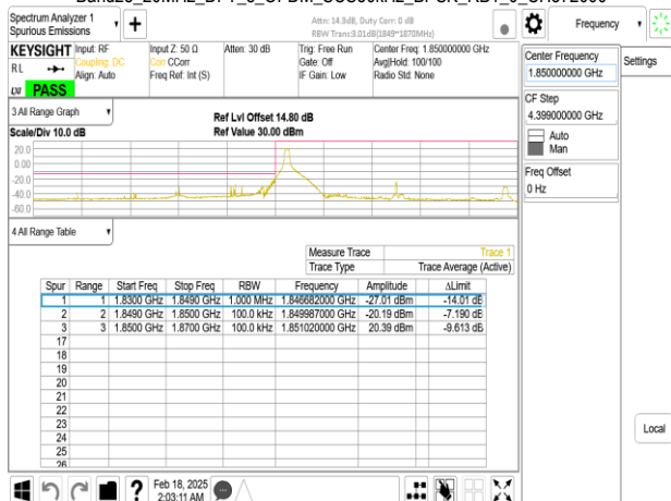
Band25_20MHz_DFT_s_OFDM_SCS30kHz_BPSK_RB50_0_CH372000
