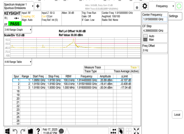
Band25_20MHz_CP_OFDM_SCS15kHz_QPSK_RB1_105_CH381000
