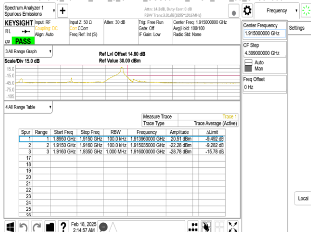
Band25_20MHz_DFT_s_OFDM_SCS30kHz_BPSK_RB1_50_CH381000
