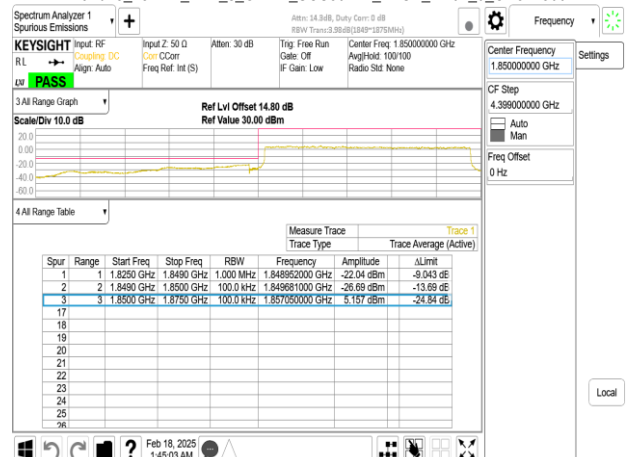
Band25_25MHz_DFT_s_OFDM_SCS30kHz_BPSK_RB64_0_CH372500
