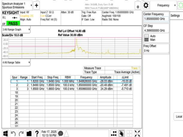
Band25_30MHz_DFT_s_OFDM_SCS15kHz_BPSK_RB160_0_CH380000
