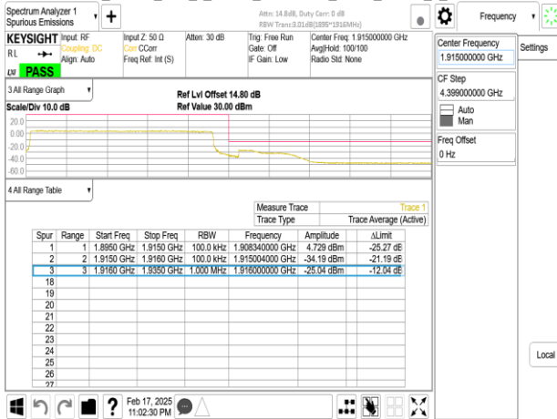
Band25_20MHz_DFT_s_OFDM_SCS15kHz_BPSK_RB1_105_CH381000
