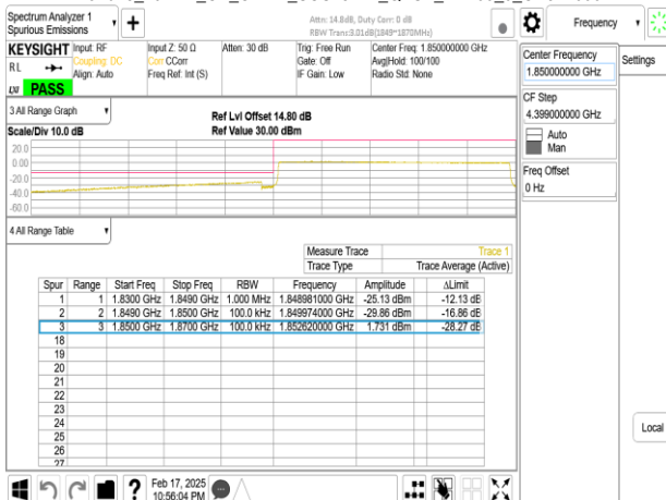
Band25_20MHz_CP_OFDM_SCS15kHz_QPSK_RB106_0_CH372000
