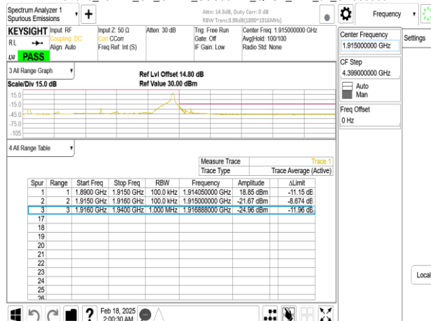
Band25_25MHz_CP_OFDM_SCS30kHz_QPSK_RB65_0_CH380500
