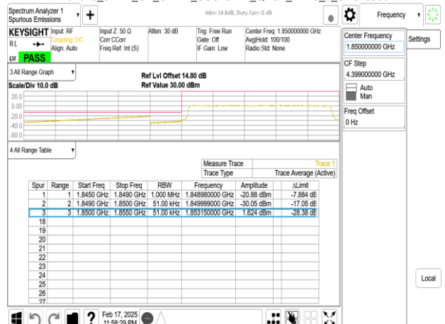
Band25_5MHz_CP_OFDM_SCS15kHz_QPSK_RB25_0_CH370500
