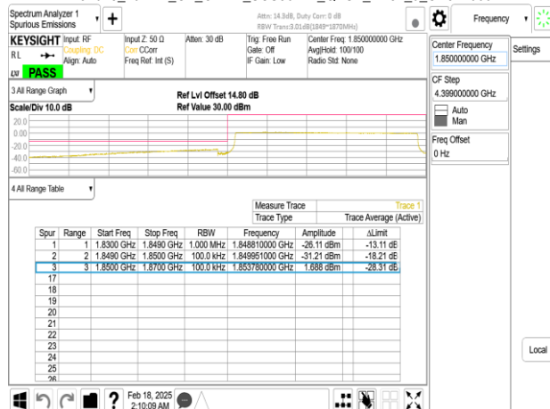
Band25_20MHz_CP_OFDM_SCS30kHz_QPSK_RB51_0_CH372000
