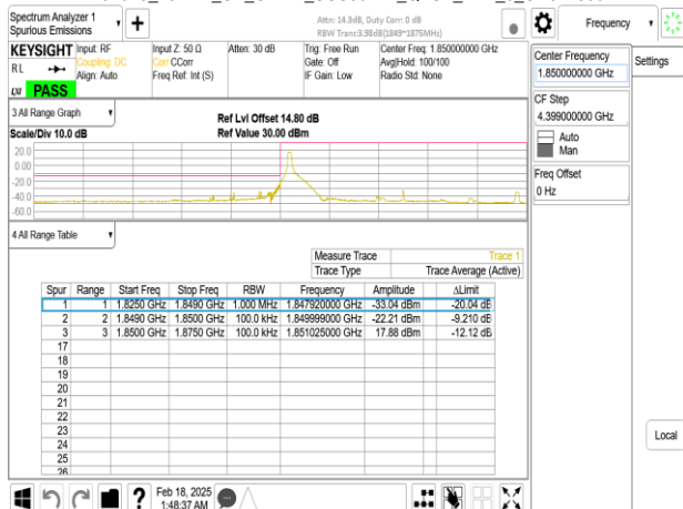
Band25_25MHz_CP_OFDM_SCS30kHz_QPSK_RB1_0_CH372500
