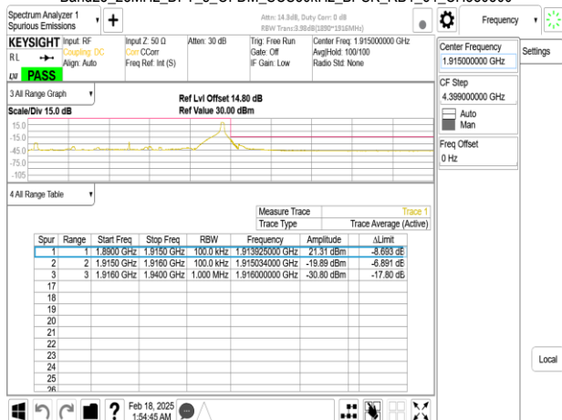
Band25_25MHz_DFT_s_OFDM_SCS30kHz_BPSK_RB64_0_CH380500
