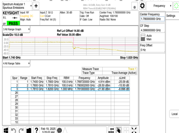
Band66_40MHz_CP_OFDM_SCS15kHz_QPSK_RB1_0_CH346000
