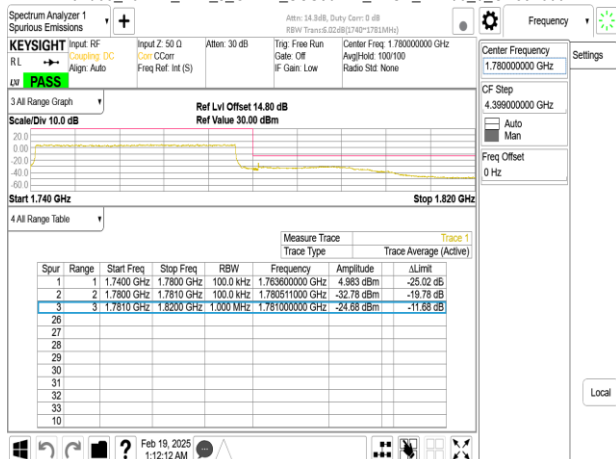
Band66_40MHz_DFT_s_OFDM_SCS30kHz_BPSK_RB100_0_CH352000
