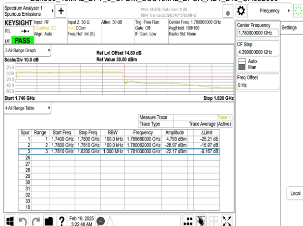
Band66_40MHz_DFT_s_OFDM_SCS15kHz_BPSK_RB216_0_CH352000
