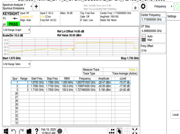
Band66_40MHz_DFT_s_OFDM_SCS30kHz_BPSK_RB1_0_CH346000
