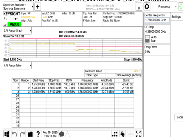
Band66_30MHz_CP_OFDM_SCS15kHz_QPSK_RB160_0_CH350000
