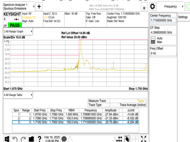
Band66_40MHz_CP_OFDM_SCS30kHz_QPSK_RB1_0_CH346000
