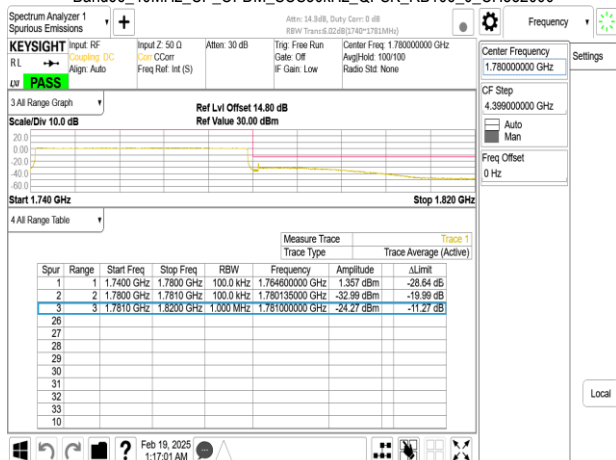
Band66_40MHz_CP_OFDM_SCS30kHz_QPSK_RB1_105_CH352000
