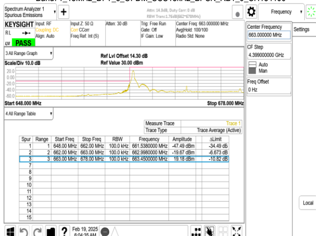
Band71_15MHz_DFT_s_OFDM_SCS15kHz_BPSK_RB1_0_CH134100
