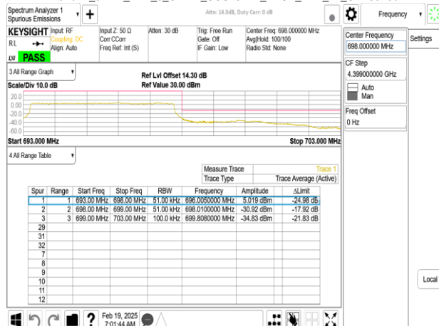
Band71_5MHz_DFT_s_OFDM_SCS15kHz_BPSK_RB25_0_CH139100
