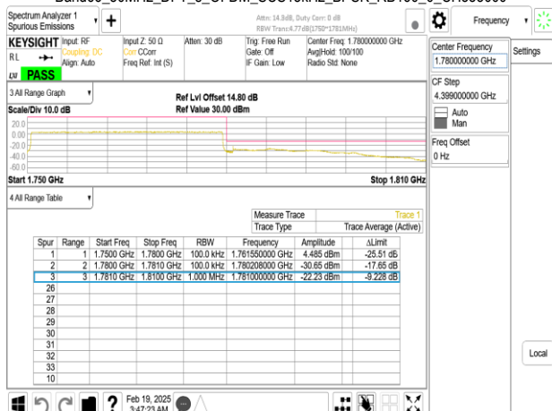
Band66_30MHz_DFT_s_OFDM_SCS15kHz_BPSK_RB160_0_CH353000
