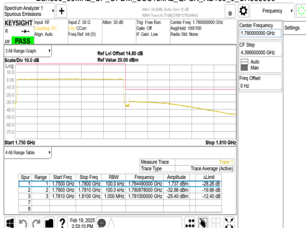
Band66_30MHz_CP_OFDM_SCS15kHz_QPSK_RB1_159_CH353000
