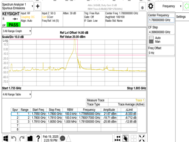
Band66_25MHz_DFT_s_OFDM_SCS30kHz_BPSK_RB64_0_CH353500
