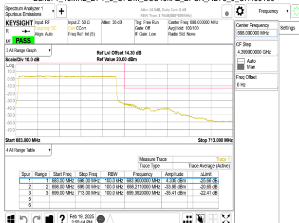
Band71_15MHz_DFT_s_OFDM_SCS15kHz_BPSK_RB75_0_CH138100
