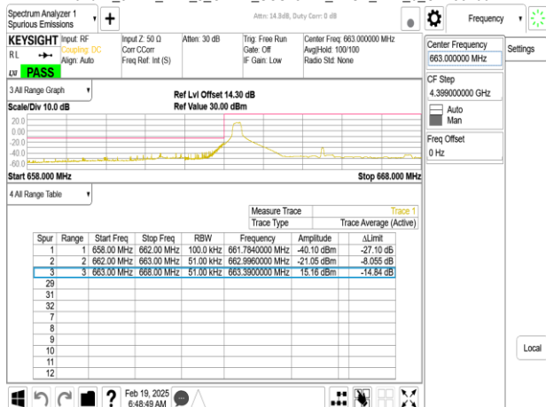
Band71_5MHz_DFT_s_OFDM_SCS15kHz_BPSK_RB1_0_CH1313100
