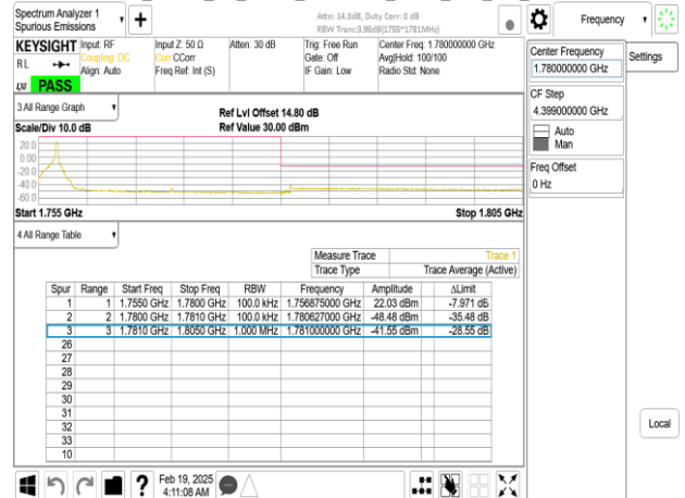
Band66_25MHz_DFT_s_OFDM_SCS30kHz_BPSK_RB1_0_CH344500
