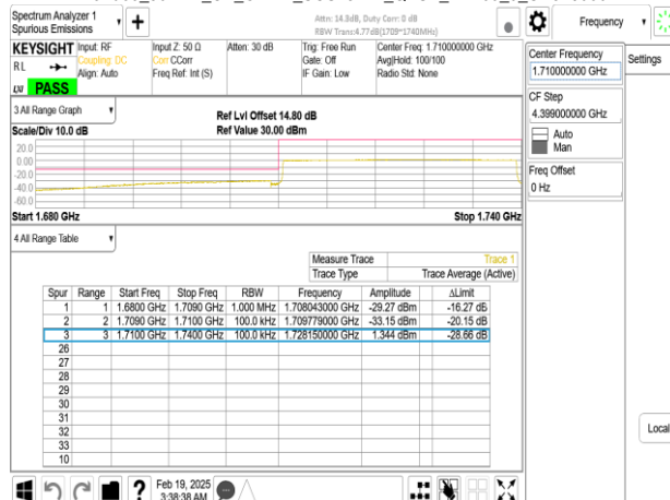
Band66_30MHz_CP_OFDM_SCS15kHz_QPSK_RB1_0_CH345000
