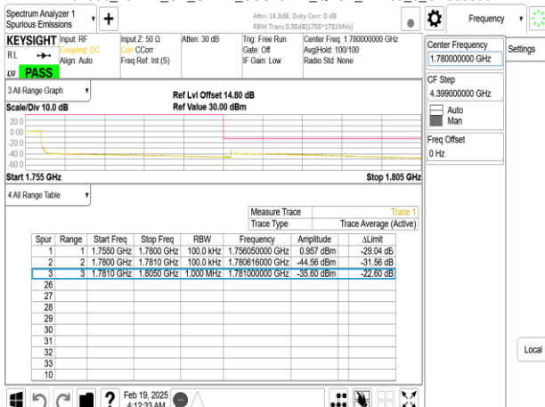
Band66_25MHz_CP_OFDM_SCS15kHz_QPSK_RB133_0_CH353500
