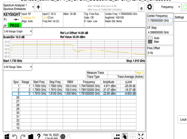
Band66_30MHz_DFT_s_OFDM_SCS30kHz_BPSK_RB75_0_CH353000
