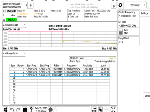
Band66_40MHz_CP_OFDM_SCS15kHz_QPSK_RB216_0_CH352000
