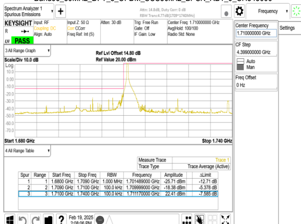
Band66_30MHz_DFT_s_OFDM_SCS30kHz_BPSK_RB1_0_CH345000
