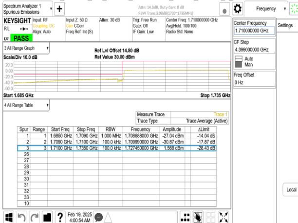
Band66_25MHz_CP_OFDM_SCS15kHz_QPSK_RB1_0_CH344500
