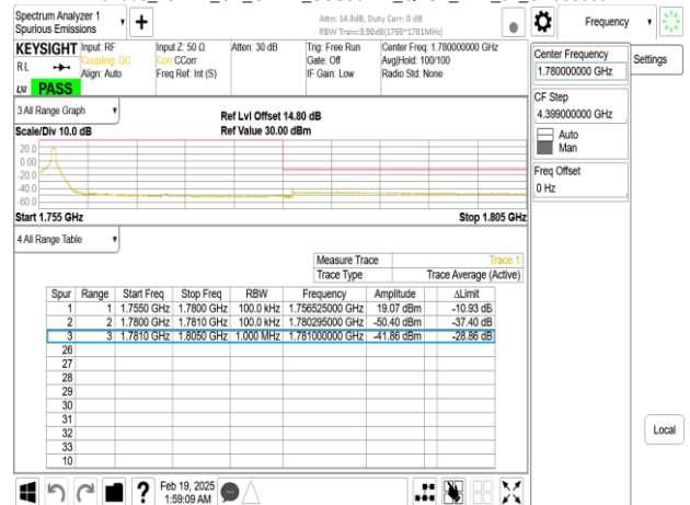
Band66_25MHz_CP_OFDM_SCS30kHz_QPSK_RB65_0_CH353500
