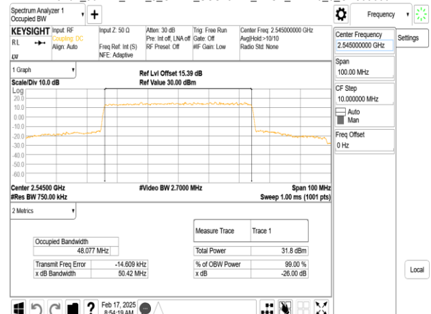
Band7_50MHz_DFT_s_OFDM_SCS15kHz_BPSK_RB270_0_CH509000
