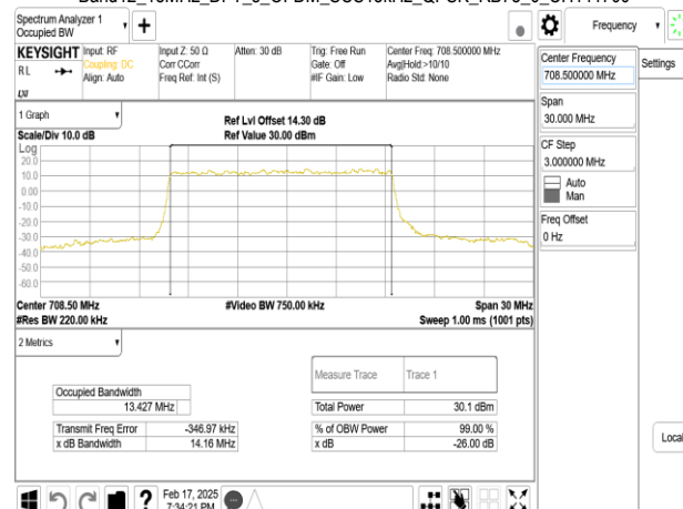
Band12_15MHz_DFT_s_OFDM_SCS15kHz_QPSK_RB75_0_CH141700
