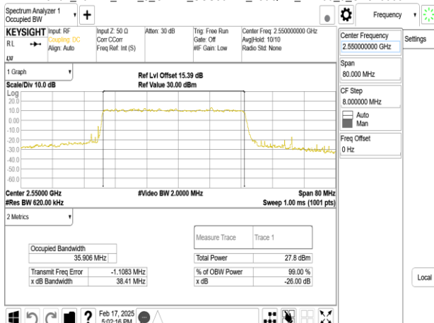
Band7_40MHz_DFT_s_OFDM_SCS30kHz_256QAM_RB100_0_CH510000
