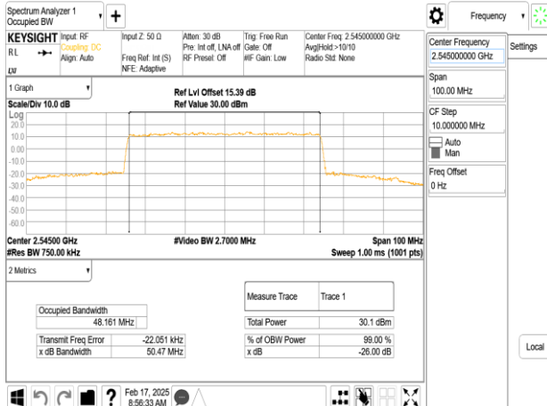
Band7_50MHz_DFT_s_OFDM_SCS15kHz_64QAM_RB270_0_CH509000
