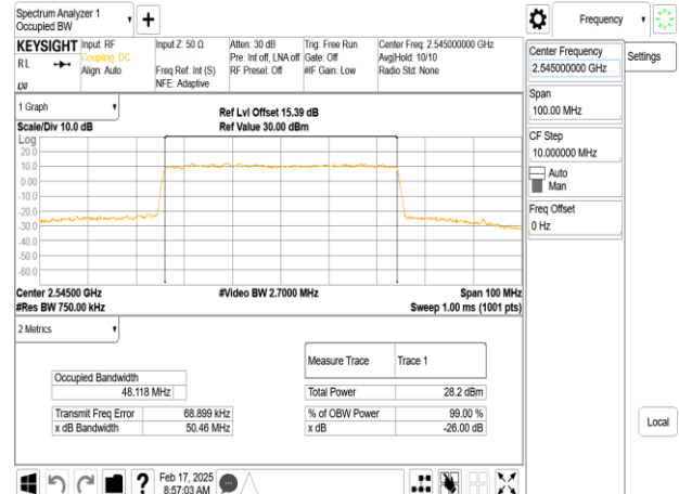
Band7_50MHz_DFT_s_OFDM_SCS15kHz_256QAM_RB270_0_CH509000
