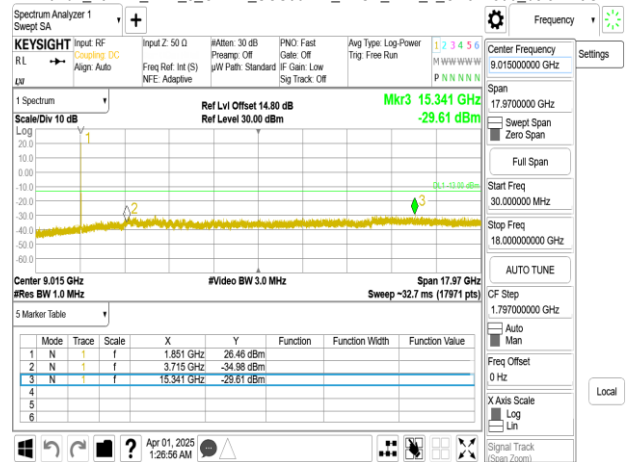
Band2_15MHz_DFT_s_OFDM_SCS30kHz_BPSK_RB1_1_CH376000_below 18G
