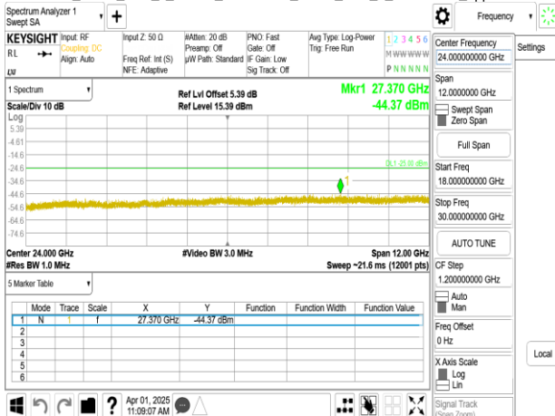
Band7_5MHz_DFT_s_OFDM_SCS15kHz_BPSK_RB1_1_CH513500_upper 18G
