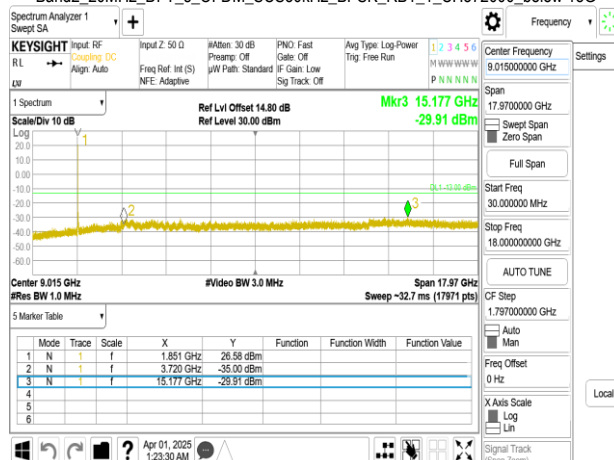
Band2_20MHz_DFT_s_OFDM_SCS30kHz_BPSK_RB1_1_CH376000_below 18G
