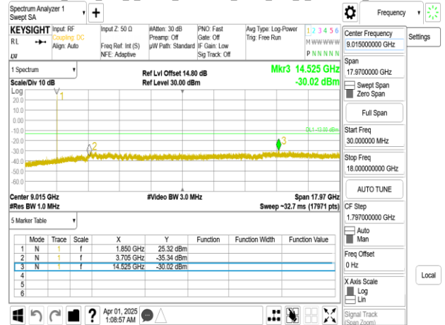
Band2_5MHz_DFT_s_OFDM_SCS15kHz_BPSK_RB1_1_CH376000_below 18G
