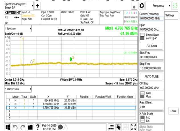
Band5_20MHz_DFT_s_OFDM_SCS15kHz_BPSK_RB1_1_CH167300
