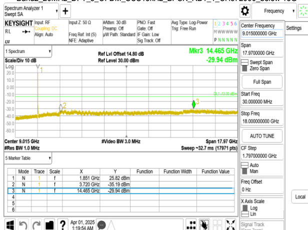
Band2_20MHz_DFT_s_OFDM_SCS15kHz_BPSK_RB1_1_CH376000_below 18G
