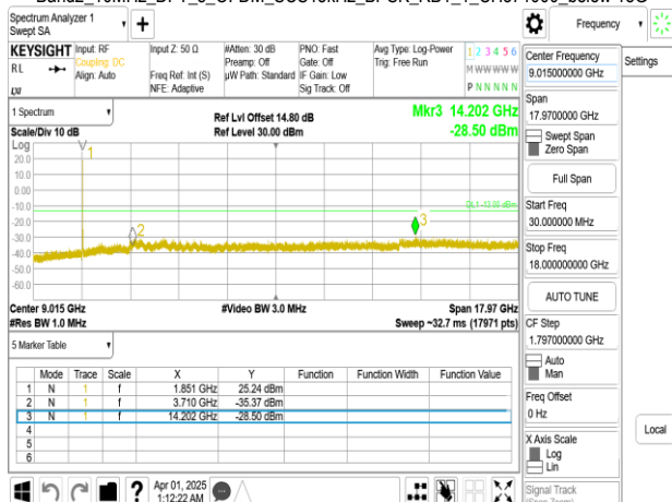
Band2_10MHz_DFT_s_OFDM_SCS15kHz_BPSK_RB1_1_CH376000_below 18G
