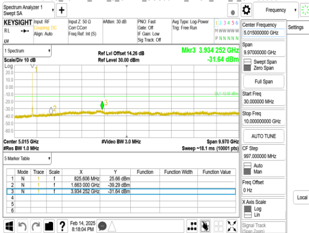
Band5_15MHz_DFT_s_OFDM_SCS30kHz_BPSK_RB1_1_CH167300
