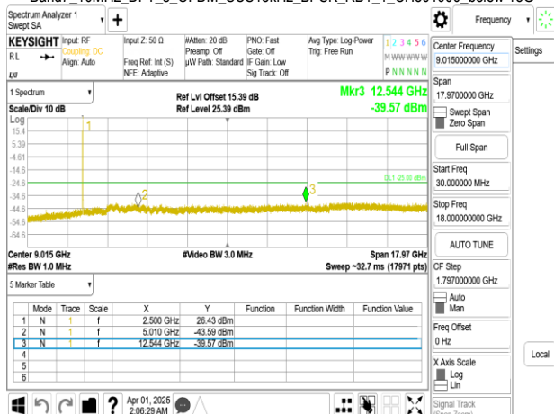
Band7_10MHz_DFT_s_OFDM_SCS15kHz_BPSK_RB1_1_CH507000_below 18G
