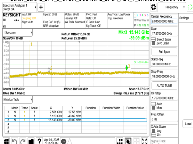
Band7_20MHz_DFT_s_OFDM_SCS15kHz_BPSK_RB1_1_CH512000_below 18G
