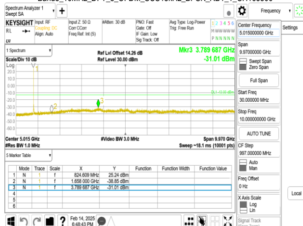
Band5_10MHz_DFT_s_OFDM_SCS15kHz_BPSK_RB1_1_CH167300
