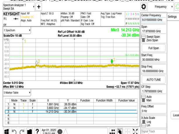
Band2_20MHz_DFT_s_OFDM_SCS30kHz_BPSK_RB1_1_CH380000_below 18G
