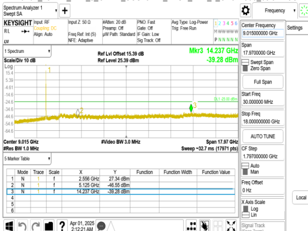
Band7_15MHz_DFT_s_OFDM_SCS15kHz_BPSK_RB1_1_CH512500_below 18G
