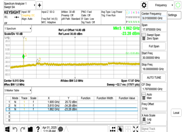
Band2_5MHz_DFT_s_OFDM_SCS15kHz_BPSK_RB1_1_CH381500_below 18G
