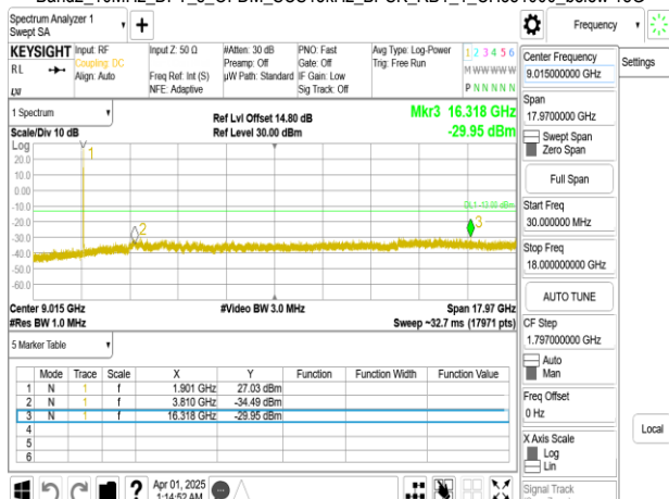
Band2_10MHz_DFT_s_OFDM_SCS15kHz_BPSK_RB1_1_CH381000_below 18G
