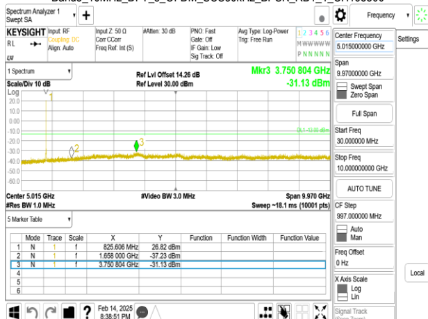
Band5_10MHz_DFT_s_OFDM_SCS30kHz_BPSK_RB1_1_CH167300
