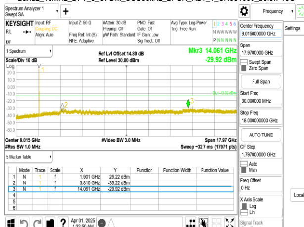
Band2_10MHz_DFT_s_OFDM_SCS30kHz_BPSK_RB1_1_CH381000_below 18G
