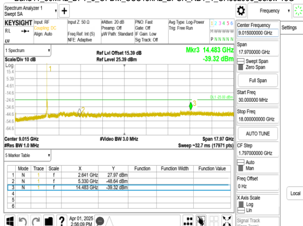
Band41_50MHz_DFT_s_OFDM_SCS30kHz_BPSK_RB1_1_CH504204_below 18G
