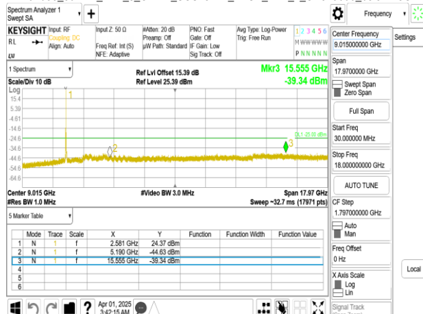
Band38_30MHz_DFT_s_OFDM_SCS15kHz_BPSK_RB1_1_CH521000_below 18G
