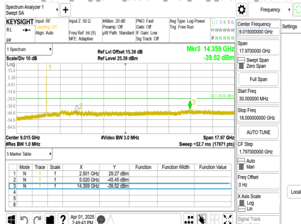
Band41_20MHz_DFT_s_OFDM_SCS15kHz_BPSK_RB1_1_CH518604_below 18G
