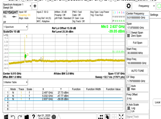
Band41_40MHz_DFT_s_OFDM_SCS30kHz_BPSK_RB1_1_CH503202_below 18G
