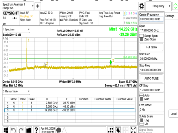
Band41_50MHz_DFT_s_OFDM_SCS30kHz_BPSK_RB1_1_CH505002_below 18G
