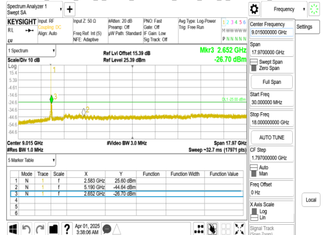
Band38_25MHz_DFT_s_OFDM_SCS15kHz_BPSK_RB1_1_CH521500_below 18G
