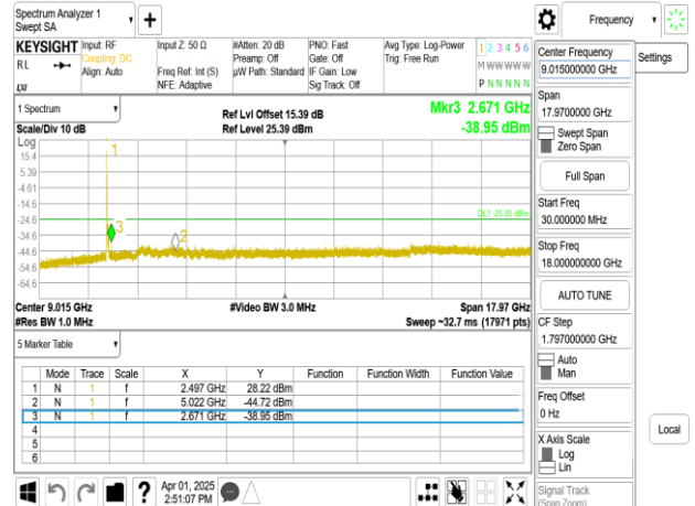
Band41_30MHz_DFT_s_OFDM_SCS15kHz_BPSK_RB1_1_CH502200_below 18G
