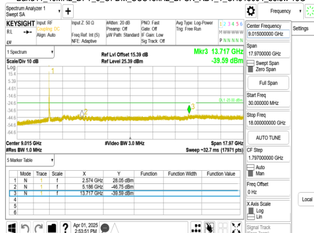
Band41_40MHz_DFT_s_OFDM_SCS15kHz_BPSK_RB1_1_CH534000_below 18G
