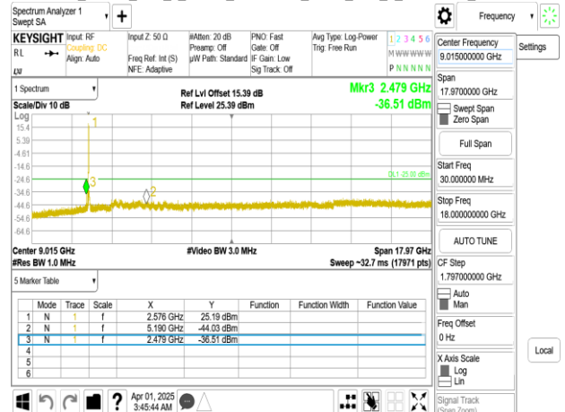
Band38_40MHz_DFT_s_OFDM_SCS15kHz_BPSK_RB1_1_CH520000_below 18G
