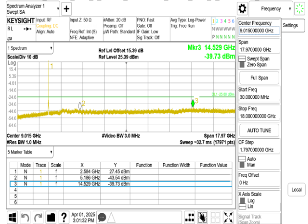
Band41_20MHz_DFT_s_OFDM_SCS30kHz_BPSK_RB1_1_CH535998_below 18G
