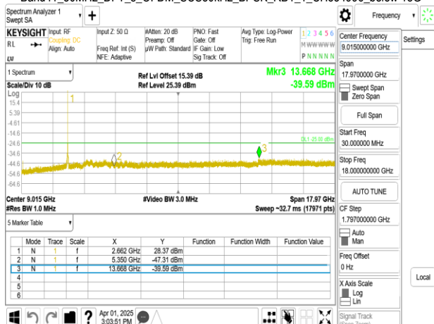
Band41_40MHz_DFT_s_OFDM_SCS15kHz_BPSK_RB1_1_CH503202_below 18G
