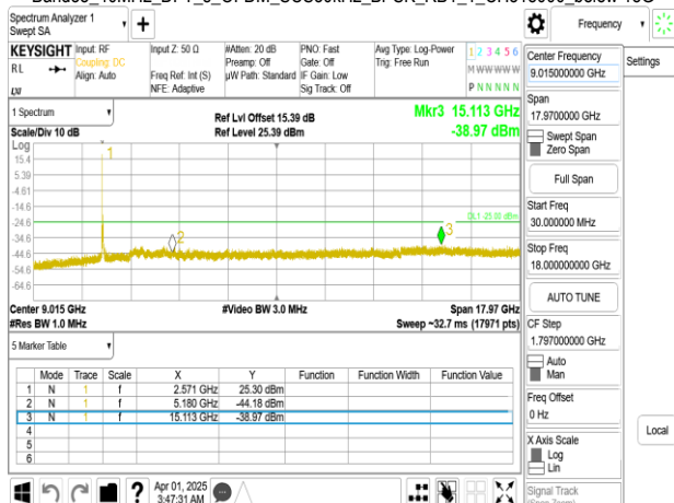
Band38_40MHz_DFT_s_OFDM_SCS30kHz_BPSK_RB1_1_CH519000_below 18G
