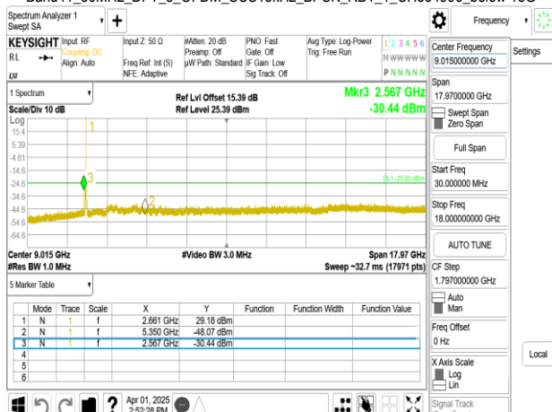
Band41_30MHz_DFT_s_OFDM_SCS15kHz_BPSK_RB1_1_CH534996_below 18G
