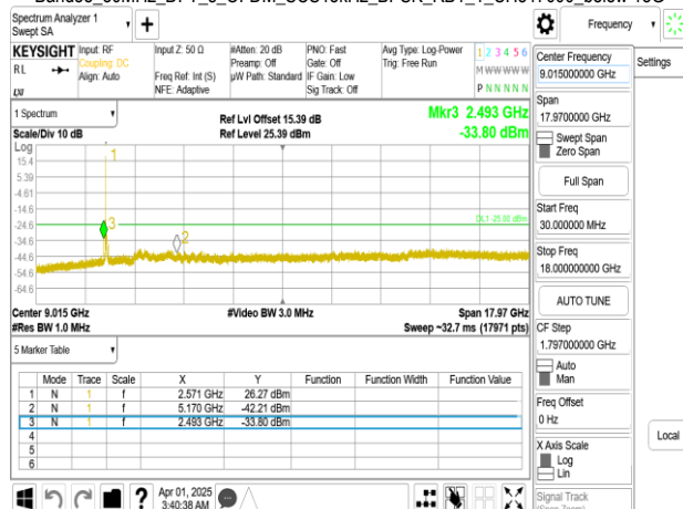
Band38_30MHz_DFT_s_OFDM_SCS15kHz_BPSK_RB1_1_CH519000_below 18G
