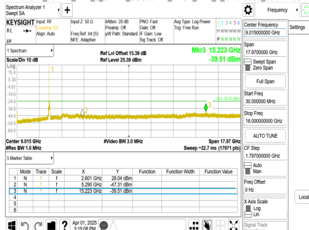
Band41_100MHz_DFT_s_OFDM_SCS30kHz_BPSK_RB1_1_CH509202_below 18G
