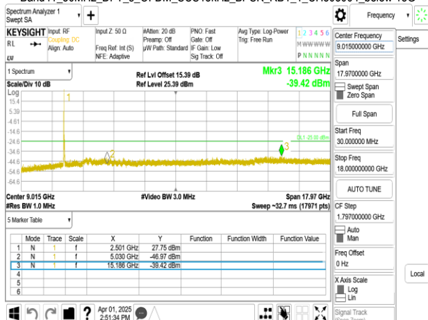
Band41_30MHz_DFT_s_OFDM_SCS15kHz_BPSK_RB1_1_CH518604_below 18G
