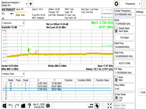
Band41_20MHz_DFT_s_OFDM_SCS30kHz_BPSK_RB1_1_CH502002_below 18G
