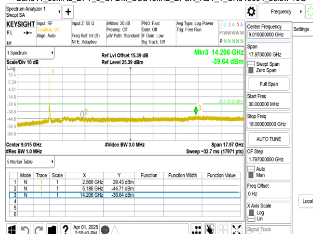
Band41_50MHz_DFT_s_OFDM_SCS15kHz_BPSK_RB1_1_CH518604_below 18G
