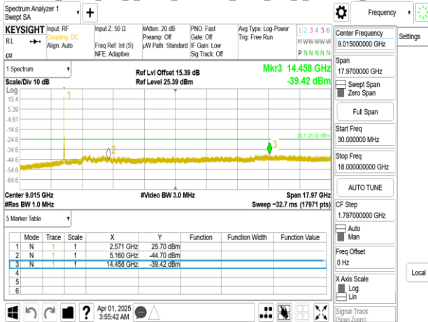
Band38_20MHz_DFT_s_OFDM_SCS30kHz_BPSK_RB1_1_CH519000_below 18G
