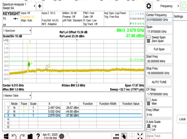
Band41_40MHz_DFT_s_OFDM_SCS15kHz_BPSK_RB1_1_CH504000_below 18G
