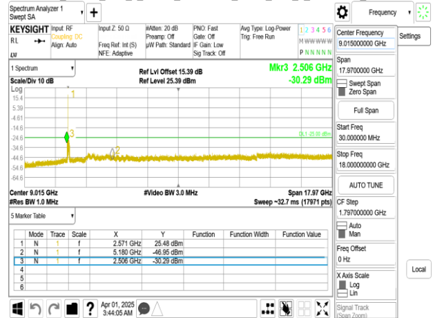
Band38_40MHz_DFT_s_OFDM_SCS15kHz_BPSK_RB1_1_CH519000_below 18G
