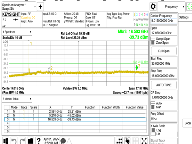
Band38_30MHz_DFT_s_OFDM_SCS30kHz_BPSK_RB1_1_CH521000_below 18G
