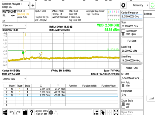
Band38_40MHz_DFT_s_OFDM_SCS30kHz_BPSK_RB1_1_CH520000_below 18G
