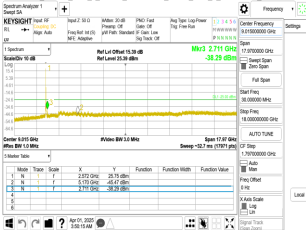
Band38_30MHz_DFT_s_OFDM_SCS30kHz_BPSK_RB1_1_CH519000_below 18G
