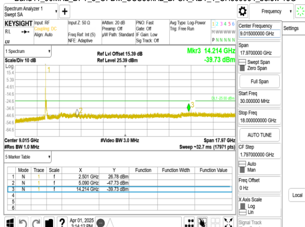
Band41_90MHz_DFT_s_OFDM_SCS30kHz_BPSK_RB1_1_CH509004_below 18G
