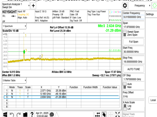
Band38_25MHz_DFT_s_OFDM_SCS30kHz_BPSK_RB1_1_CH519000_below 18G
