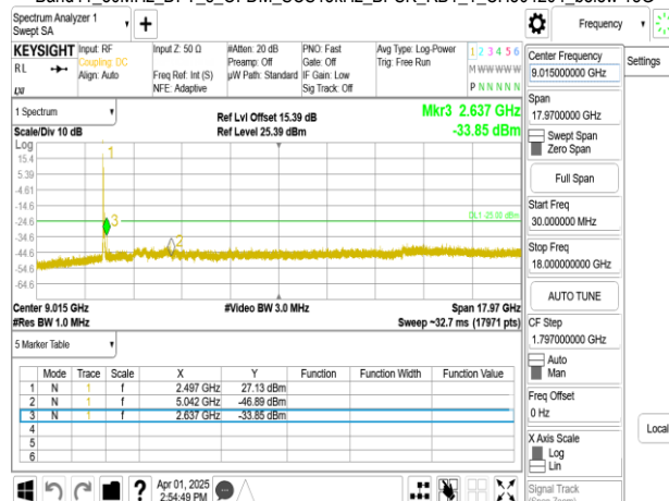
Band41_50MHz_DFT_s_OFDM_SCS15kHz_BPSK_RB1_1_CH505002_below 18G
