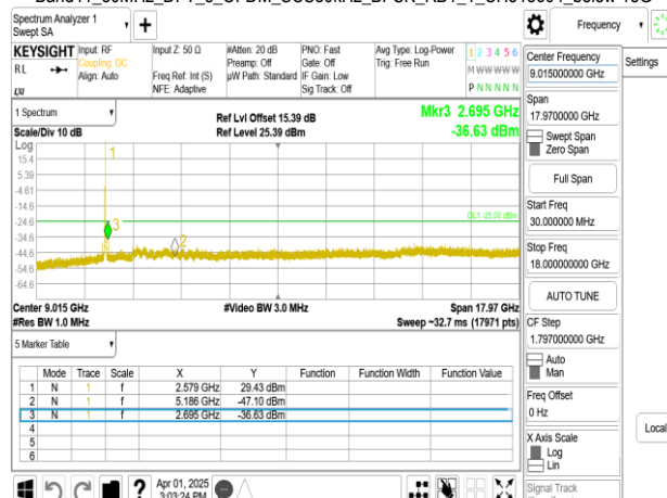
Band41_30MHz_DFT_s_OFDM_SCS30kHz_BPSK_RB1_1_CH518604_below 18G
