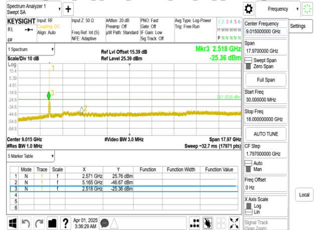
Band38_25MHz_DFT_s_OFDM_SCS15kHz_BPSK_RB1_1_CH519000_below 18G
