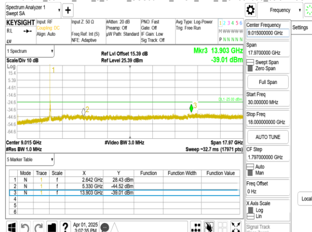
Band41_60MHz_DFT_s_OFDM_SCS30kHz_BPSK_RB1_1_CH505200_below 18G
