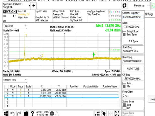
Band41_50MHz_DFT_s_OFDM_SCS30kHz_BPSK_RB1_1_CH532998_below 18G
