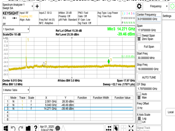
Band41_40MHz_DFT_s_OFDM_SCS30kHz_BPSK_RB1_1_CH518604_below 18G
