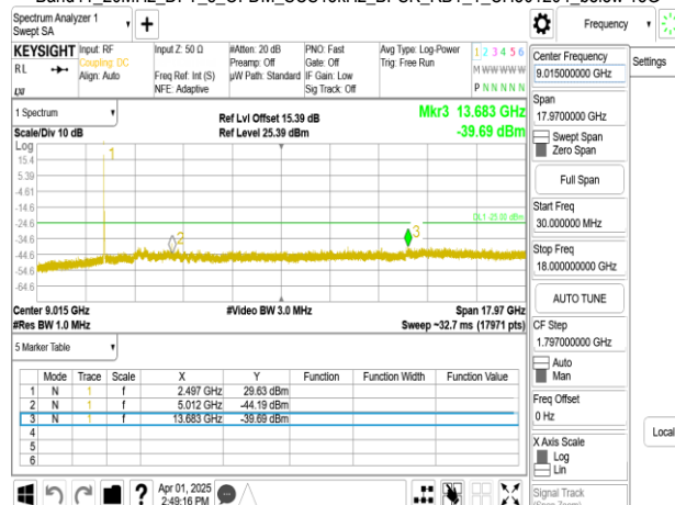
Band41_20MHz_DFT_s_OFDM_SCS15kHz_BPSK_RB1_1_CH502002_below 18G
