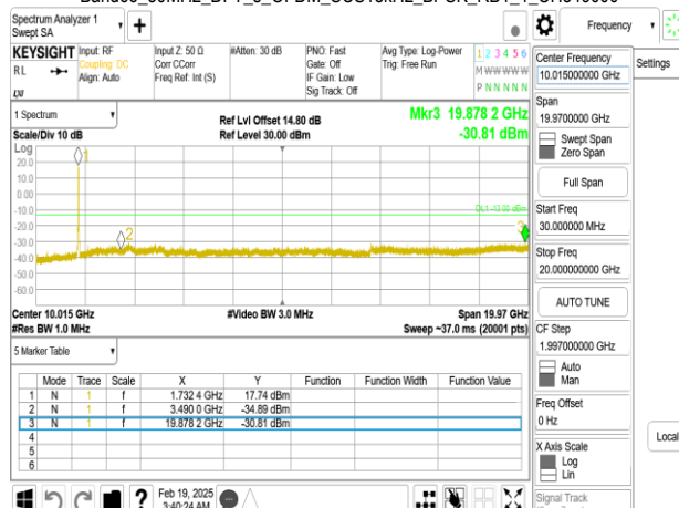
Band66_30MHz_DFT_s_OFDM_SCS15kHz_BPSK_RB1_1_CH349000
