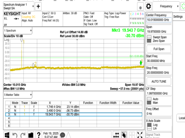
Band66_5MHz_DFT_s_OFDM_SCS15kHz_BPSK_RB1_1_CH349000
