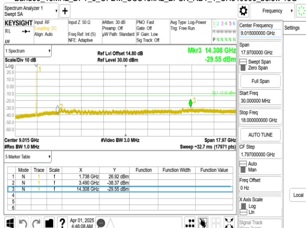
Band66_15MHz_DFT_s_OFDM_SCS15kHz_BPSK_RB1_1_CH345400
