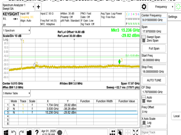
Band66_25MHz_DFT_s_OFDM_SCS30kHz_BPSK_RB1_1_CH353500_below 18G
