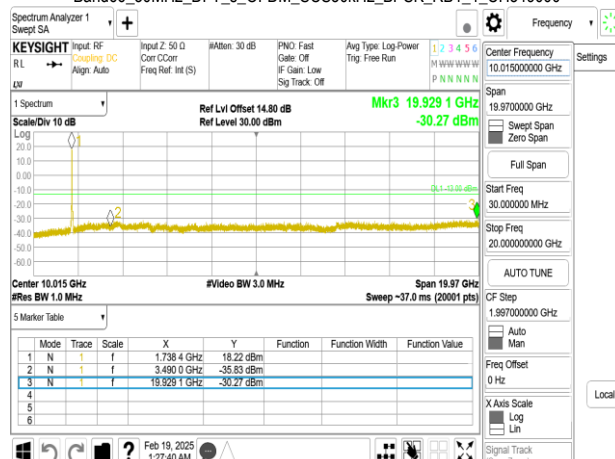
Band66_30MHz_DFT_s_OFDM_SCS30kHz_BPSK_RB1_1_CH349000
