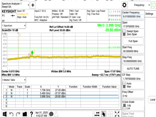
Band66_20MHz_DFT_s_OFDM_SCS15kHz_BPSK_RB1_1_CH354000
