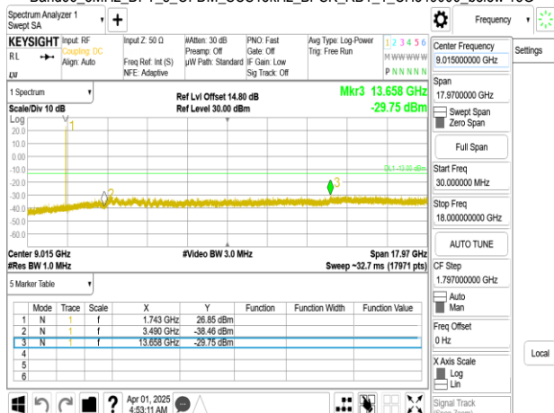
Band66_5MHz_DFT_s_OFDM_SCS15kHz_BPSK_RB1_1_CH355500
