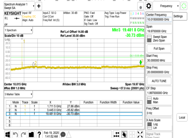
Band66_25MHz_DFT_s_OFDM_SCS30kHz_BPSK_RB1_1_CH344500_below 18G
