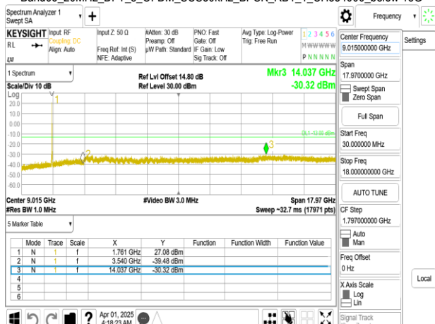
Band66_20MHz_DFT_s_OFDM_SCS30kHz_BPSK_RB1_1_CH354000_below 18G
