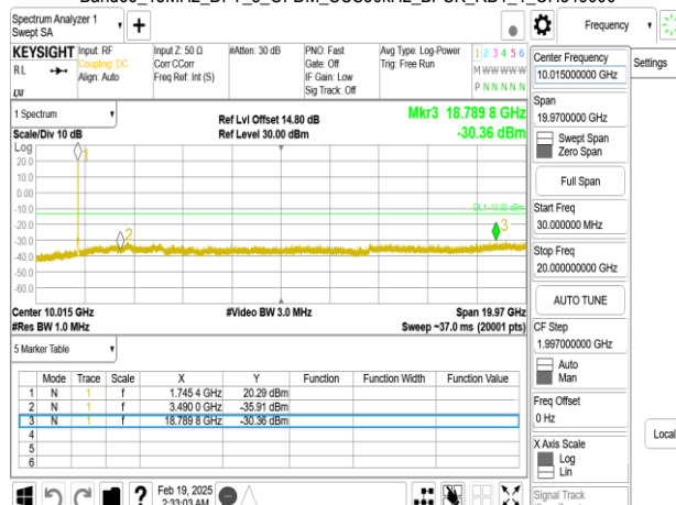
Band66_15MHz_DFT_s_OFDM_SCS30kHz_BPSK_RB1_1_CH349000
