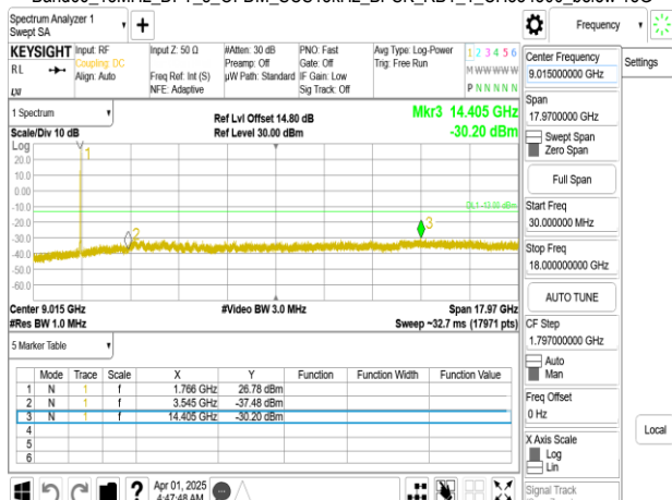
Band66_15MHz_DFT_s_OFDM_SCS15kHz_BPSK_RB1_1_CH345400_below 18G
