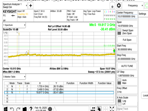
Band66_25MHz_DFT_s_OFDM_SCS15kHz_BPSK_RB1_1_CH349000
