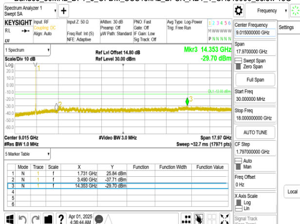
Band66_30MHz_DFT_s_OFDM_SCS15kHz_BPSK_RB1_1_CH353000
