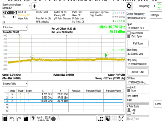
Band66_30MHz_DFT_s_OFDM_SCS15kHz_BPSK_RB1_1_CH353000_below 18G
