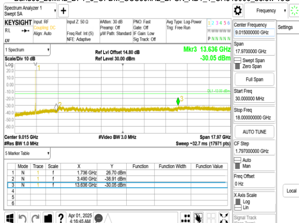
Band66_20MHz_DFT_s_OFDM_SCS30kHz_BPSK_RB1_1_CH354000
