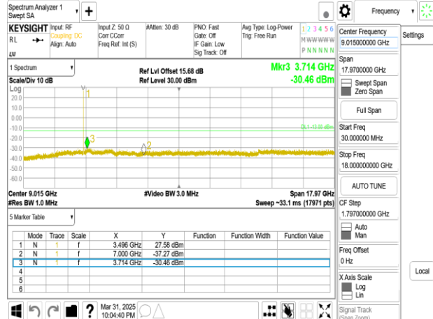
Band77-Part27_10MHz_DFT_s_OFDM_SCS30kHz_BPSK_RB1_1_CH636332_below 18G
