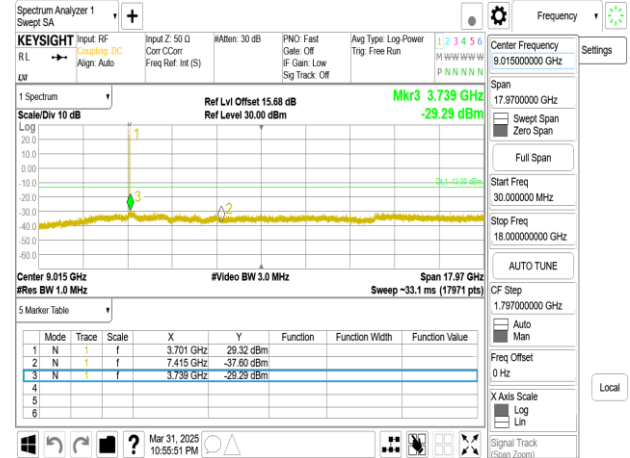
Band77-Part27_15MHz_DFT_s_OFDM_SCS15kHz_BPSK_RB1_1_CH656000_below 18G
