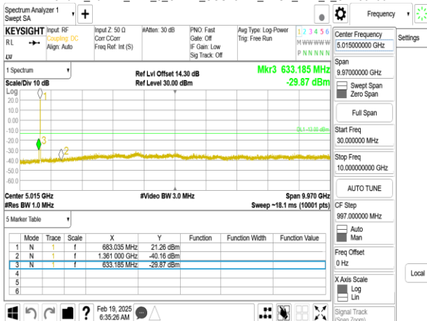
Band71_10MHz_DFT_s_OFDM_SCS15kHz_BPSK_RB1_1.CH136600
