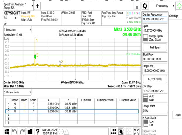
Band77-Part27_10MHz_DFT_s_OFDM_SCS15kHz_BPSK_RB1_1_CH633334_below 18G
