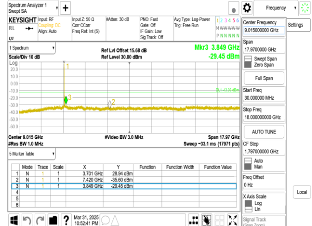
Band77-Part27_20MHz_DFT_s_OFDM_SCS15kHz_BPSK_RB1_1_CH656000_below 18G
