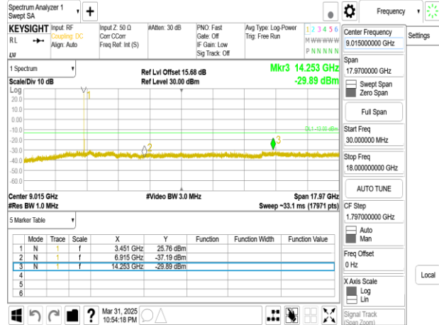
Band77-Part27_15MHz_DFT_s_OFDM_SCS15kHz_BPSK_RB1_1_CH633334_below 18G
