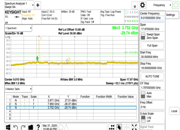
Band77-Part27_10MHz_DFT_s_OFDM_SCS30kHz_BPSK_RB1_1_CH650000_below 18G
