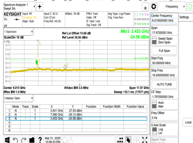
Band77-Part27_10MHz_DFT_s_OFDM_SCS15kHz_BPSK_RB1_1_CH636332_below 18G
