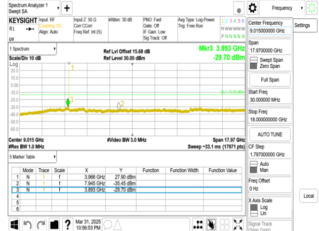
Band77-Part27_15MHz_DFT_s_OFDM_SCS15kHz_BPSK_RB1_1_CH664832_below 18G
