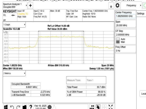
Band25_10MHz_DFT_s_OFDM_SCS30kHz_QPSK_RB24_0_CH376500
