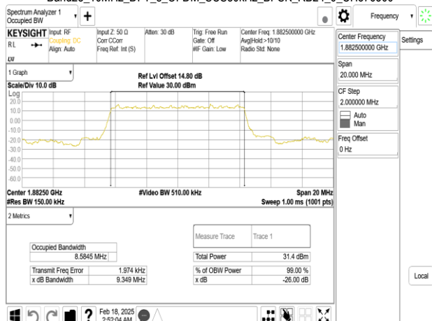
Band25_10MHz_DFT_s_OFDM_SCS30kHz_BPSK_RB24_0_CH376500
