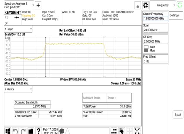
Band25_10MHz_DFT_s_OFDM_SCS15kHz_BPSK_RB50_0_CH376500
