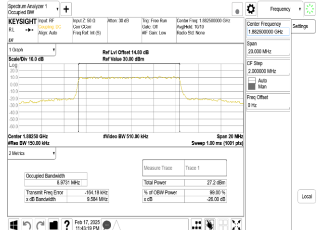
Band25_10MHz_DFT_s_OFDM_SCS15kHz_256QAM_RB50_0_CH376500
