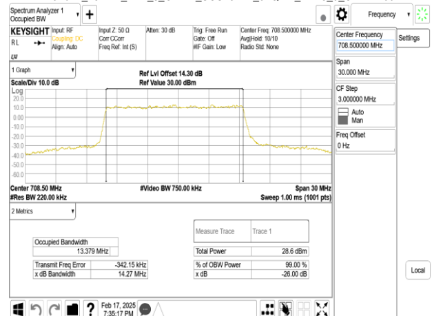
Band12_15MHz_DFT_s_OFDM_SCS15kHz_64QAM_RB75_0_CH141700
