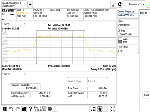
Band5_10MHz_DFT_s_OFDM_SCS15kHz_BPSK_RB50_0_CH168800
