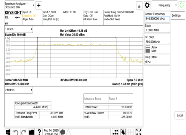
Band5_5MHz_DFT_s_OFDM_SCS15kHz_16QAM_RB25_0_CH169300
