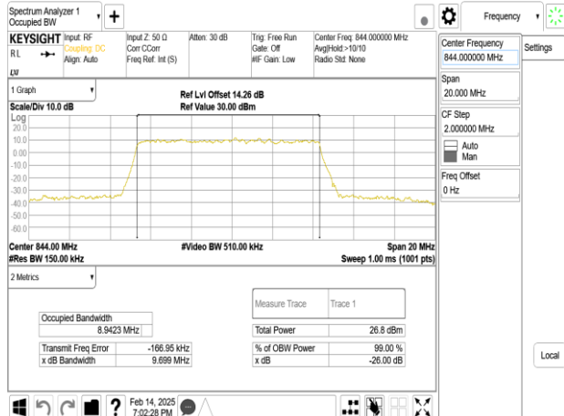
Band5_10MHz_DFT_s_OFDM_SCS15kHz_256QAM_RB50_0_CH168800
