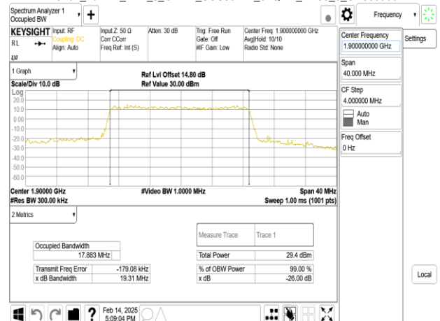
Band2_20MHz_DFT_s_OFDM_SCS30kHz_64QAM_RB50_0_CH380000
