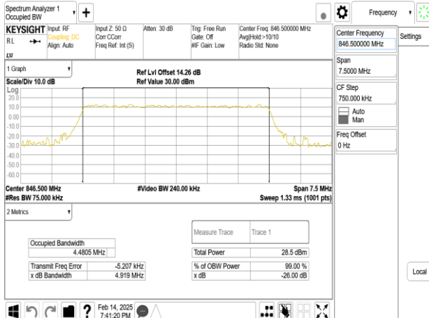
Band5_5MHz_DFT_s_OFDM_SCS15kHz_64QAM_RB25_0_CH169300
