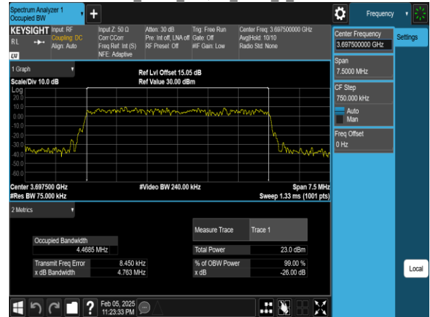
Band48 5MHz 64QAM_RB25_0_CH56715
