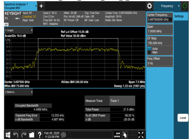
Band48 5MHz 256QAM_RB25_0_CH56715
