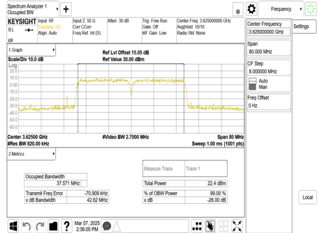
Band48_20MHz+20MHz_256QAM_RB100-0+RB100-0_CH55891+CH56089
