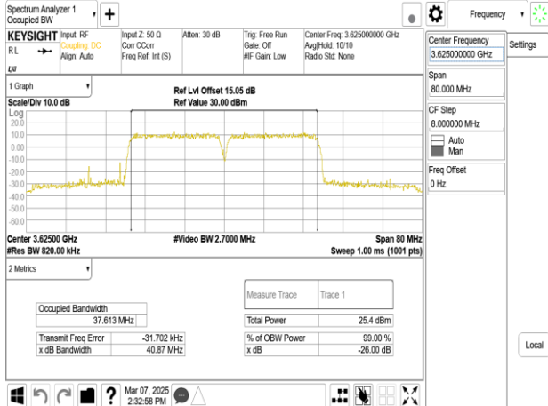
Band48_20MHz+20MHz_64QAM_RB100-0+RB100-0_CH55891+CH56089
