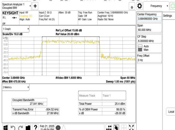
Band48_30MHz_DFT_s_OFDM_SCS30kHz_QPSK_RB75_0_CH645666
