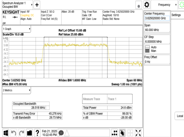
Band48_30MHz_DFT_s_OFDM_SCS15kHz_16QAM_RB160_0_CH645666
