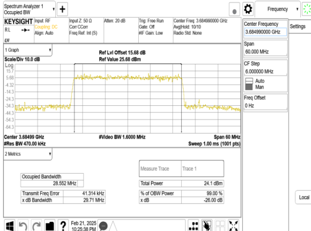
Band48_30MHz_DFT_s_OFDM_SCS15kHz_16QAM_RB160_0_CH645666
