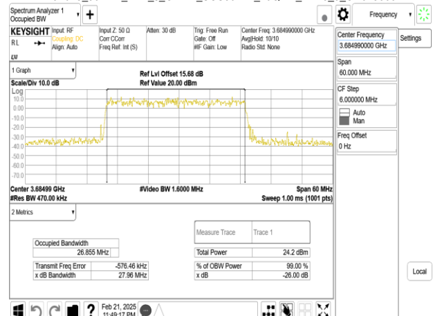
Band48_30MHz_DFT_s_OFDM_SCS30kHz_16QAM_RB75_0_CH645666
