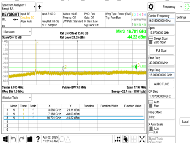
Band48_15MHz+20MHz_QPSK_RB1-74_1-0_CH55318-55489_upper 18G
