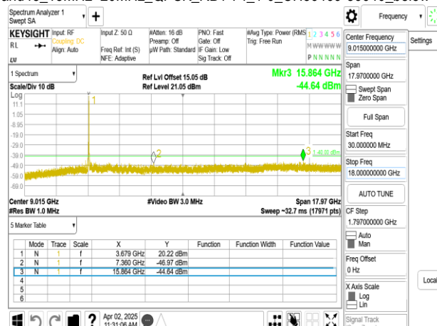
Band48_15MHz+20MHz_QPSK_RB1-74_1-0_CH56469-56640_upper 18G
