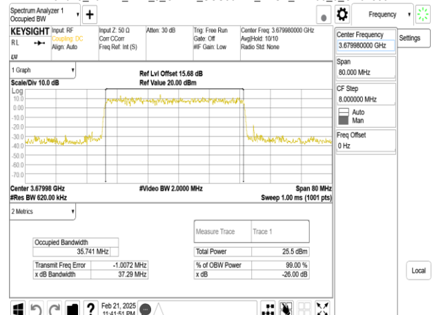
Band48_40MHz_DFT_s_OFDM_SCS30kHz_BPSK_RB100_0_CH645332
