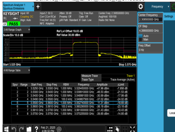
Band48_10MHz_QPSK_RB50_0_CH55290
