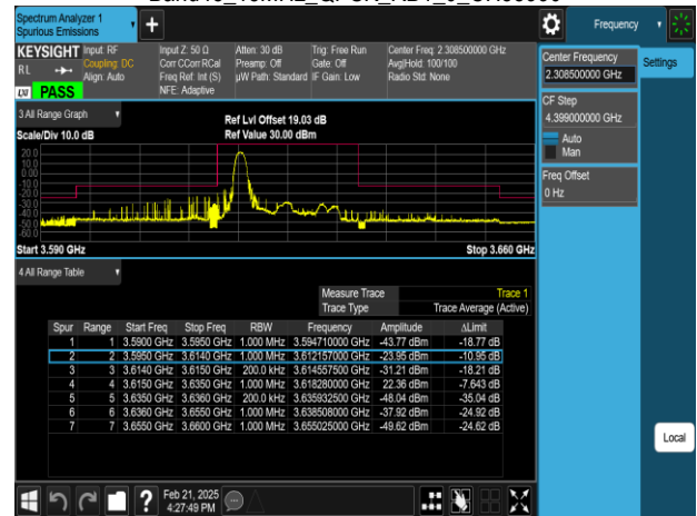
Band48_15MHz_QPSK_RB1_74_CH55990
