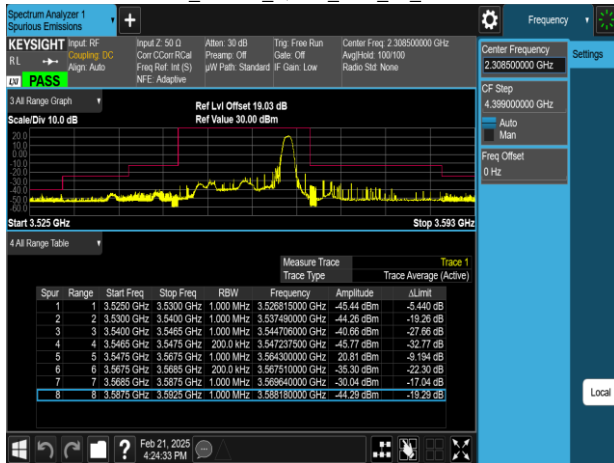
Band48_15MHz_QPSK_RB75_0_CH55315
