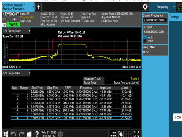
Band48_15MHz_QPSK_RB75_0_CH55315
