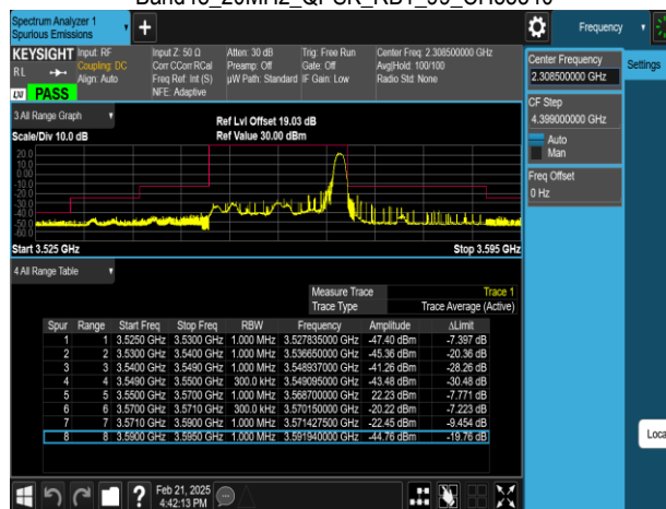
Band48_20MHz_QPSK_RB100_0_CH55340
