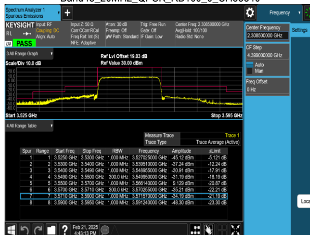
Band48_20MHz_QPSK_RB100_0_CH55340
