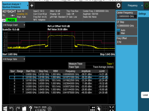
Band48_10MHz_QPSK_RB50_0_CH55990
