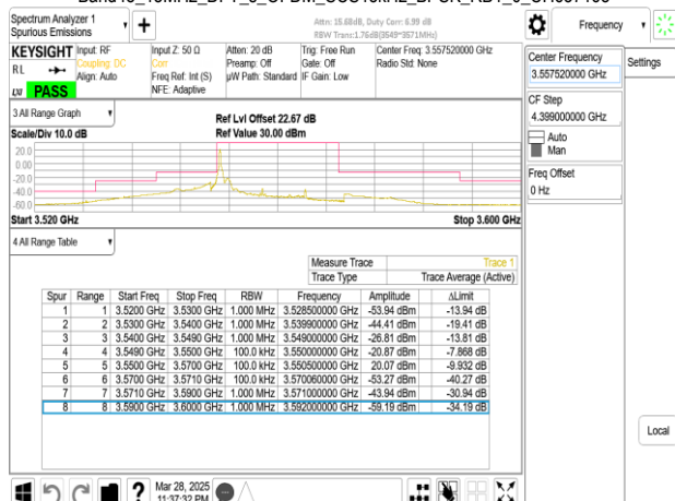
Band48_15MHz_DFT_s_OFDM_SCS15kHz_BPSK_RB1_0_CH637168
