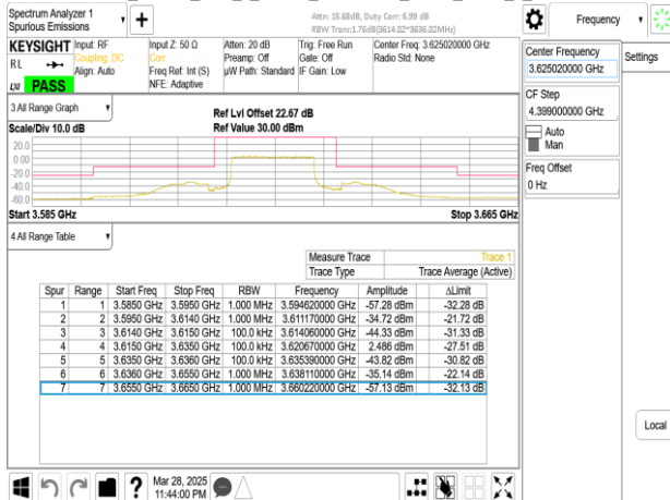
Band48_15MHz_DFT_s_OFDM_SCS15kHz_BPSK_RB1_0_CH641666
