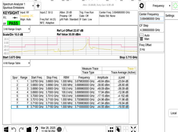
Band48_10MHz_DFT_s_OFDM_SCS15kHz_BPSK_RB50_0_CH646332
