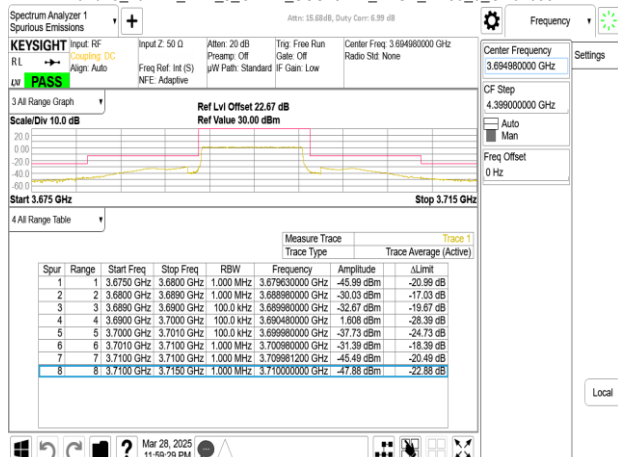
Band48_10MHz_DFT_s_OFDM_SCS15kHz_BPSK_RB50_0_CH646332
