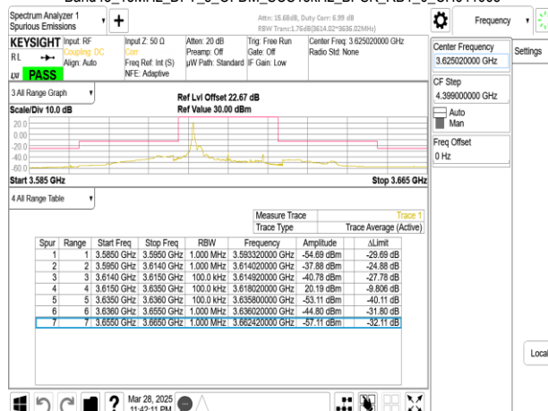
Band48_15MHz_DFT_s_OFDM_SCS15kHz_BPSK_RB1_0_CH641668
