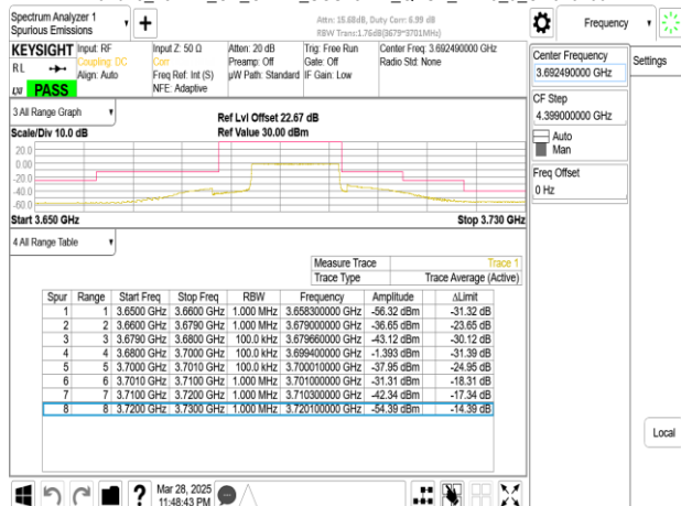
Band48_15MHz_CP_OFDM_SCS15kHz_QPSK_RB79_0_CH646166
