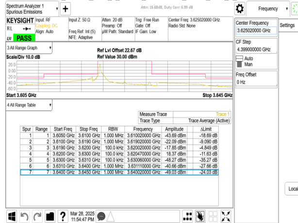
Band48_10MHz_DFT_s_OFDM_SCS15kHz_BPSK_RB1_51_CH641668
