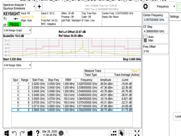
Band48_15MHz_DFT_s_OFDM_SCS15kHz_BPSK_RB75_0_CH637168
