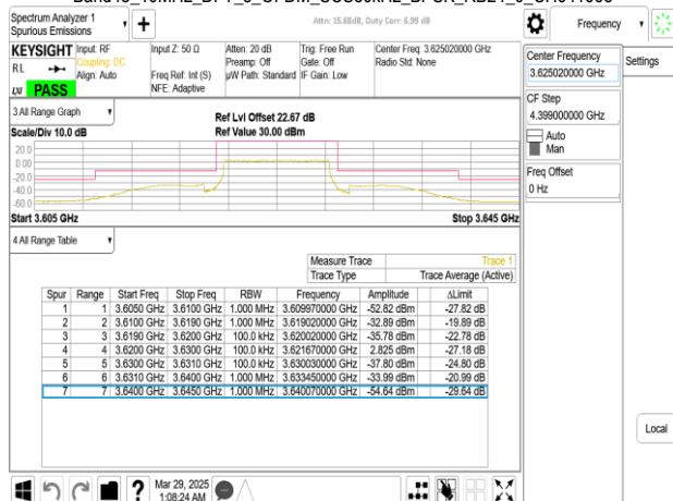
Band48_10MHz_DFT_s_OFDM_SCS30kHz_BPSK_RB1_0_CH646332
