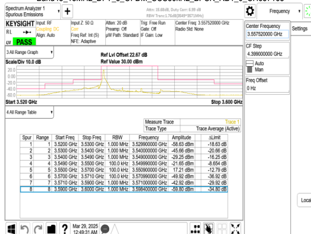
Band48_15MHz_DFT_s_OFDM_SCS30kHz_BPSK_RB1_37_CH637168
