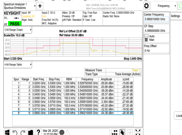
Band48_20MHz_DFT_s_OFDM_SCS15kHz_BPSK_RB1_0_CH637334
