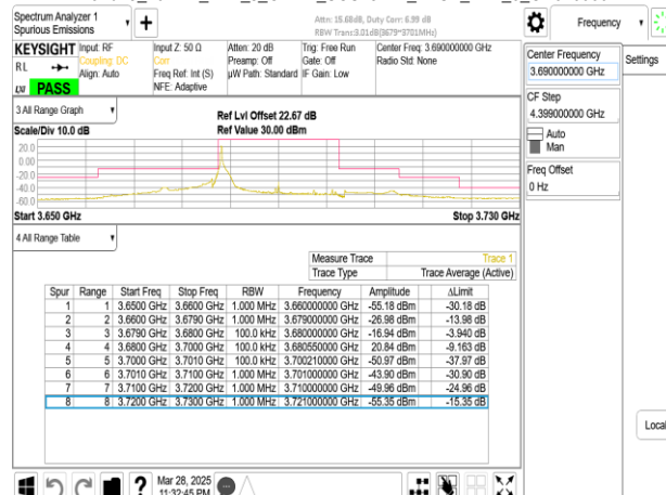
Band48_20MHz_DFT_s_OFDM_SCS15kHz_BPSK_RB1_0_CH646000
