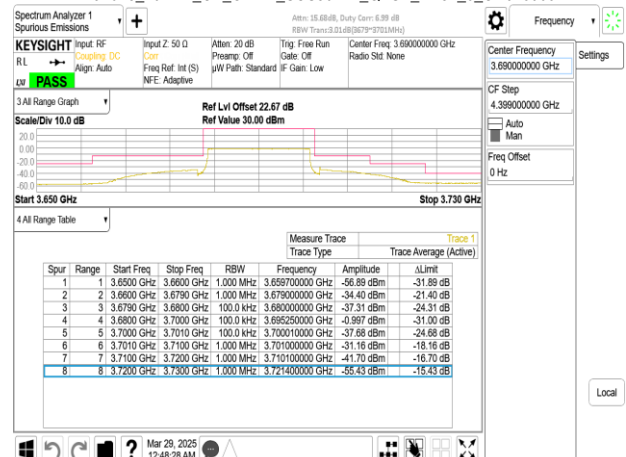
Band48_20MHz_CP_OFDM_SCS30kHz_QPSK_RB51_0_CH646000
