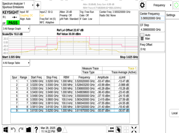
Band48_30MHz_DFT_s_OFDM_SCS15kHz_BPSK_RB1_0_CH637668
