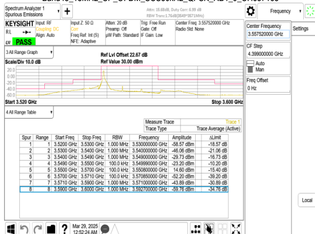
Band48_15MHz_CP_OFDM_SCS30kHz_QPSK_RB38_0_CH637168
