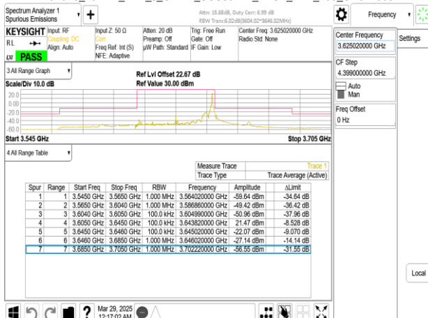
Band48_40MHz_DFT_s_OFDM_SCS30kHz_BPSK_RB1_105_CH641668
