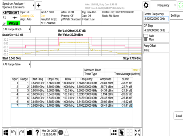
Band48_40MHz_DFT_s_OFDM_SCS30kHz_BPSK_RB1_0_CH641668
