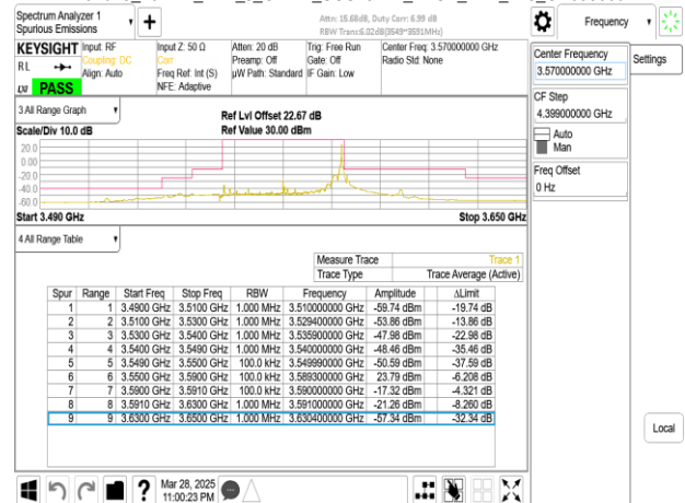
Band48_40MHz_DFT_s_OFDM_SCS15kHz_BPSK_RB216_0_CH638000
