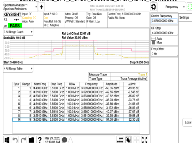
Band48_40MHz_DFT_s_OFDM_SCS30kHz_BPSK_RB1_0_CH638000
