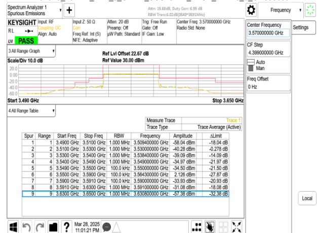
Band48_40MHz_DFT_s_OFDM_SCS15kHz_BPSK_RB1_0_CH641668
