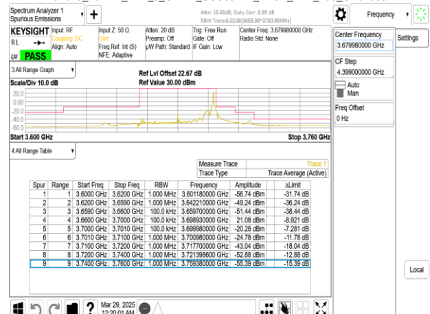
Band48_40MHz_DFT_s_OFDM_SCS30kHz_BPSK_RB1_105_CH645332
