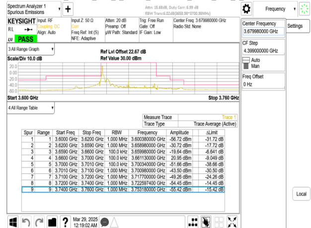
Band48_40MHz_DFT_s_OFDM_SCS30kHz_BPSK_RB1_105_CH645332
