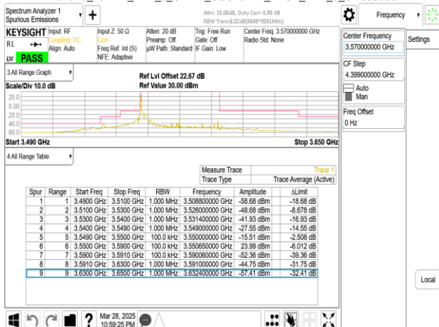
Band48_40MHz_DFT_s_OFDM_SCS15kHz_BPSK_RB1_0_CH638000
