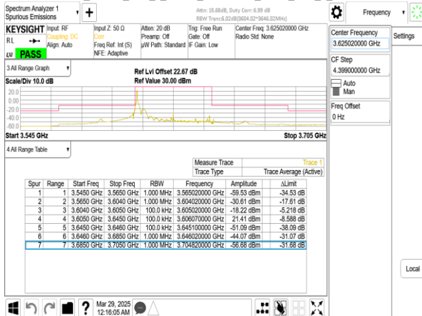
Band48_40MHz_DFT_s_OFDM_SCS30kHz_BPSK_RB1_105_CH641668
