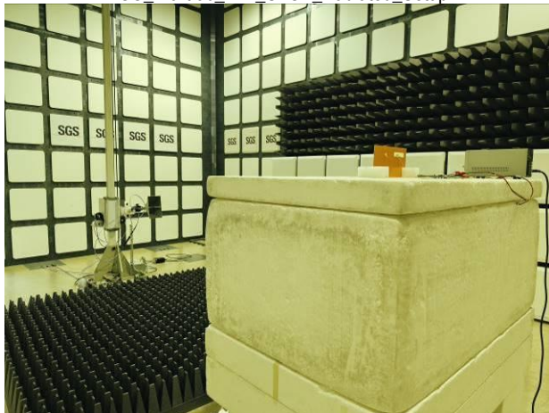
FCC_Part 96 LTE_ULCA_Radiated_Setup
