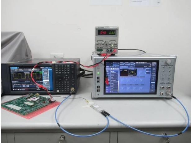
FCC_Part 96_NR_Conducted_Setup
