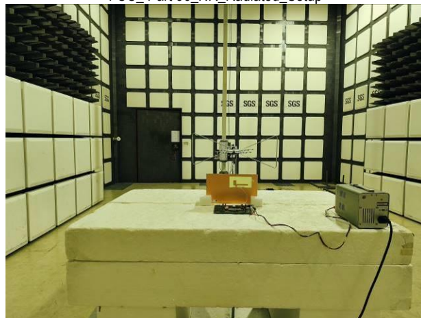
FCC_Part 96 NR_Radiated_Setup
