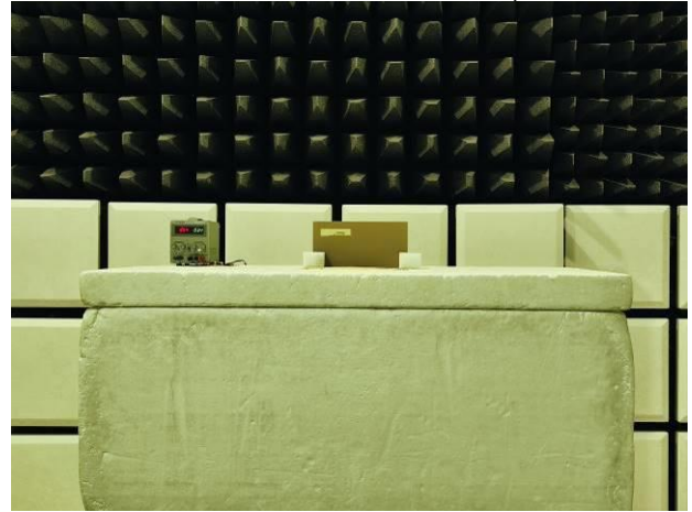
FCC_Part 96_LTE_Radiated_Setup
