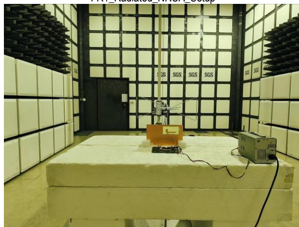
FR1_Radiated_NRCA_Setup
