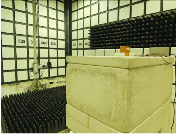
LTE_Radiated_Setup
