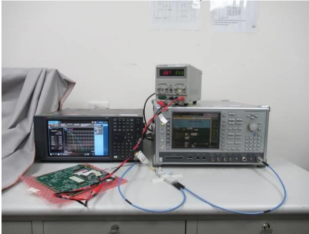
FR1_Conducted_Setup
