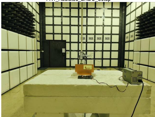
FR1_Radiated_ENDC_Setup
