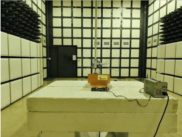
FR1_Radiated_SA_Setup
