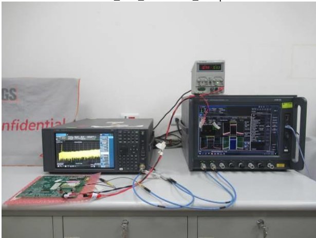
FR1_2TX_Conducted_Setup
