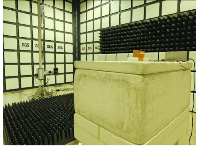
LTE_ULCA_Radiated_Setup
