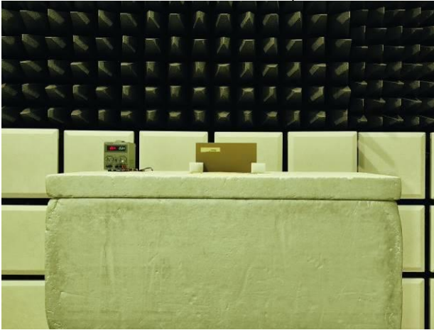
FR1_Radiated_SA_Setup
