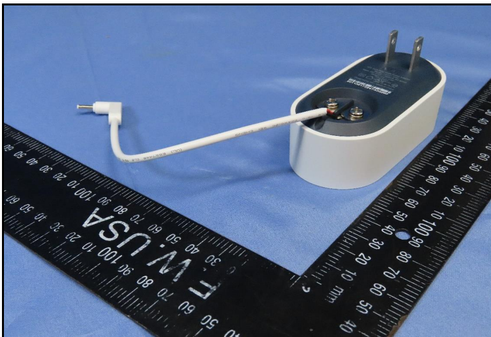
Adapter (Brand: ADT, Model: 1A102-1215)
