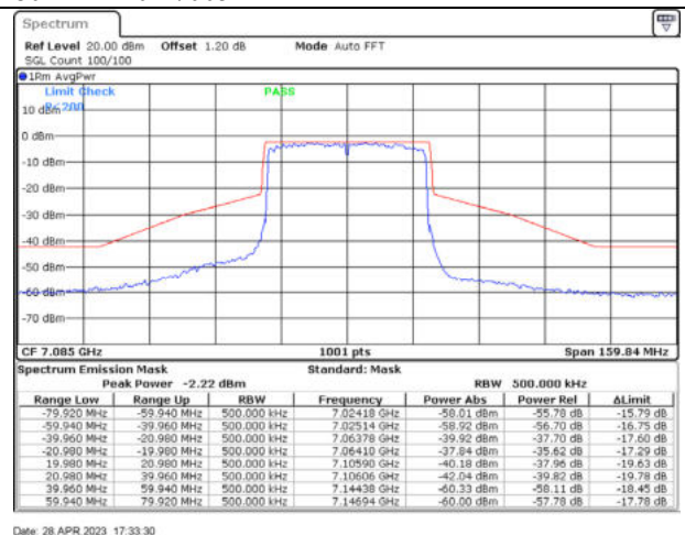
802.11ax40 / 7085MHz / Chain B - CDD
