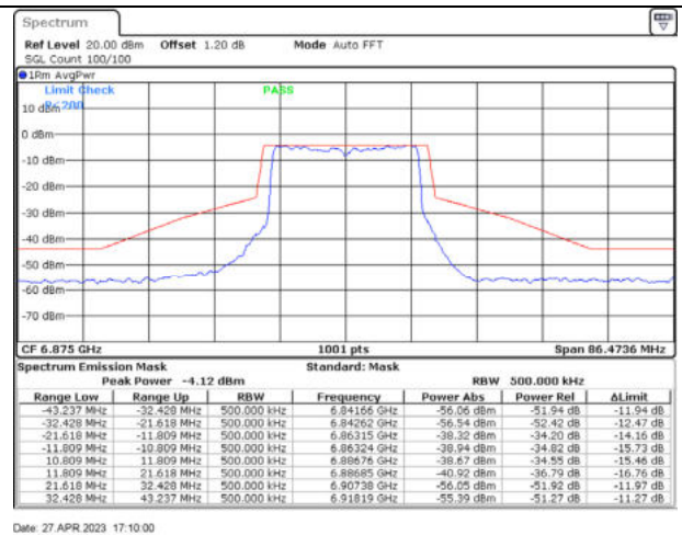
802.11ax20 / 6875MHz / Chain B - CDD
