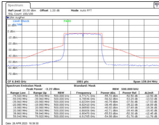
802.11ax40 / 6845MHz / Chain A - CDD
