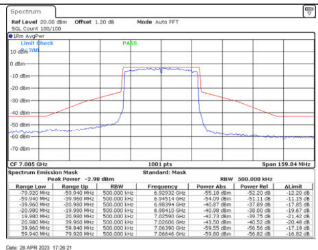
802.11ax40 / 7005MHz / Chain B - CDD
