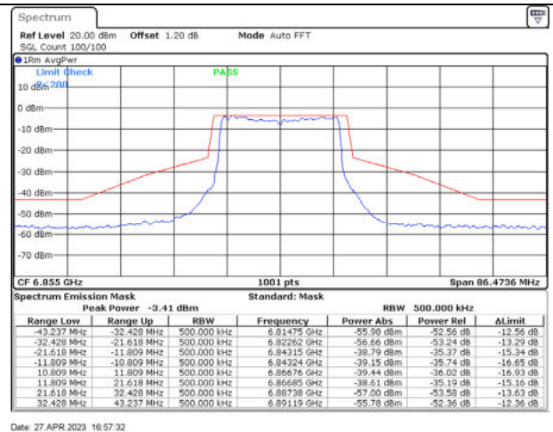
802.11ax20 / 6855MHz / Chain D - CDD
