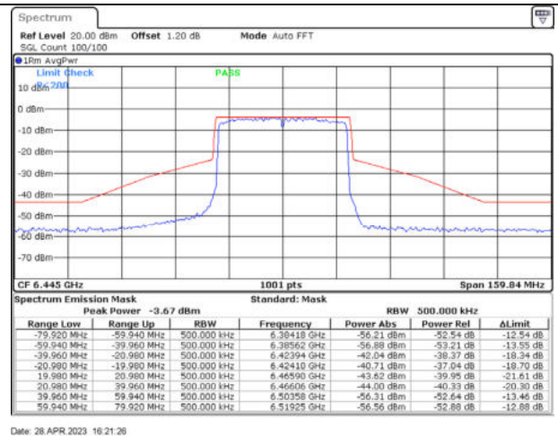
802.11ax40 / 6445MHz / Chain B - CDD
