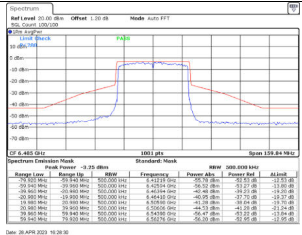
802.11ax40 / 6485MHz / Chain D - CDD
