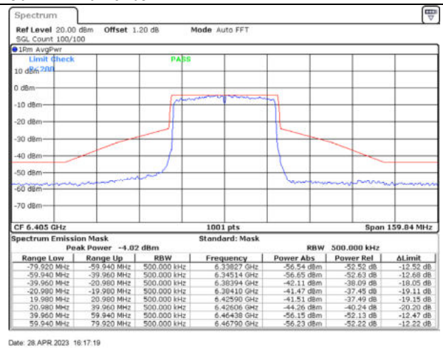
802.11ax40 / 6405MHz / Chain D - CDD
