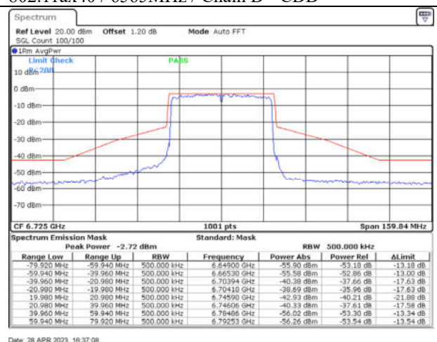
802.11ax40 / 6725MHz / Chain B - CDD
