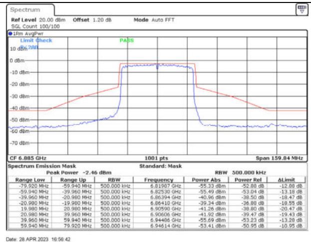
802.11ax40 / 6885MHz / Chain B - CDD
