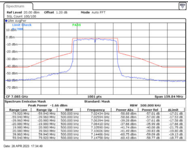
802.11ax40 / 7085MHz / Chain D - CDD
