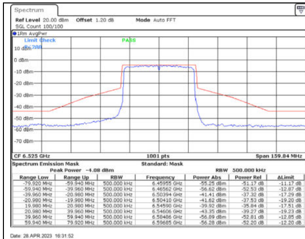
802.11ax40 / 6525MHz / Chain A - CDD
