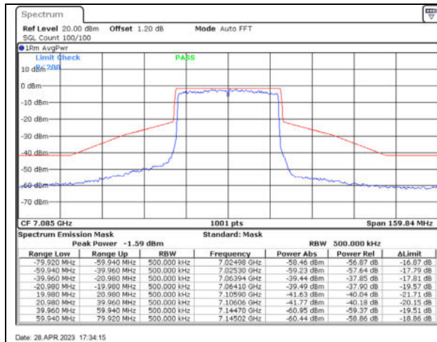
802.11ax40 / 7085MHz / Chain C - CDD
