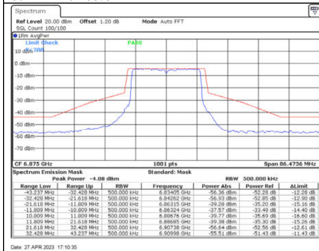
802.11ax20 / 6875MHz / Chain C - CDD
