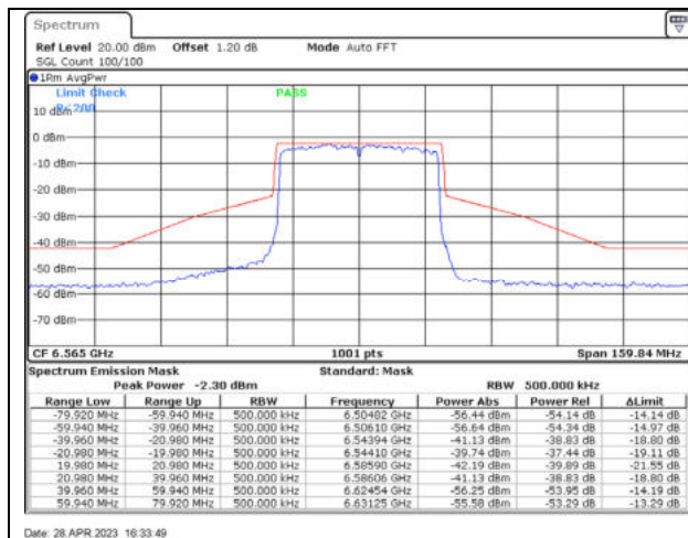
802.11ax40 / 6565MHz / Chain C - CDD
