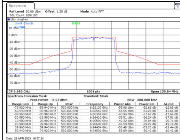
802.11ax40 / 6885MHz / Chain A - CDD
