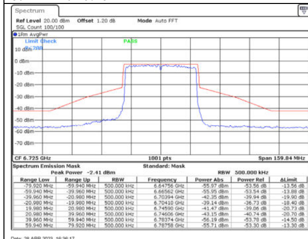
802.11ax40 / 6725MHz / Chain C - CDD
