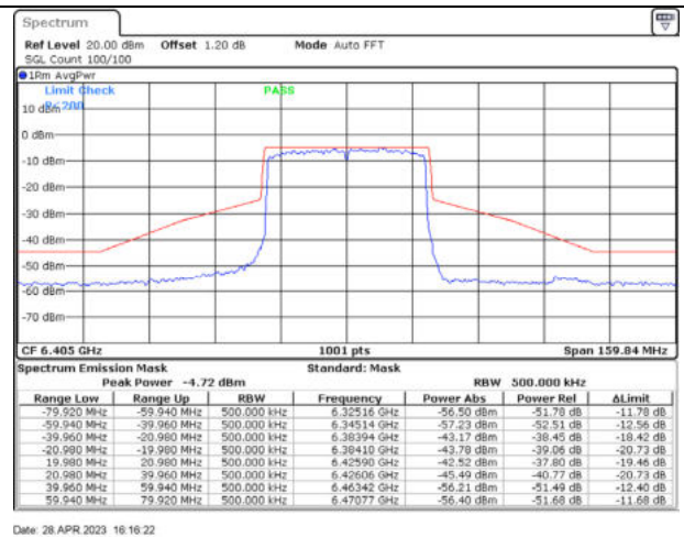
802.11ax40 / 6405MHz / Chain B - CDD
