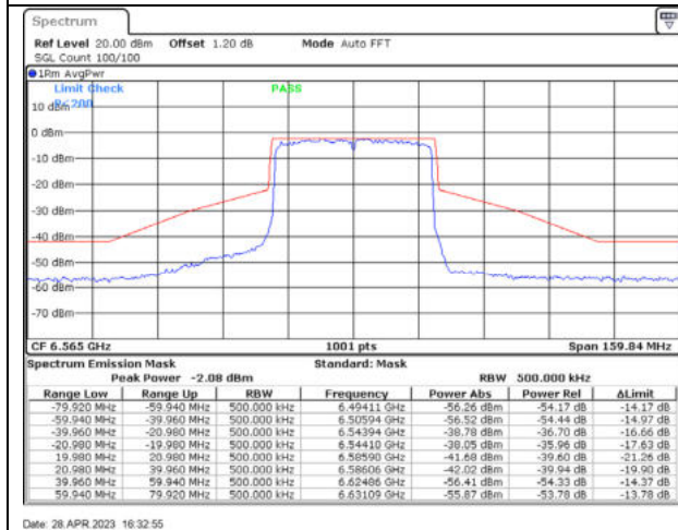
802.11ax40 / 6565MHz / Chain A - CDD
