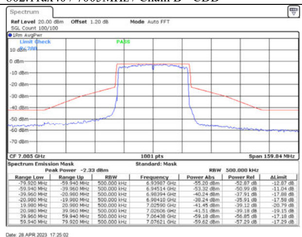
802.11ax40 / 7005MHz / Chain D - CDD
