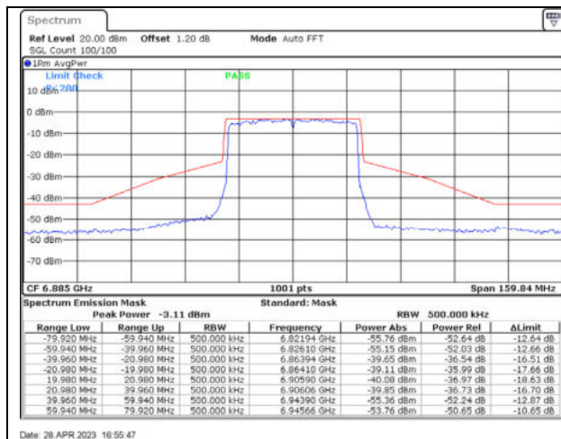
802.11ax40 / 6885MHz / Chain C - CDD
