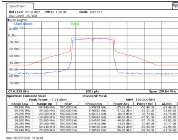
802.11ax40 / 6525MHz / Chain C - CDD
