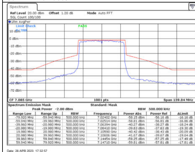
802.11ax40 / 7085MHz / Chain A - CDD
