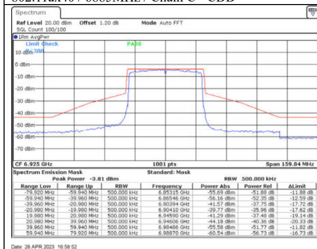
802.11ax40 / 6925MHz / Chain A - CDD
