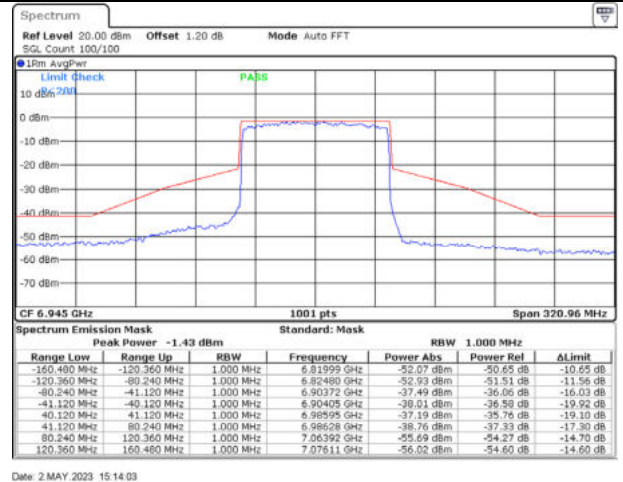
802.11ax80 / 6945MHz / Chain D - CDD
