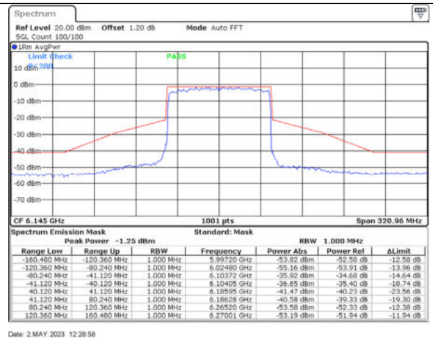
802.11ax80 / 6145MHz / Chain D - CDD
