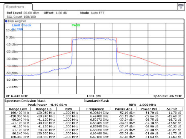
802.11ax80 / 6545MHz / Chain B - CDD
