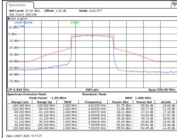
802.11ax80 / 6945MHz / Chain A - CDD
