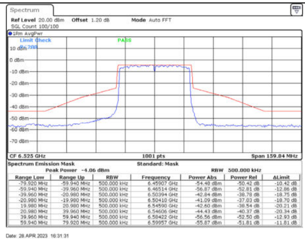
802.11ax40 / 6525MHz / Chain B - CDD
