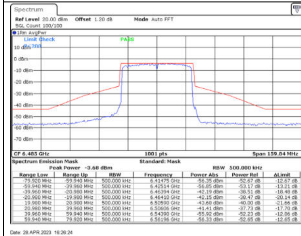
802.11ax40 / 6485MHz / Chain A - CDD
