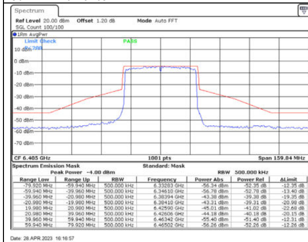
802.11ax40 / 6405MHz / Chain C - CDD
