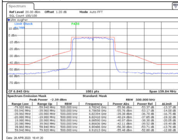
802.11ax40 / 6845MHz / Chain C - CDD
