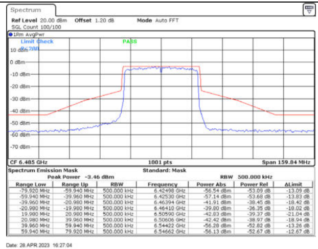
802.11ax40 / 6485MHz / Chain B - CDD
