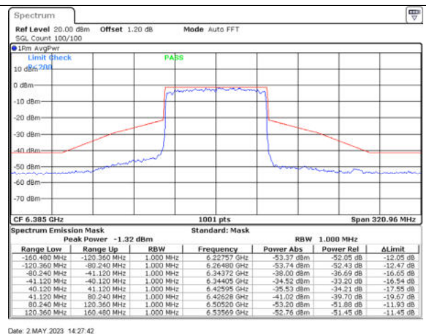
802.11ax80 / 6385MHz / Chain D - CDD
