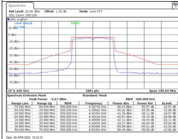
802.11ax40 / 6445MHz / Chain A - CDD
