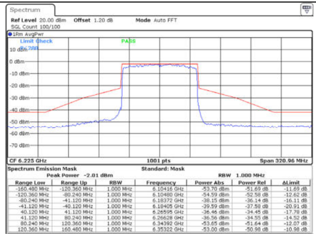
802.11ax80 / 6225MHz / Chain B - CDD
