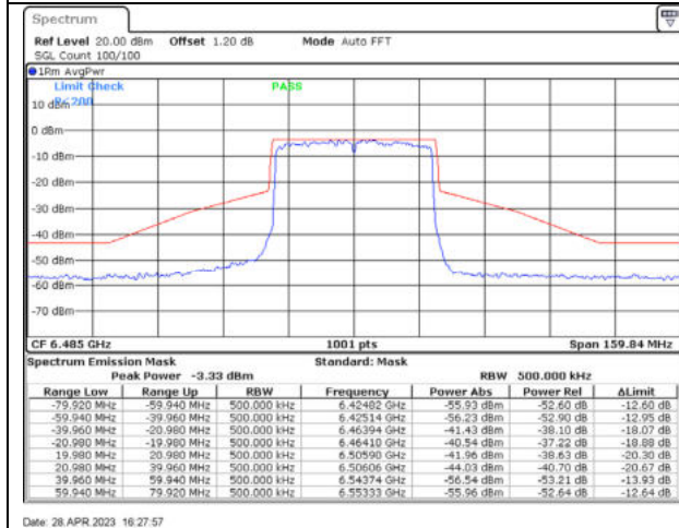
802.11ax40 / 6485MHz / Chain C - CDD
