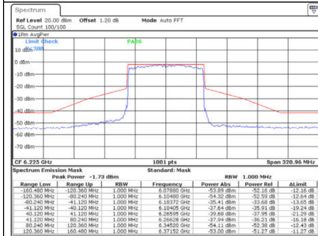
802.11ax80 / 6225MHz / Chain A - CDD
