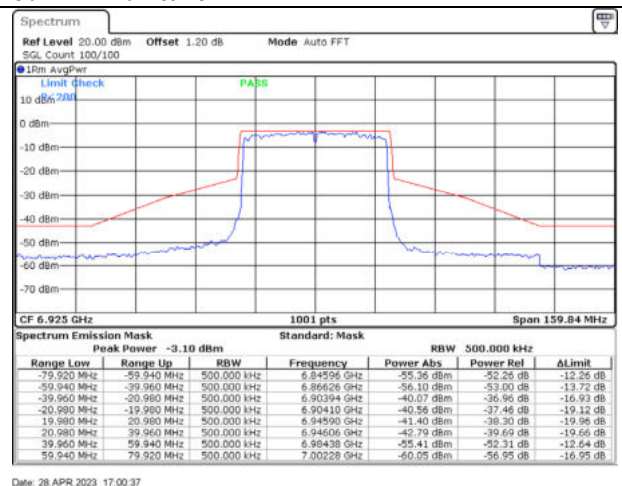
802.11ax40 / 6925MHz / Chain D - CDD
