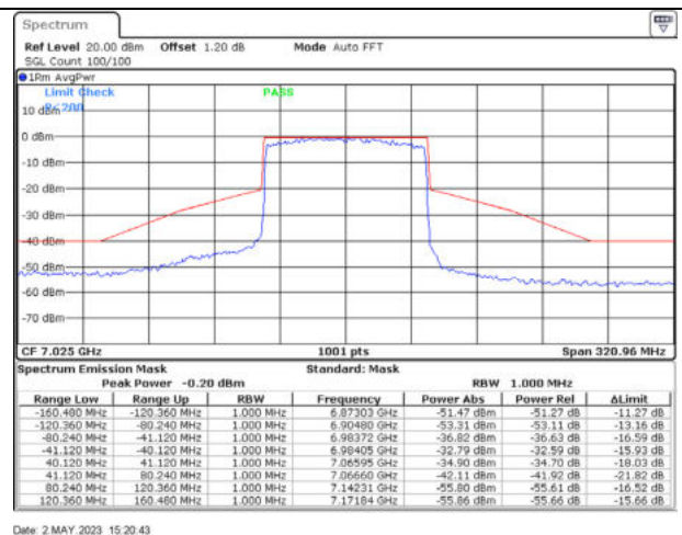
802.11ax80 / 7025MHz / Chain B - CDD
