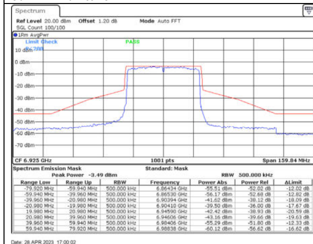
802.11ax40 / 6925MHz / Chain C - CDD
