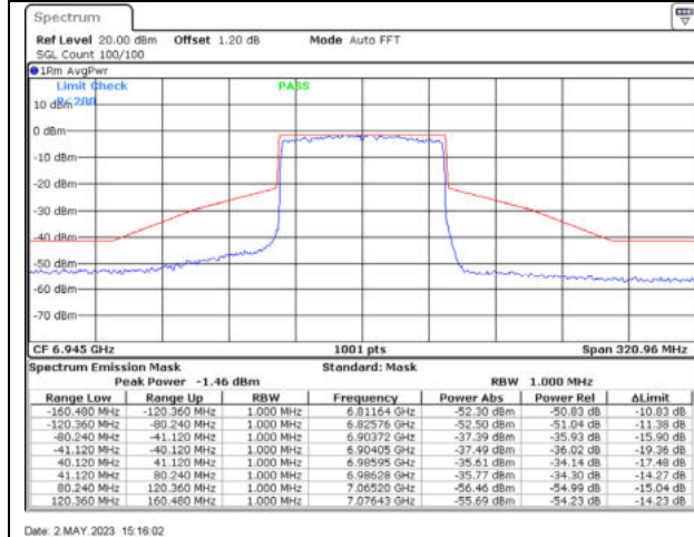
802.11ax80 / 6945MHz / Chain C - CDD
