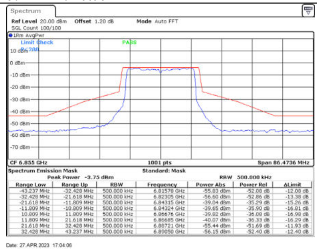
802.11ax20 / 6855MHz / Chain B - CDD
