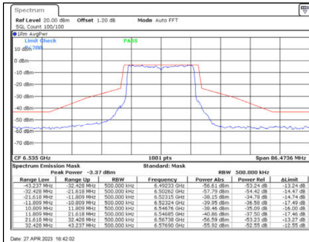
802.11ax20 / 6535MHz / Chain A - CDD
