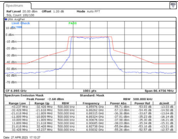
802.11ax20 / 6895MHz / Chain B - CDD
