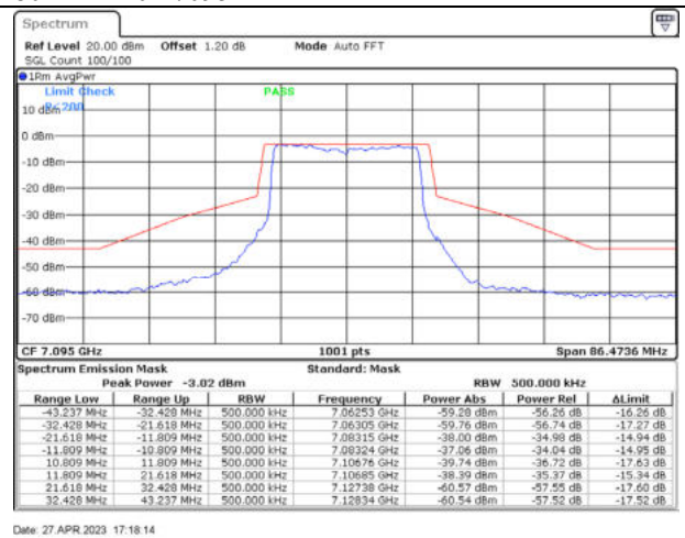
802.11ax20 / 7095MHz / Chain D - CDD
