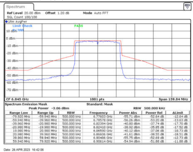
802.11ax40 / 6845MHz / Chain D - CDD
