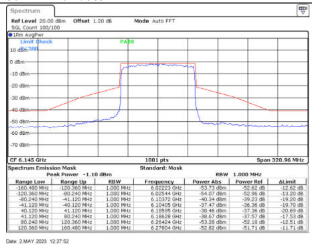
802.11ax80 / 6145MHz / Chain B - CDD
