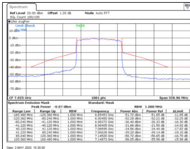
802.11ax80 / 7025MHz / Chain A - CDD
