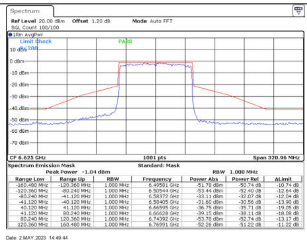
802.11ax80 / 6625MHz / Chain D - CDD
