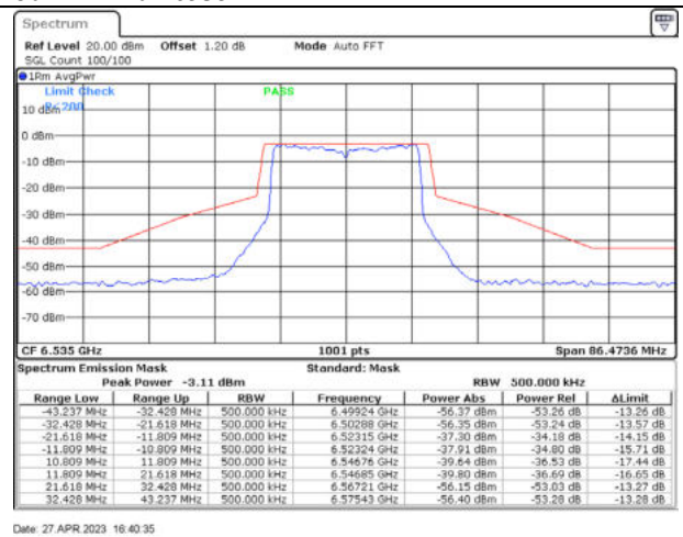
802.11ax20 / 6535MHz / Chain D - CDD
