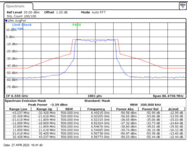
802.11ax20 / 6535MHz / Chain B - CDD
