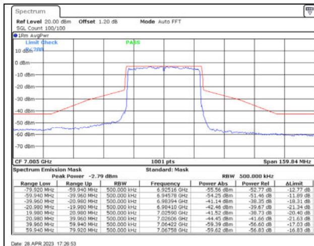
802.11ax40 / 7005MHz / Chain A - CDD
