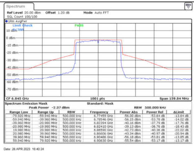
802.11ax40 / 6845MHz / Chain B - CDD
