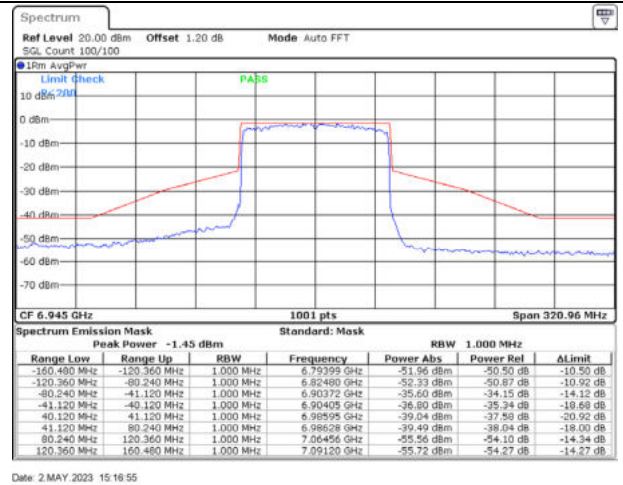
802.11ax80 / 6945MHz / Chain B - CDD
