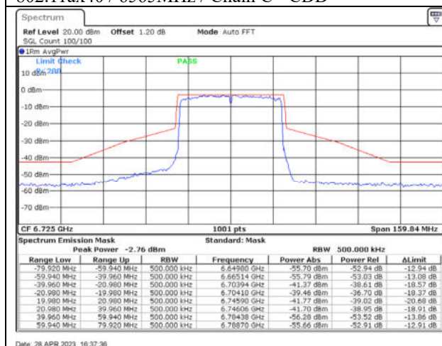
802.11ax40 / 6725MHz / Chain A - CDD
