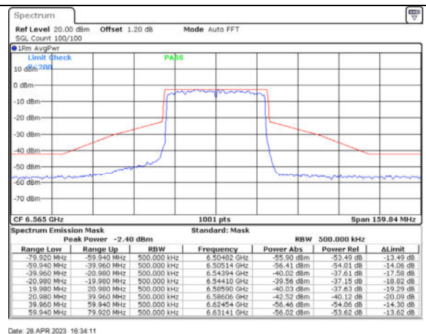
802.11ax40 / 6565MHz / Chain D - CDD
