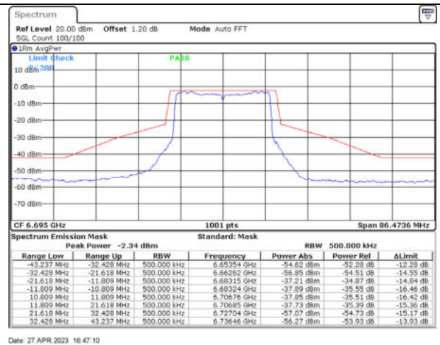
802.11ax20 / 6695MHz / Chain D - CDD
