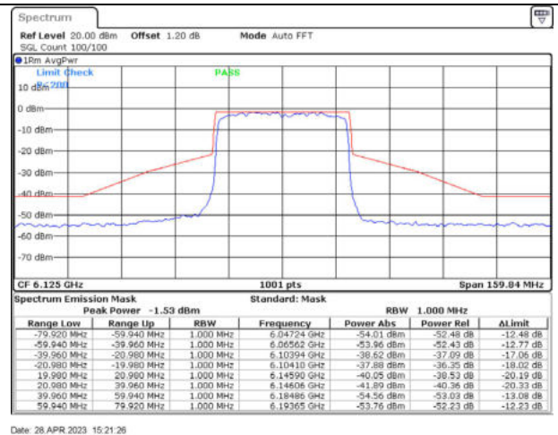
802.11ax40 / 6125MHz / Chain B - CDD
