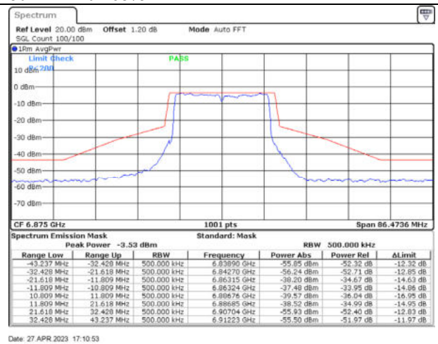
802.11ax20 / 6875MHz / Chain D - CDD
