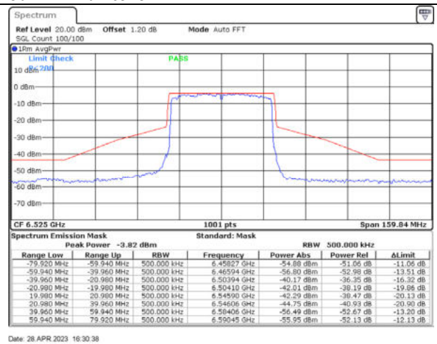
802.11ax40 / 6525MHz / Chain D - CDD
