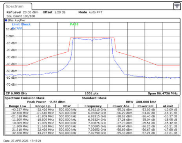
802.11ax20 / 6995MHz / Chain B - CDD
