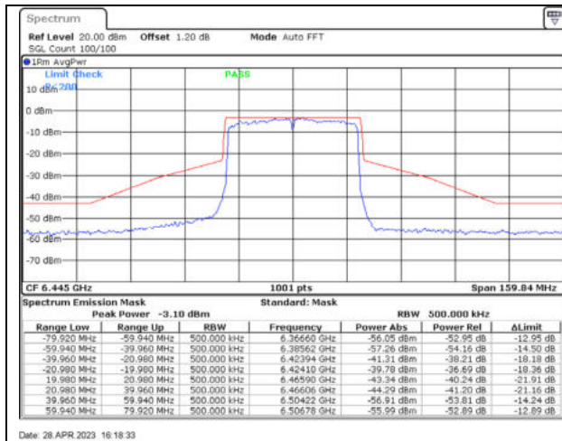
802.11ax40 / 6445MHz / Chain C - CDD
