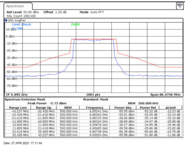
802.11ax20 / 6895MHz / Chain D - CDD
