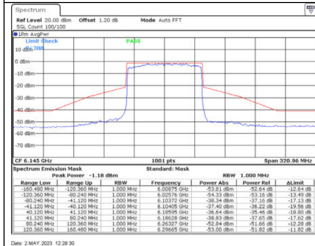
802.11ax80 / 6145MHz / Chain C - CDD
