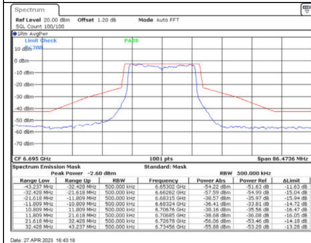
802.11ax20 / 6695MHz / Chain A - CDD
