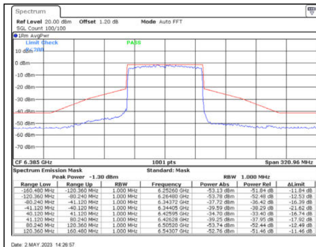
802.11ax80 / 6385MHz / Chain C - CDD
