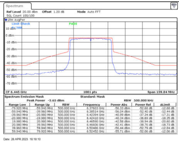
802.11ax40 / 6445MHz / Chain D - CDD
