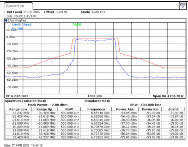
802.11ax20 / 6695MHz / Chain B - CDD
