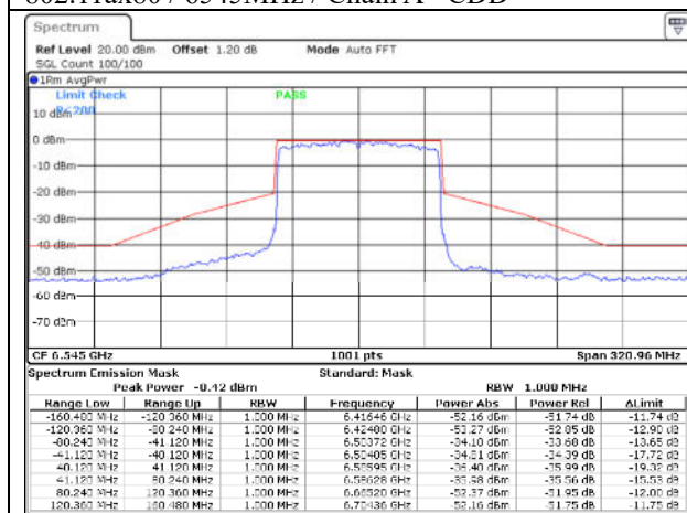
802.11ax80 / 6545MHz / Chain A - CDD
