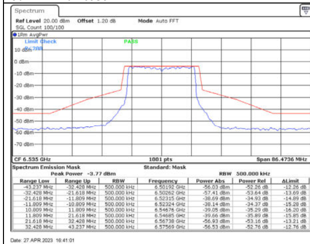
802.11ax20 / 6535MHz / Chain C - CDD
