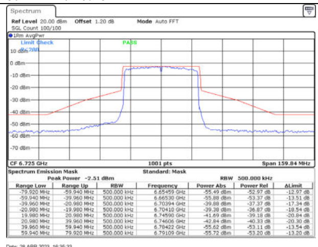
802.11ax40 / 6725MHz / Chain D - CDD
