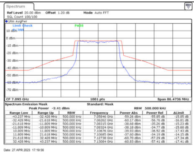
802.11ax20 / 7095MHz / Chain B - CDD
