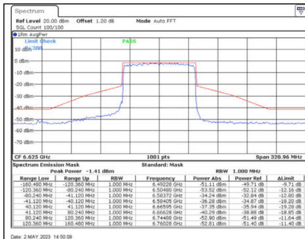
802.11ax80 / 6625MHz / Chain C - CDD
