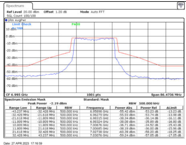
802.11ax20 / 6995MHz / Chain D - CDD
