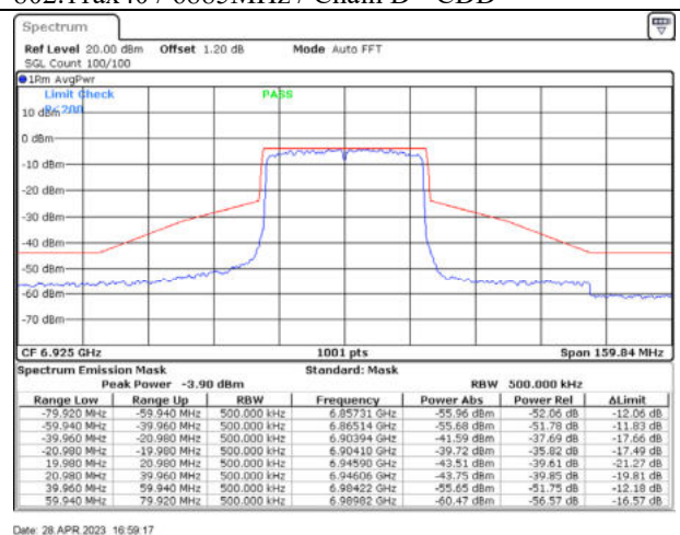
802.11ax40 / 6925MHz / Chain B - CDD
