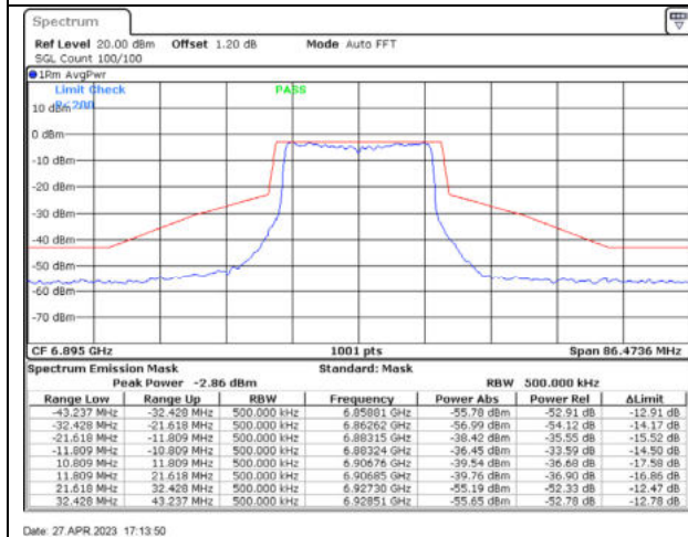
802.11ax20 / 6895MHz / Chain A - CDD
