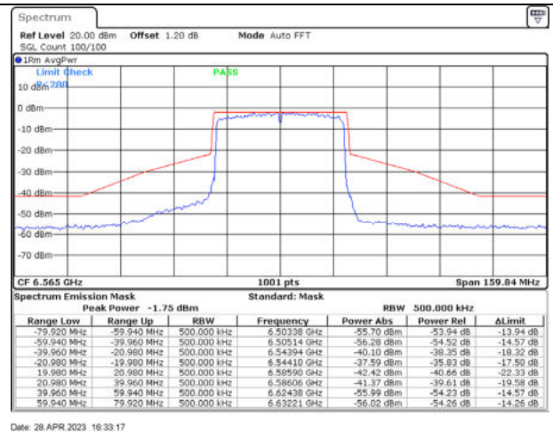
802.11ax40 / 6565MHz / Chain B - CDD
