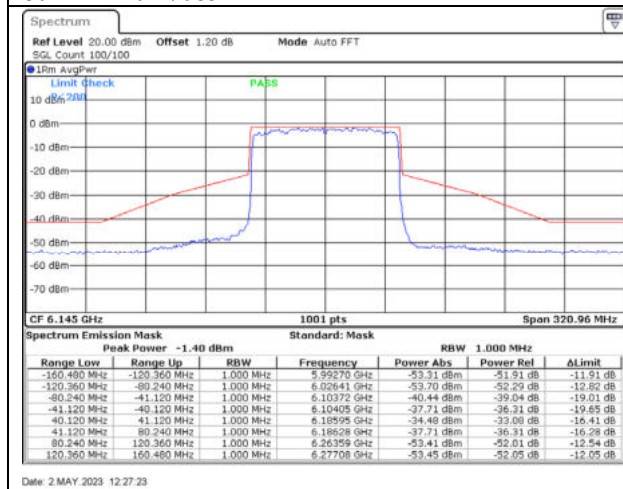
802.11ax80 / 6145MHz / Chain A - CDD
