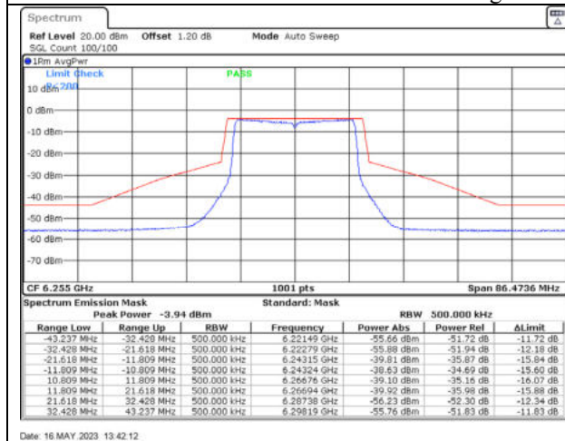
802.11ax20 / 6255MHz / Chain C - Beamforming
