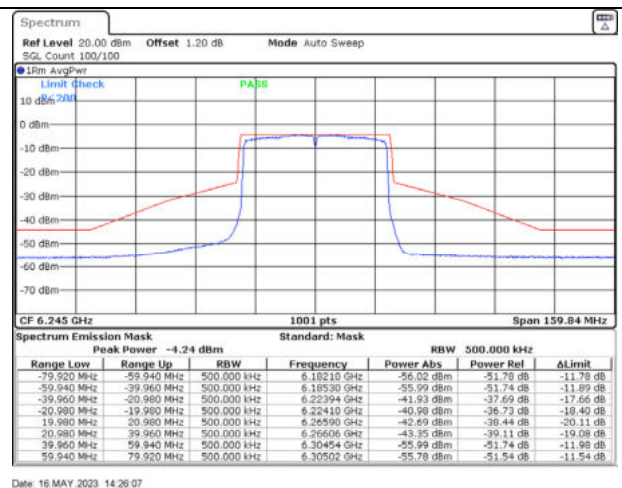
802.11ax40 / 6245MHz / Chain B - Beamforming
