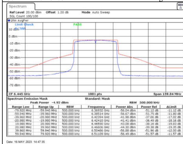
802.11ax40 / 6445MHz / Chain A - Beamforming
