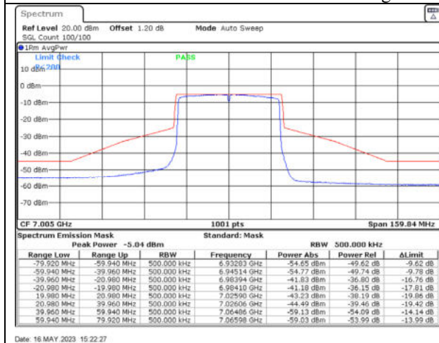
802.11ax40 / 7005MHz / Chain A - Beamforming
