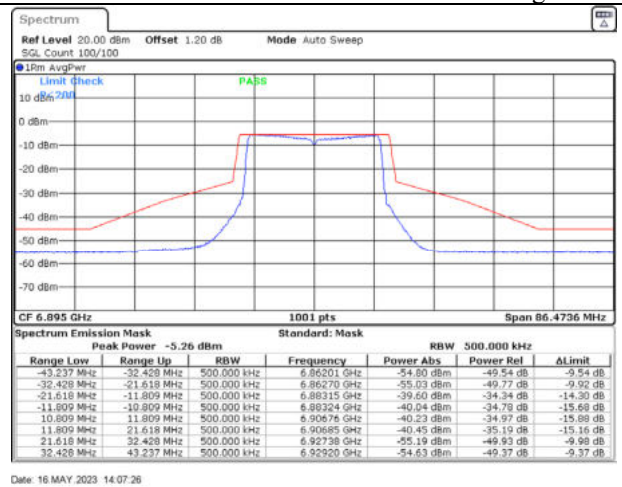
802.11ax20 / 6895MHz / Chain B - Beamforming
