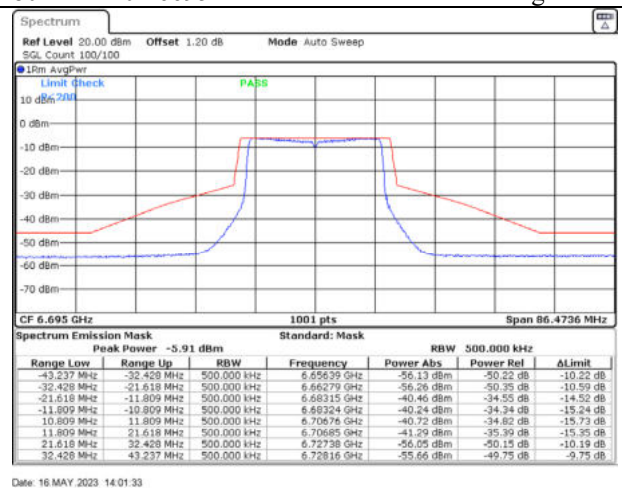
802.11ax20 / 6695MHz / Chain D - Beamforming
