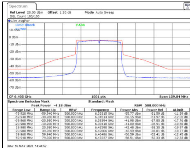
802.11ax40 / 6405MHz / Chain C - Beamforming
