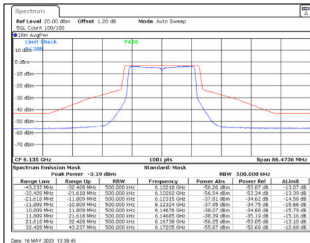
802.11ax20 / 6135MHz / Chain C - Beamforming
