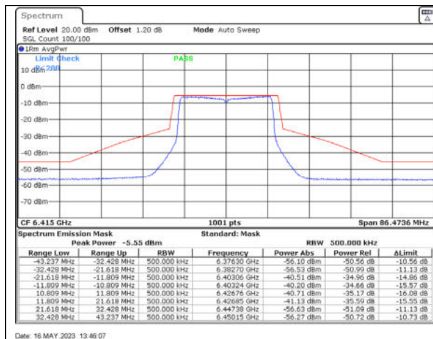
802.11ax20 / 6415MHz / Chain A - Beamforming
