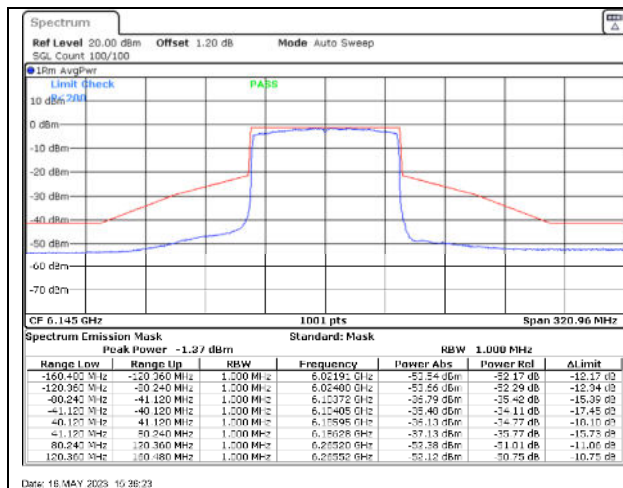
802.11ax80 / 6145MHz / Chain A - Beamforming
