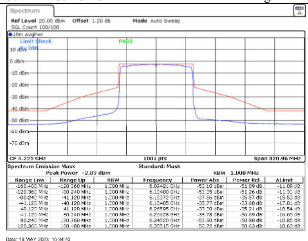
802.11ax80 / 6225MHz / Chain B - Beamforming
