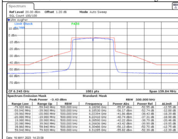
802.11ax40 / 6245MHz / Chain C - Beamforming
