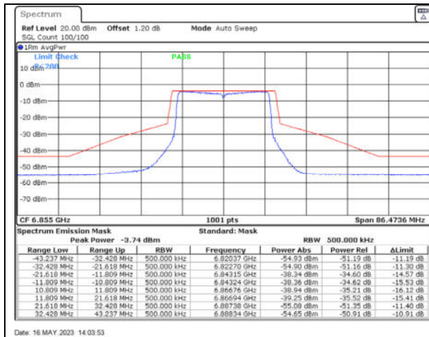
802.11ax20 / 6855MHz / Chain A - Beamforming
