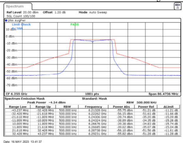
802.11ax20 / 6255MHz / Chain B - Beamforming
