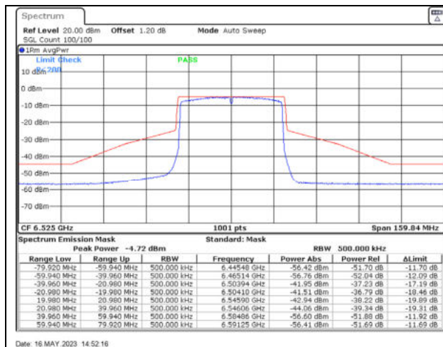
802.11ax40 / 6525MHz / Chain C - Beamforming
