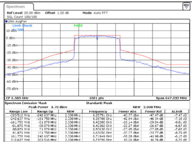
802.11ax160 / 6505MHz / Chain B - CDD
