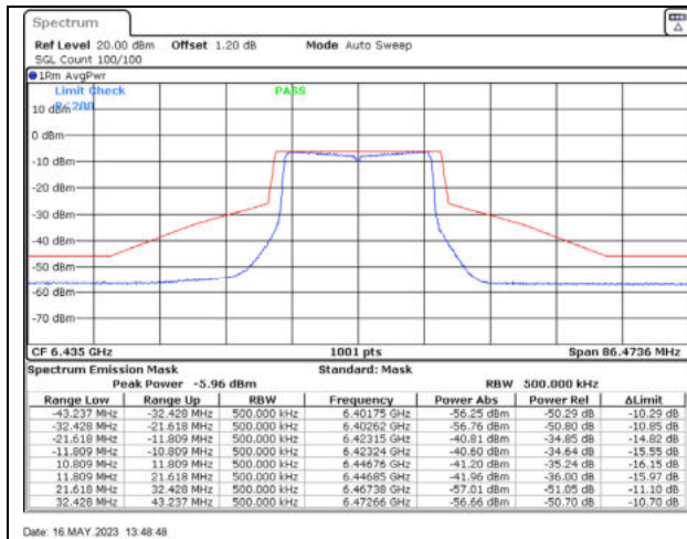
802.11ax20 / 6435MHz / Chain C - Beamforming
