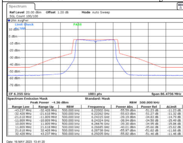
802.11ax20 / 6255MHz / Chain A - Beamforming
