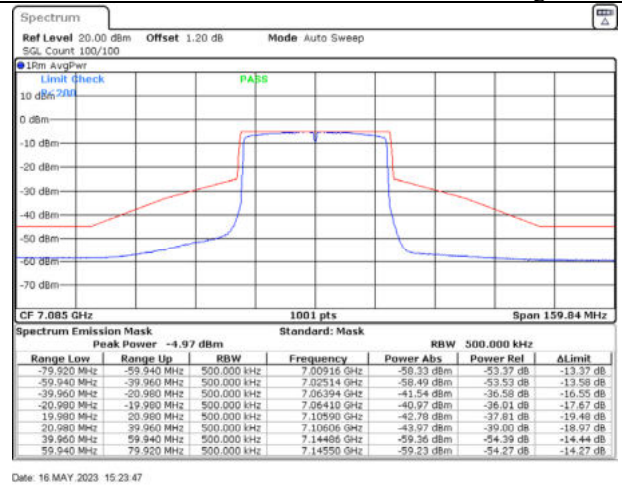
802.11ax40 / 7085MHz / Chain B - Beamforming
