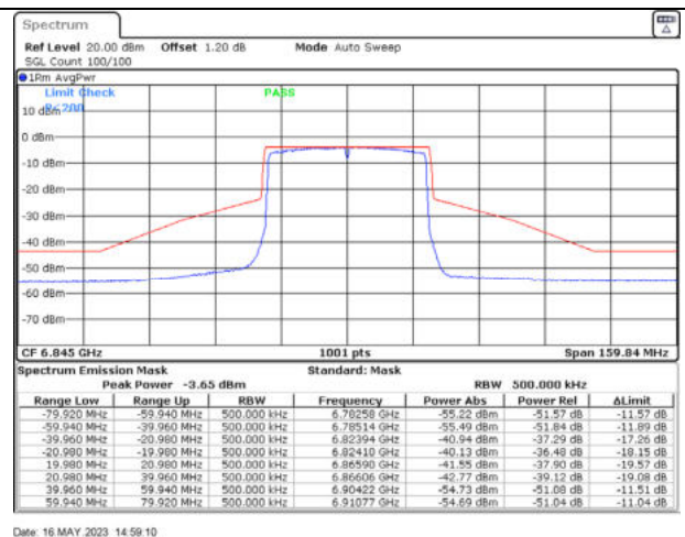
802.11ax40 / 6845MHz / Chain D - Beamforming
