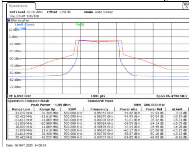
802.11ax20 / 6895MHz / Chain C - Beamforming
