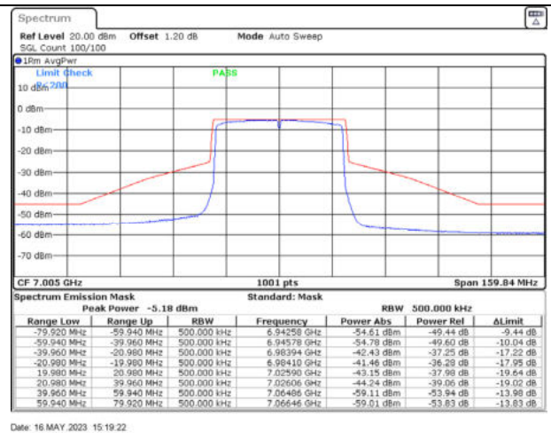
802.11ax40 / 7005MHz / Chain D - Beamforming
