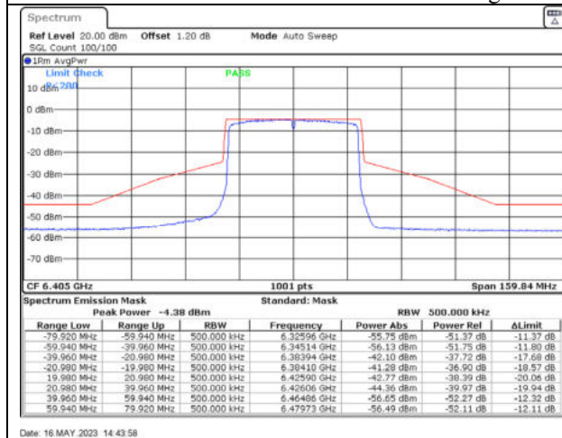
802.11ax40 / 6405MHz / Chain A - Beamforming
