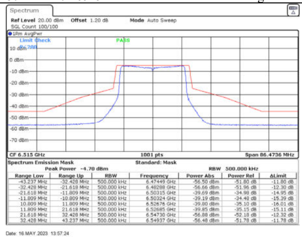
802.11ax20 / 6515MHz / Chain D - Beamforming
