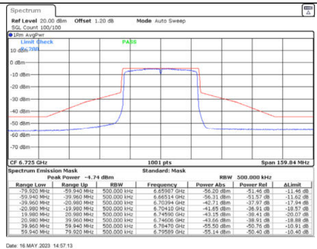
802.11ax40 / 6725MHz / Chain B - Beamforming
