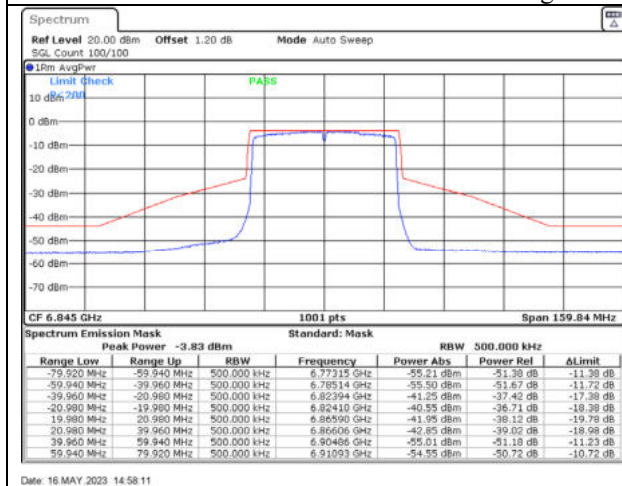
802.11ax40 / 6845MHz / Chain A - Beamforming
