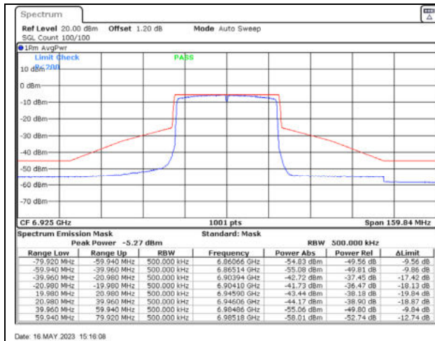
802.11ax40 / 6925MHz / Chain A - Beamforming
