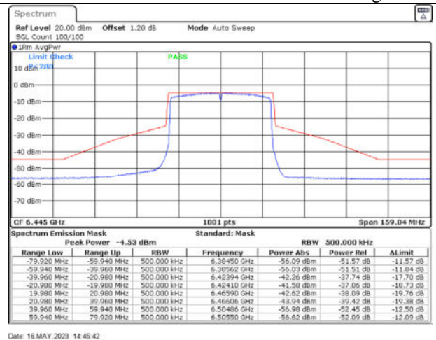
802.11ax40 / 6445MHz / Chain D - Beamforming
