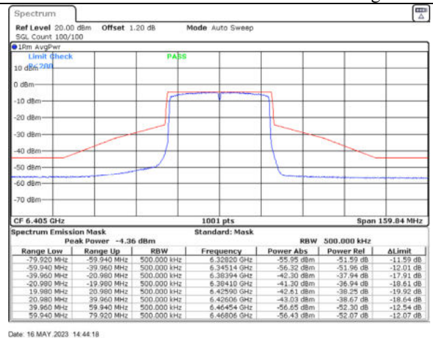
802.11ax40 / 6405MHz / Chain B - Beamforming
