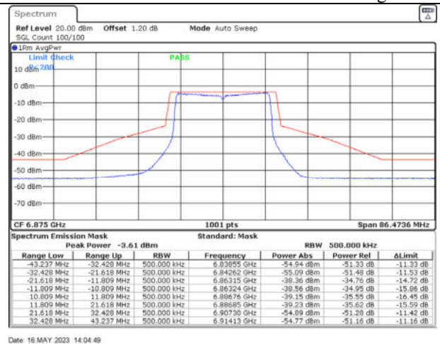
802.11ax20 / 6875MHz / Chain B - Beamforming
