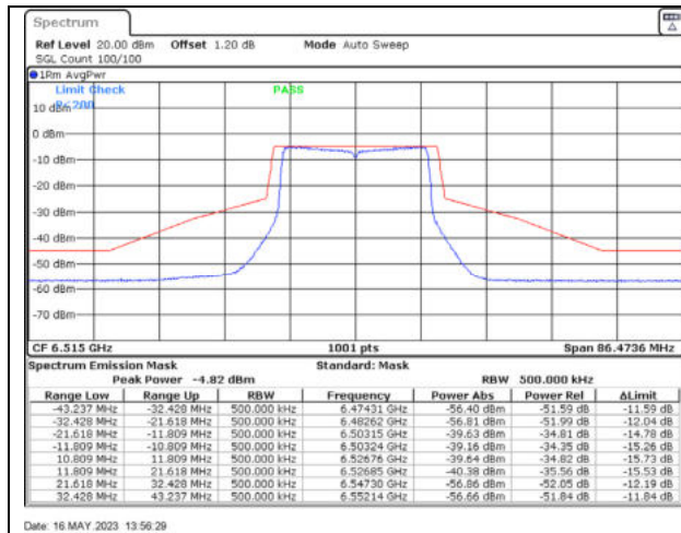
802.11ax20 / 6515MHz / Chain A - Beamforming
