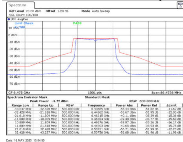
802.11ax20 / 6475MHz / Chain C - Beamforming
