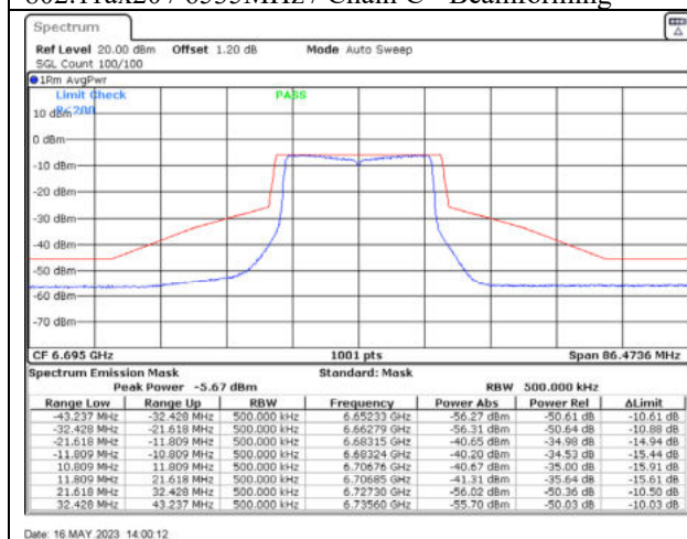
802.11ax20 / 6695MHz / Chain A - Beamforming
