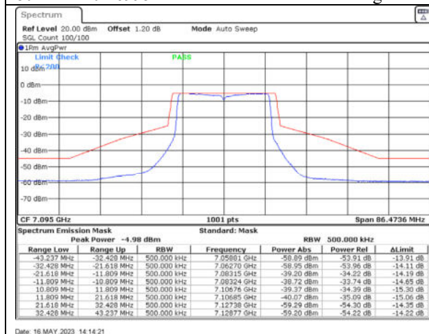
802.11ax20 / 7095MHz / Chain A - Beamforming
