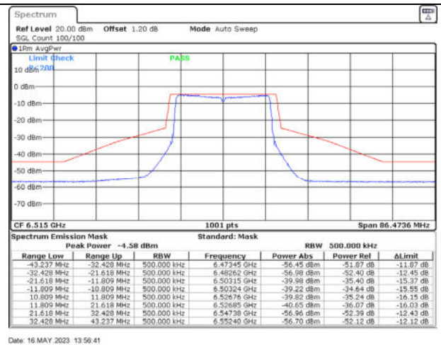
802.11ax20 / 6515MHz / Chain B - Beamforming
