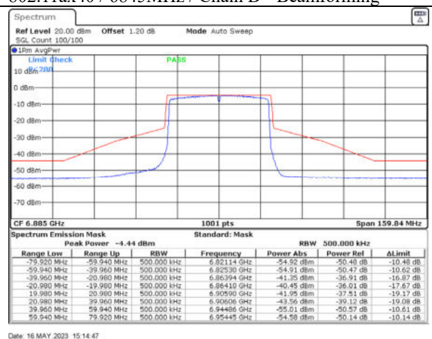
802.11ax40 / 6885MHz / Chain B - Beamforming
