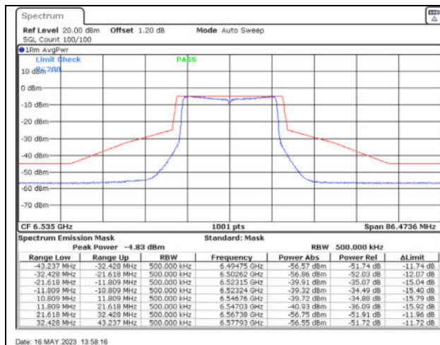
802.11ax20 / 6535MHz / Chain C - Beamforming
