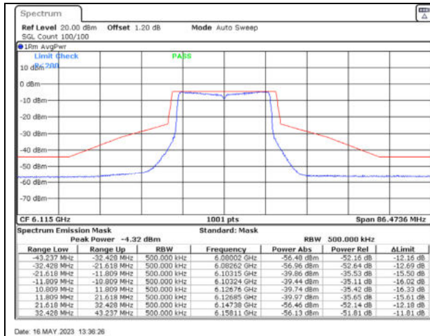
802.11ax20 / 6115MHz / Chain A - Beamforming
