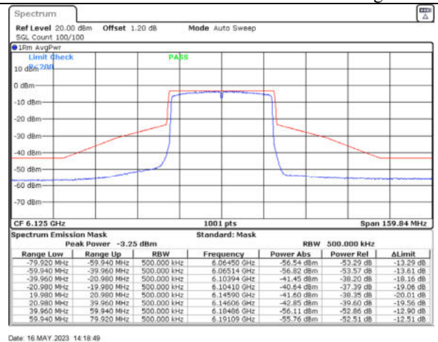
802.11ax40 / 6125MHz / Chain D - Beamforming
