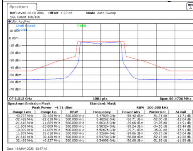
802.11ax20 / 6515MHz / Chain C - Beamforming
