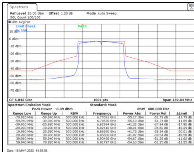
802.11ax40 / 6845MHz / Chain C - Beamforming
