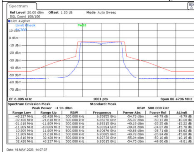
802.11ax20 / 6895MHz / Chain A - Beamforming
