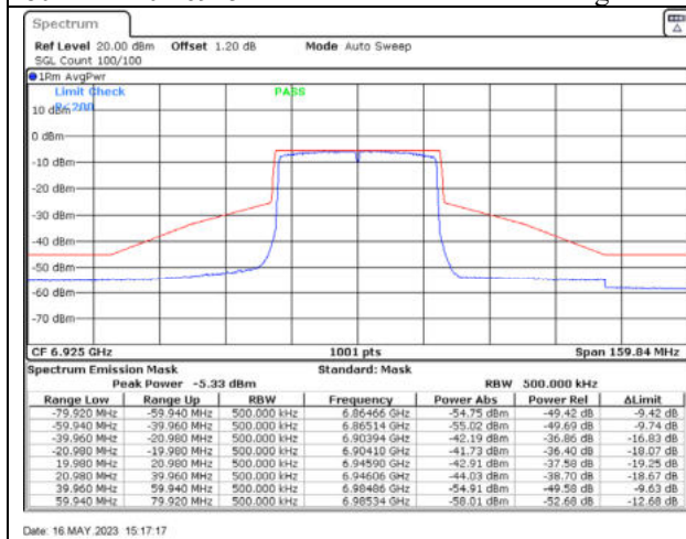
802.11ax40 / 6925MHz / Chain C - Beamforming
