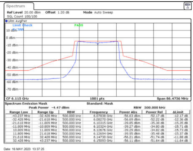
802.11ax20 / 6115MHz / Chain B - Beamforming
