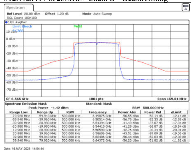
802.11ax40 / 6565MHz / Chain B - Beamforming
