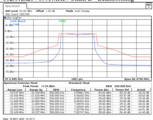
802.11ax20 / 6995MHz / Chain D - Beamforming
