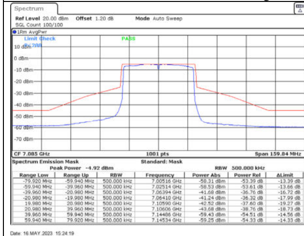
802.11ax40 / 7085MHz / Chain C - Beamforming
