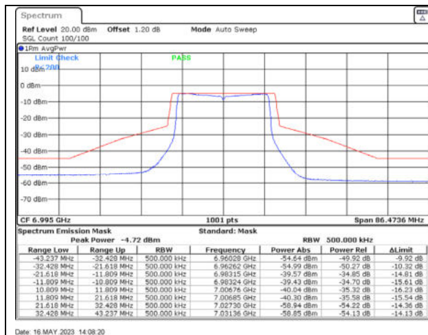
802.11ax20 / 6995MHz / Chain A - Beamforming
