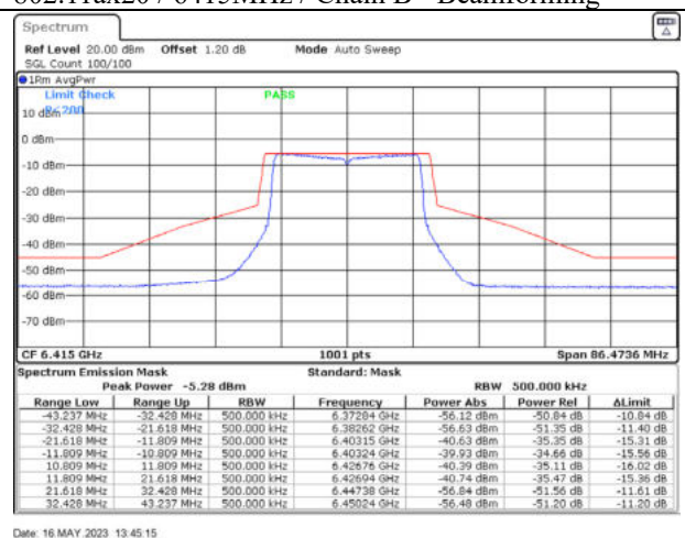
802.11ax20 / 6415MHz / Chain D - Beamforming
