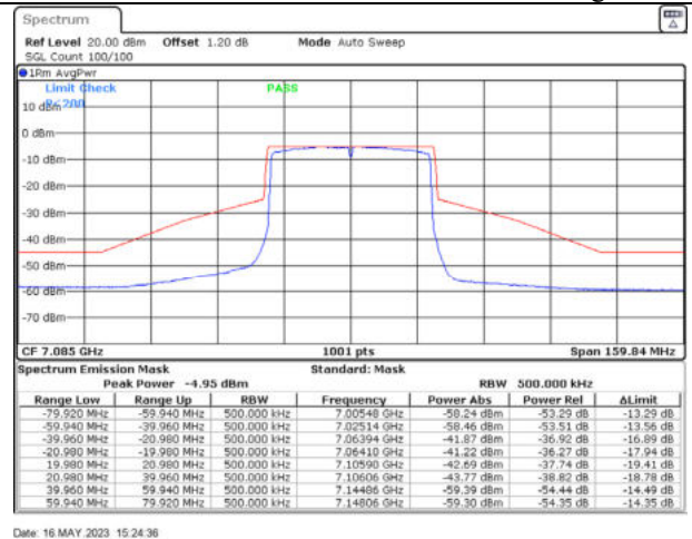
802.11ax40 / 7085MHz / Chain D - Beamforming
