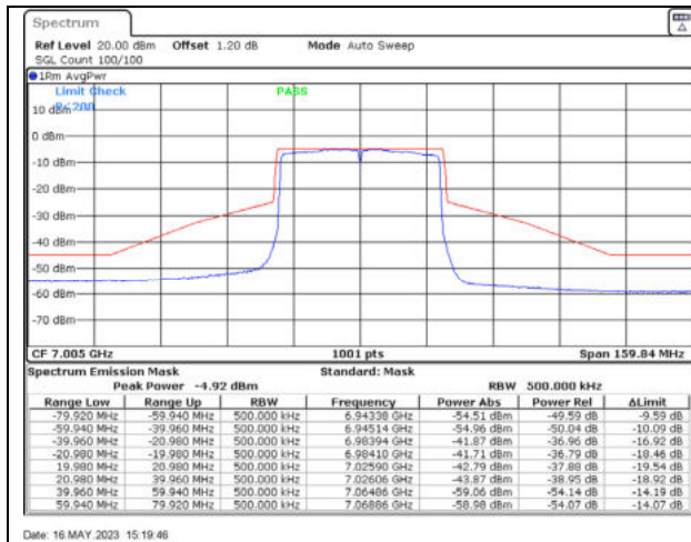
802.11ax40 / 7005MHz / Chain C - Beamforming
