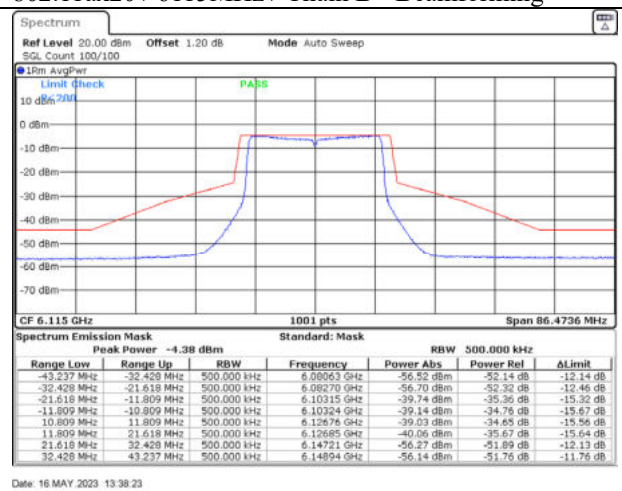
802.11ax20 / 6115MHz / Chain D - Beamforming
