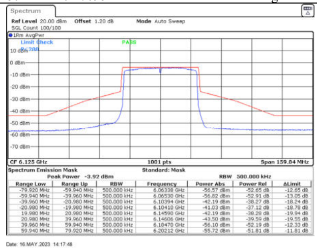
802.11ax40 / 6125MHz / Chain B - Beamforming
