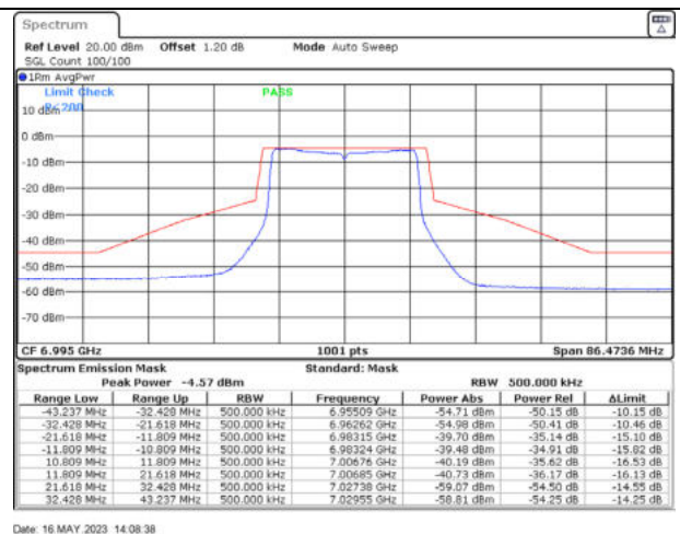
802.11ax20 / 6995MHz / Chain B - Beamforming
