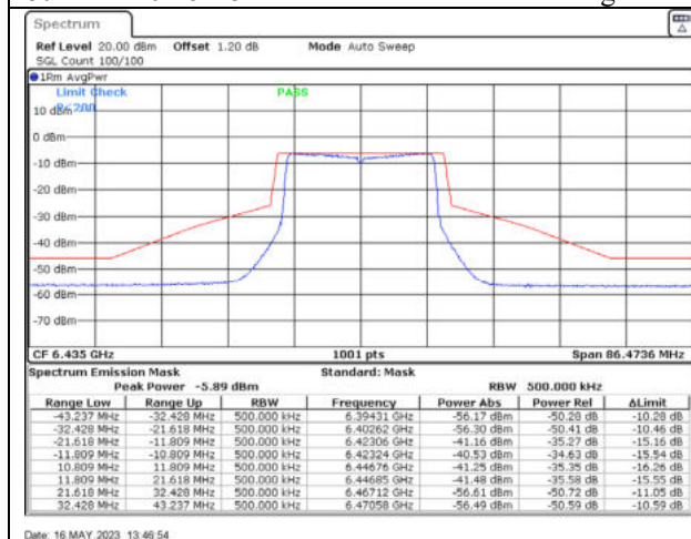
802.11ax20 / 6435MHz / Chain A - Beamforming
