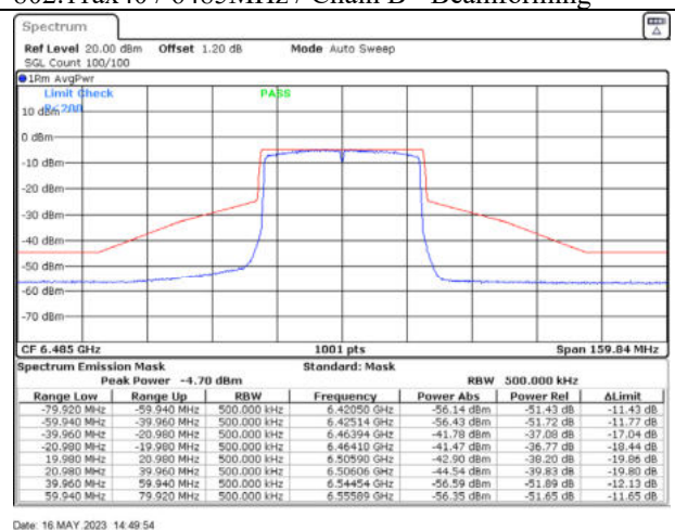
802.11ax40 / 6485MHz / Chain D - Beamforming
