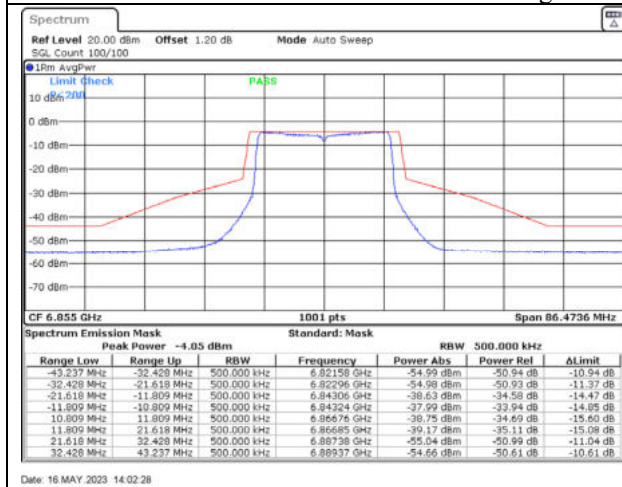
802.11ax20 / 6855MHz / Chain C - Beamforming
