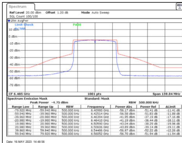
802.11ax40 / 6485MHz / Chain A - Beamforming
