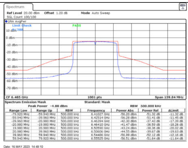
802.11ax40 / 6485MHz / Chain B - Beamforming
