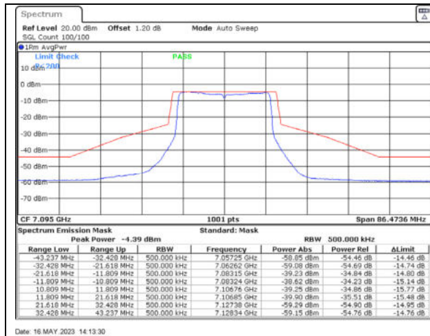
802.11ax20 / 7095MHz / Chain C - Beamforming
