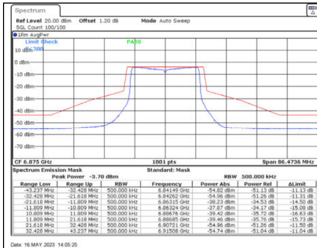
802.11ax20 / 6875MHz / Chain C - Beamforming
