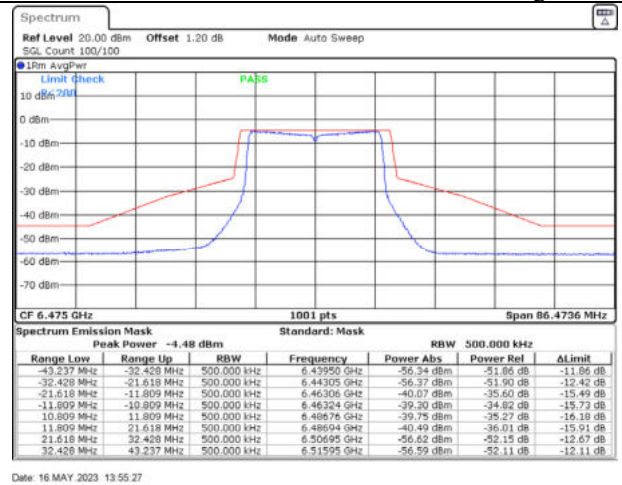
802.11ax20 / 6475MHz / Chain B - Beamforming
