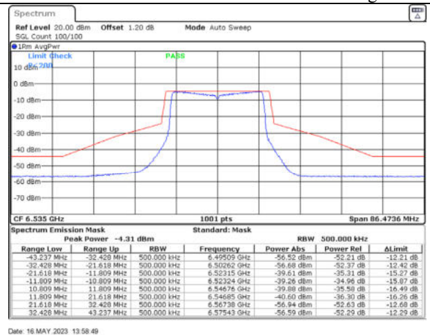
802.11ax20 / 6535MHz / Chain B - Beamforming
