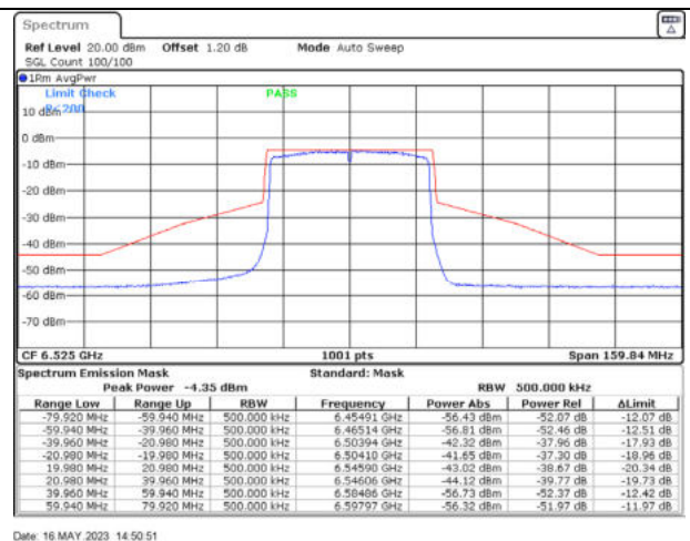
802.11ax40 / 6525MHz / Chain D - Beamforming
