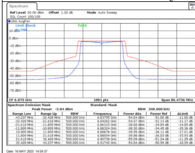
802.11ax20 / 6875MHz / Chain A - Beamforming
