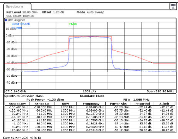
802.11ax80 / 6145MHz / Chain B - Beamforming
