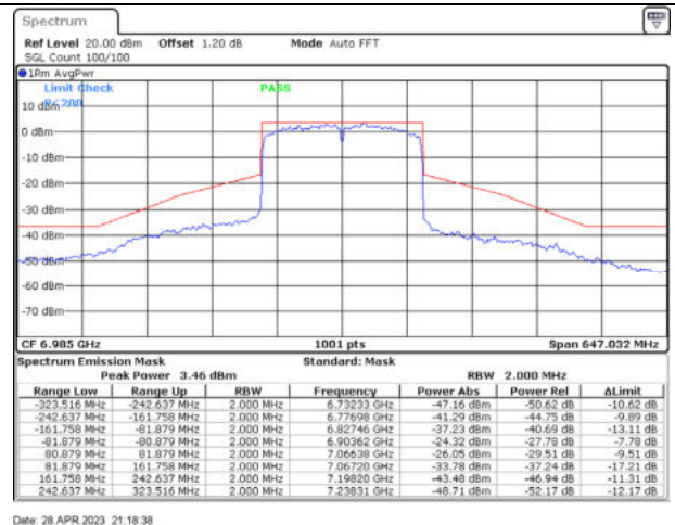
802.11ax160 / 6985MHz / Chain D - CDD
