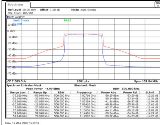
802.11ax40 / 7085MHz / Chain A - Beamforming
