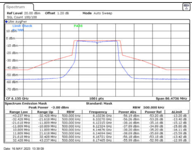
802.11ax20 / 6135MHz / Chain D - Beamforming
