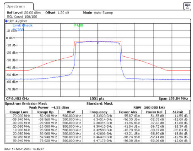
802.11ax40 / 6405MHz / Chain D - Beamforming
