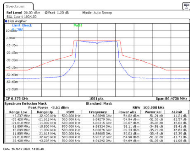
802.11ax20 / 6875MHz / Chain D - Beamforming
