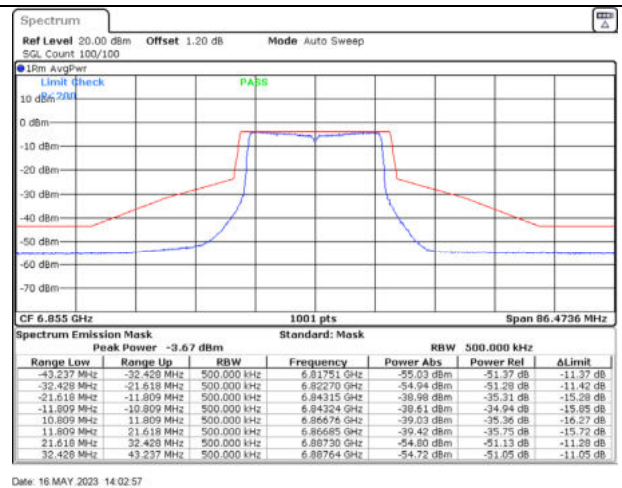
802.11ax20 / 6855MHz / Chain B - Beamforming
