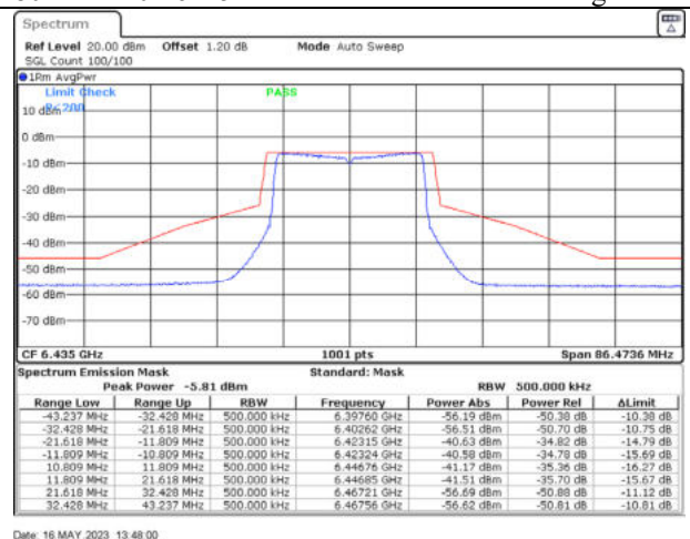
802.11ax20 / 6435MHz / Chain B - Beamforming
