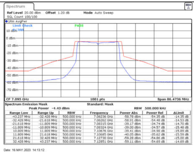
802.11ax20 / 7095MHz / Chain D - Beamforming
