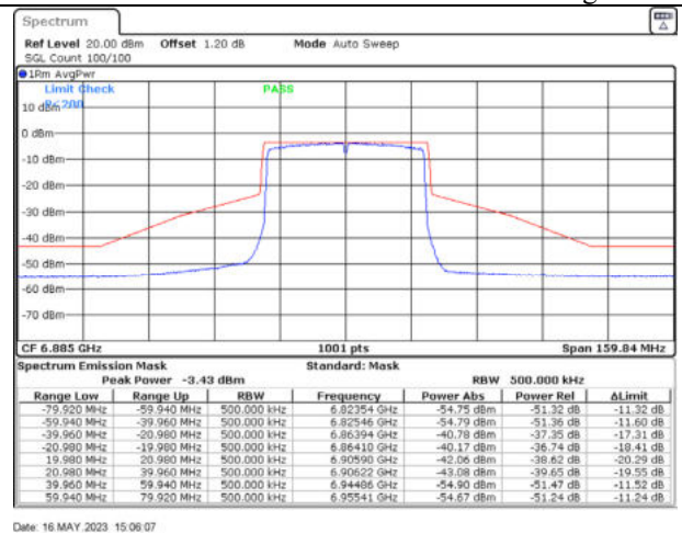
802.11ax40 / 6885MHz / Chain D - Beamforming
