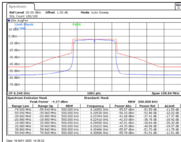
802.11ax40 / 6245MHz / Chain A - Beamforming
