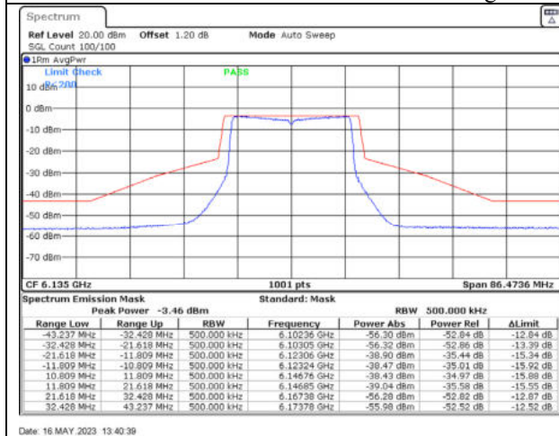
802.11ax20 / 6135MHz / Chain A - Beamforming
