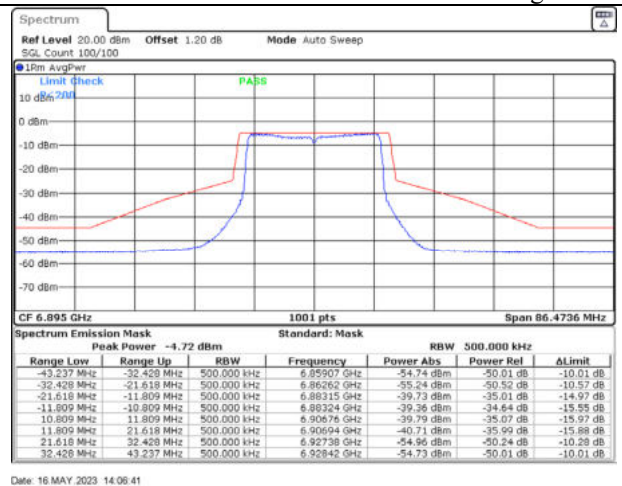
802.11ax20 / 6895MHz / Chain D - Beamforming
