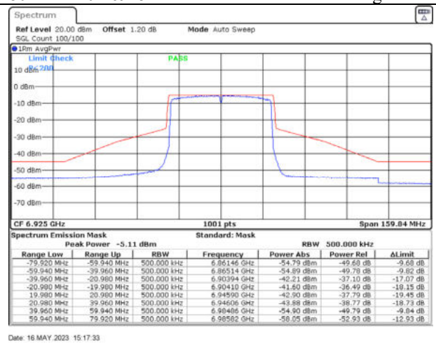
802.11ax40 / 6925MHz / Chain D - Beamforming
