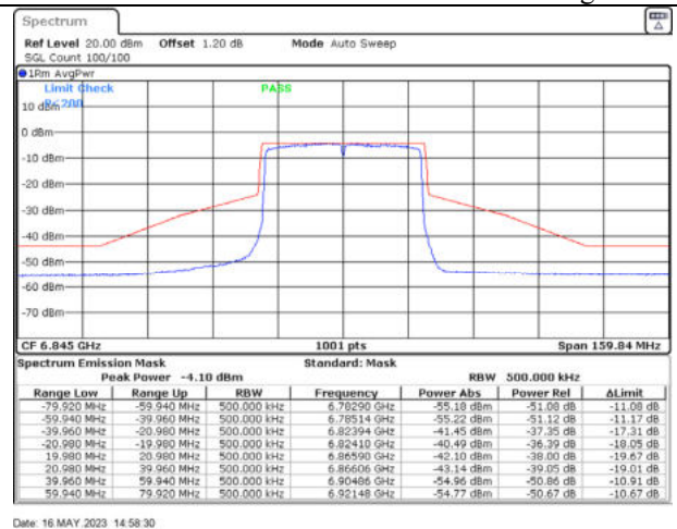
802.11ax40 / 6845MHz / Chain B - Beamforming
