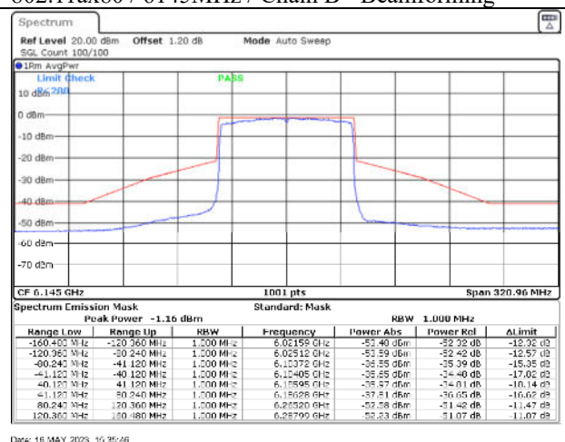
802.11ax80 / 6145MHz / Chain D - Beamforming
