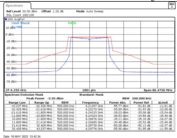
802.11ax20 / 6255MHz / Chain D - Beamforming
