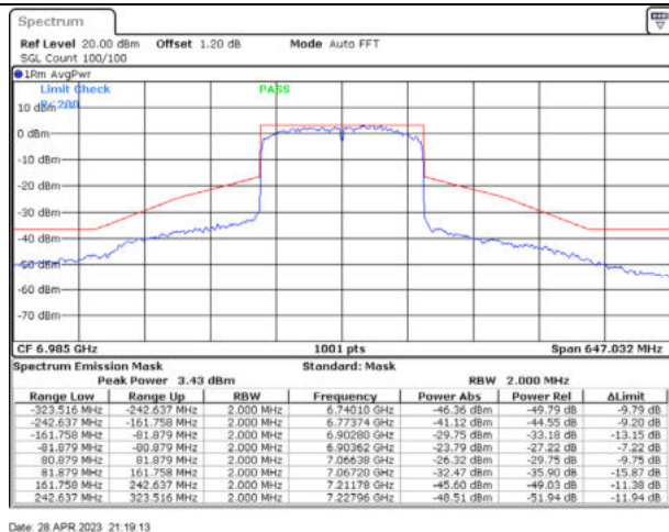
802.11ax160 / 6985MHz / Chain C - CDD
