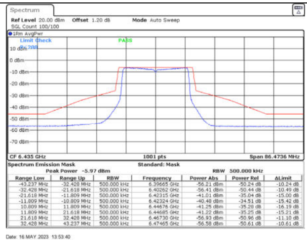
802.11ax20 / 6435MHz / Chain D - Beamforming
