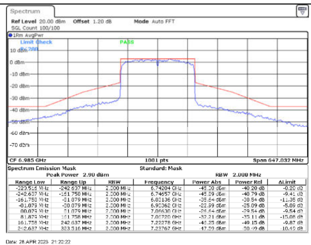
802.11ax160 / 6985MHz / Chain B - CDD
