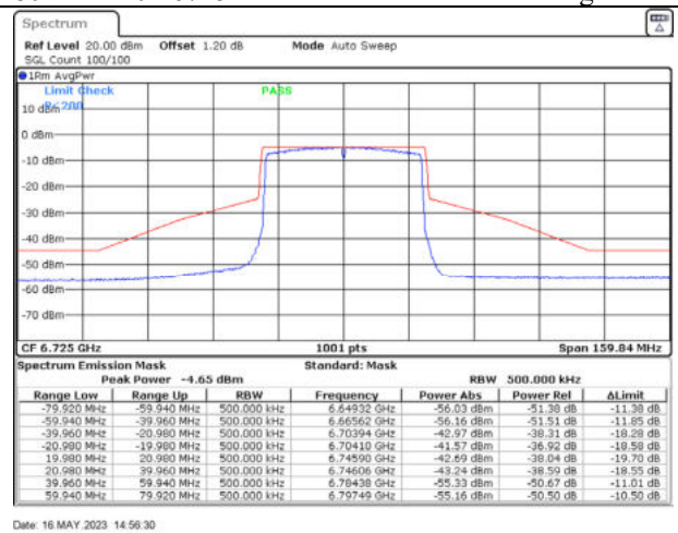
802.11ax40 / 6725MHz / Chain D - Beamforming
