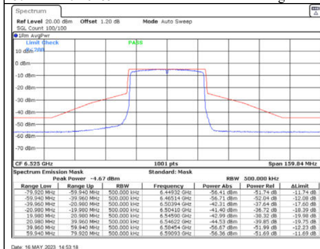
802.11ax40 / 6525MHz / Chain A - Beamforming
