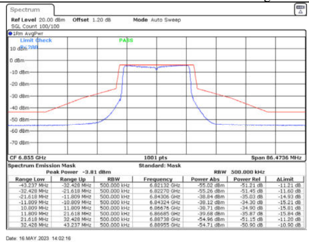
802.11ax20 / 6855MHz / Chain D - Beamforming
