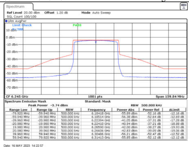
802.11ax40 / 6245MHz / Chain D - Beamforming
