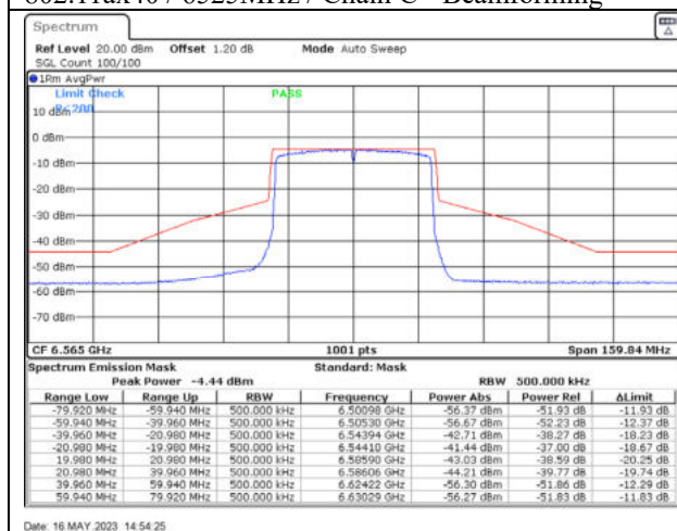
802.11ax40 / 6565MHz / Chain A - Beamforming
