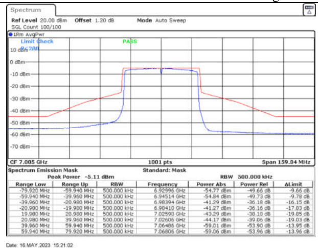
802.11ax40 / 7005MHz / Chain B - Beamforming
