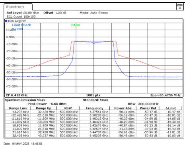
802.11ax20 / 6415MHz / Chain B - Beamforming
