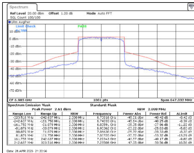
802.11ax160 / 6985MHz / Chain A - CDD
