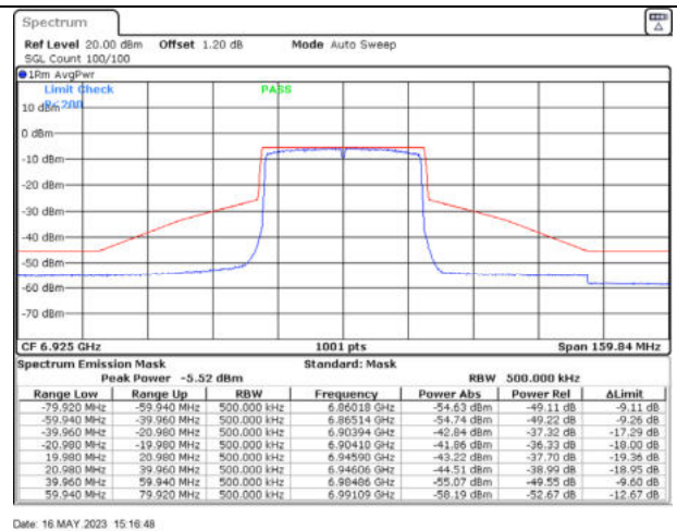
802.11ax40 / 6925MHz / Chain B - Beamforming
