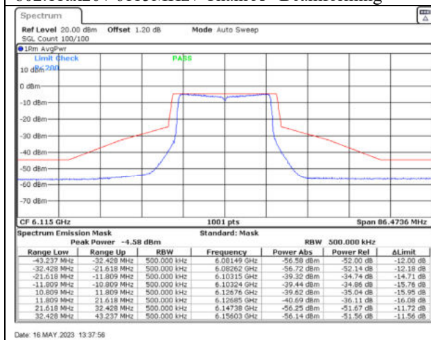
802.11ax20 / 6115MHz / Chain C - Beamforming
