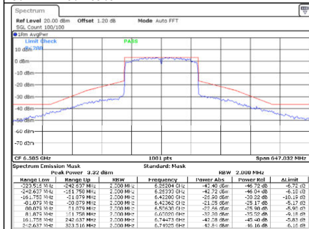
802.11ax160 / 6505MHz / Chain A - CDD
