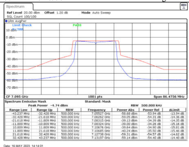
802.11ax20 / 7095MHz / Chain B - Beamforming
