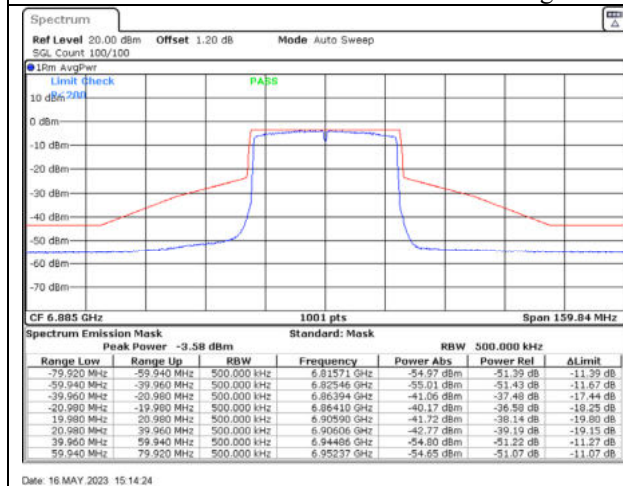
802.11ax40 / 6885MHz / Chain C - Beamforming
