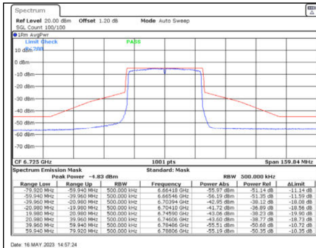
802.11ax40 / 6725MHz / Chain A - Beamforming
