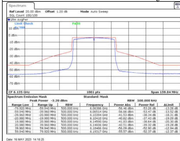
802.11ax40 / 6125MHz / Chain C - Beamforming
