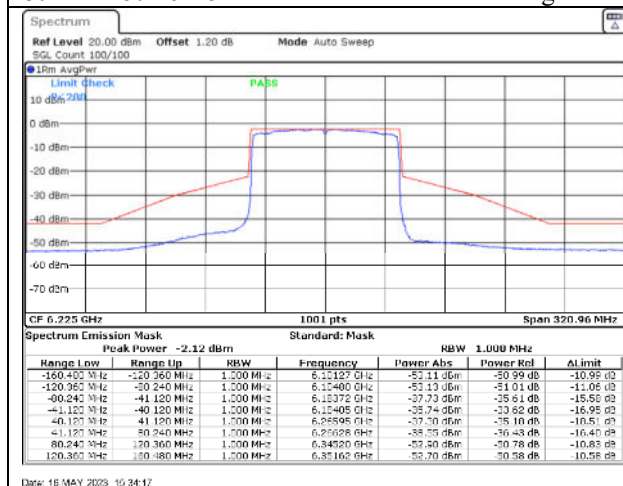
802.11ax80 / 6225MHz / Chain A - Beamforming
