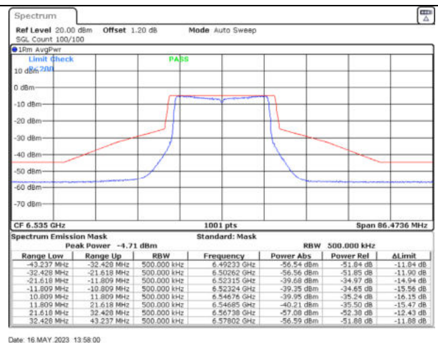
802.11ax20 / 6535MHz / Chain D - Beamforming
