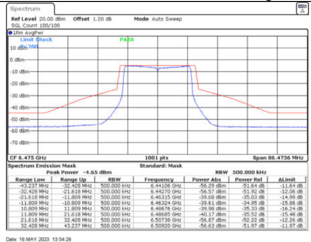
802.11ax20 / 6475MHz / Chain D - Beamforming
