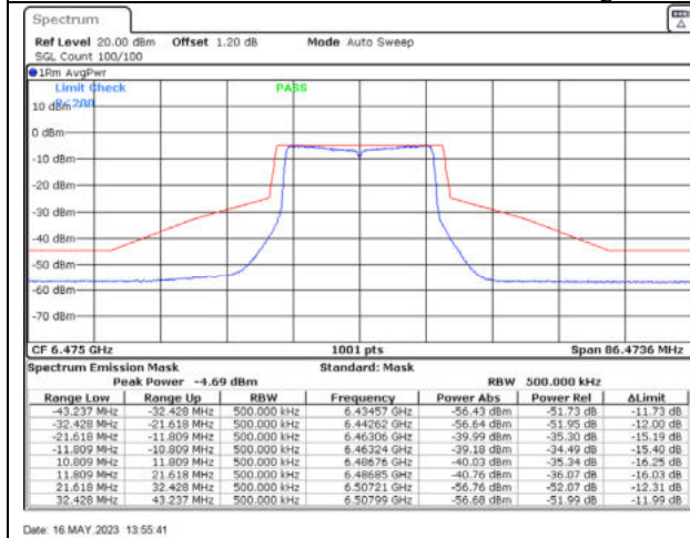
802.11ax20 / 6475MHz / Chain A - Beamforming
