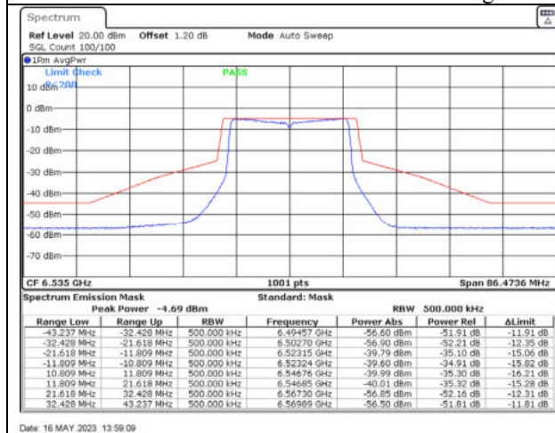
802.11ax20 / 6535MHz / Chain A - Beamforming
