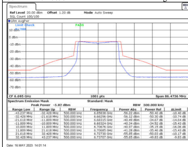
802.11ax20 / 6695MHz / Chain C - Beamforming
