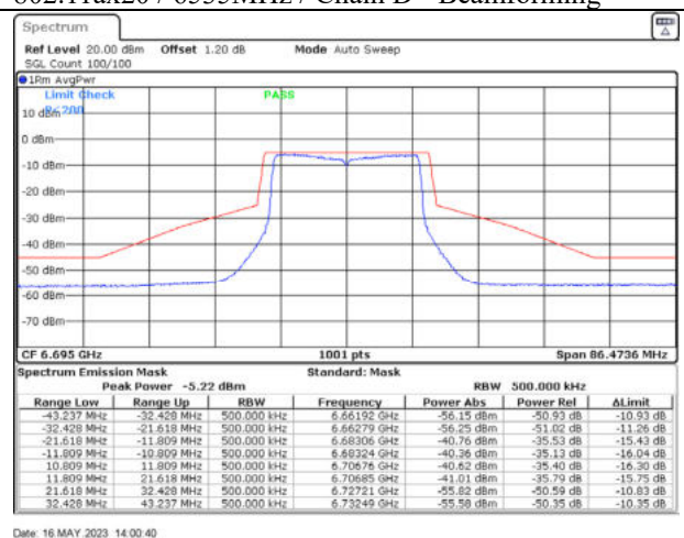
802.11ax20 / 6695MHz / Chain B - Beamforming
