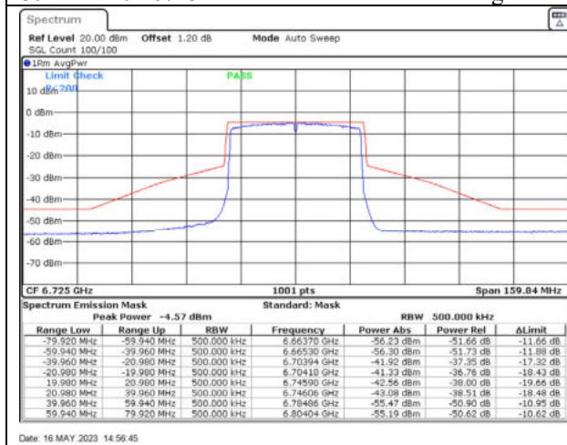
802.11ax40 / 6725MHz / Chain C - Beamforming
