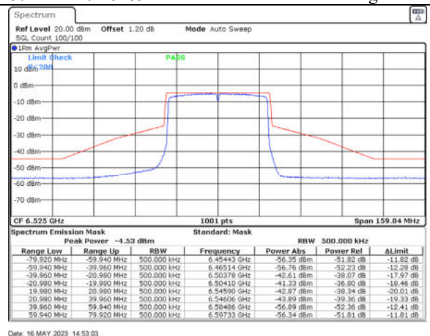
802.11ax40 / 6525MHz / Chain B - Beamforming
