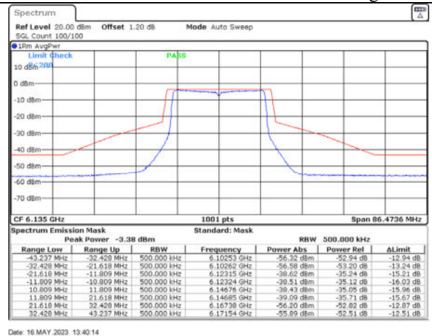
802.11ax20 / 6135MHz / Chain B - Beamforming
