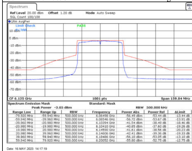
802.11ax40 / 6125MHz / Chain A - Beamforming
