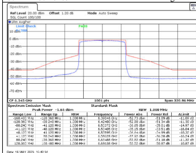
802.11ax80 / 6545MHz / Chain A - Beamforming
