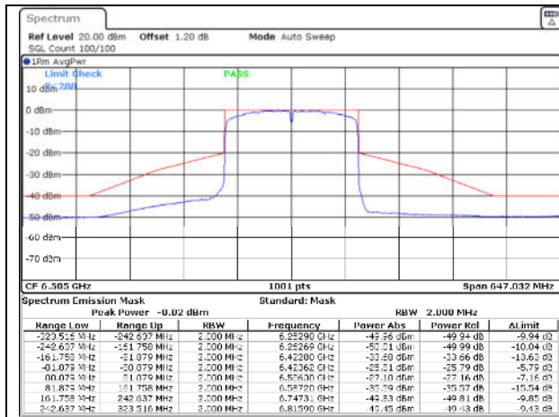
802.11ax160 / 6505MHz / Chain C - Beamforming
