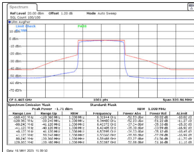
802.11ax80 / 6465MHz / Chain A - Beamforming
