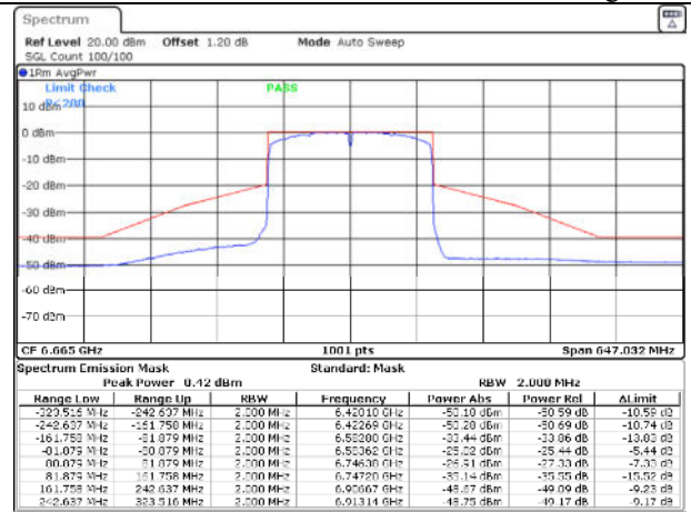
802.11ax160 / 6665MHz / Chain B - Beamforming
