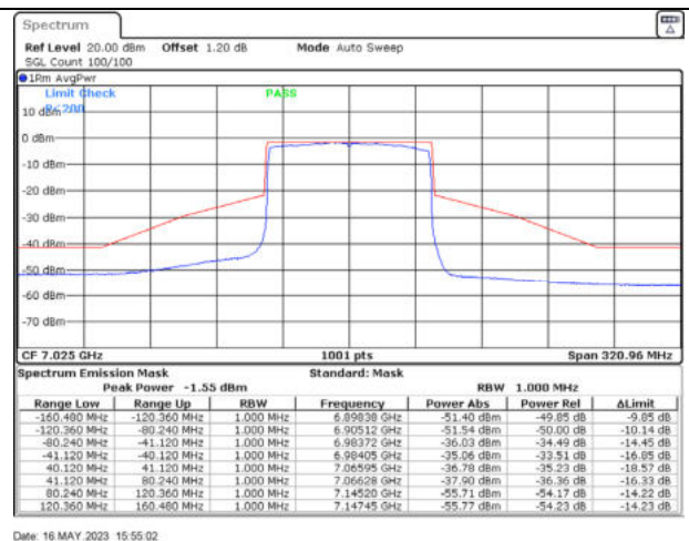
802.11ax80 / 7025MHz / Chain D - Beamforming
