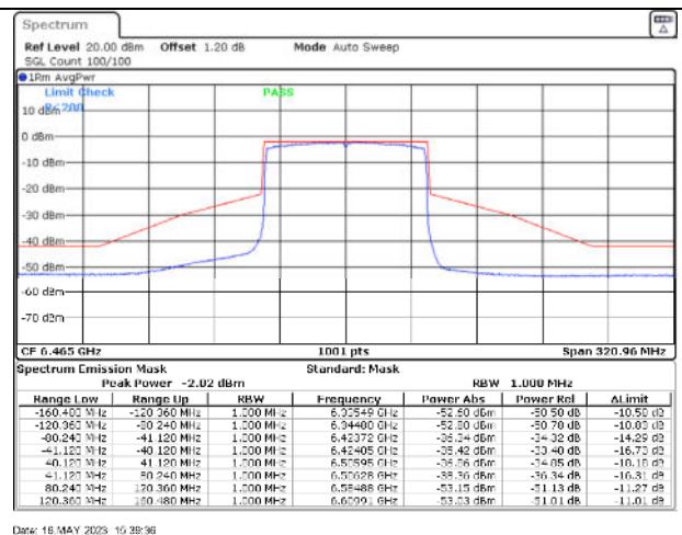
802.11ax80 / 6465MHz / Chain B - Beamforming
