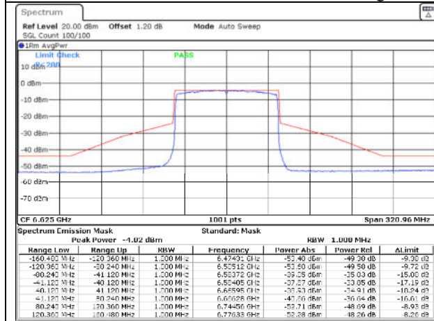
802.11ax80 / 6625MHz / Chain A - Beamforming
