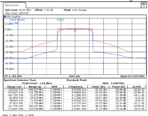
802.11ax160 / 6185MHz / Chain D - Beamforming
