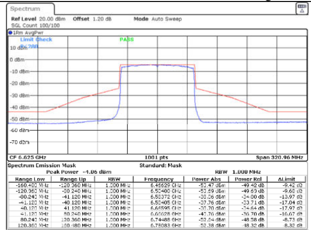
802.11ax80 / 6625MHz / Chain B - Beamforming
