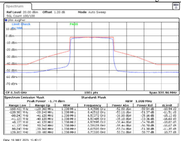
802.11ax80 / 6545MHz / Chain B - Beamforming
