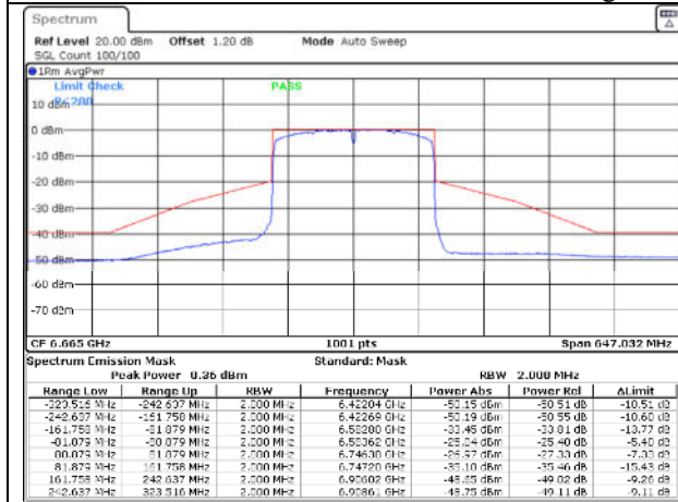
802.11ax160 / 6665MHz / Chain A - Beamforming
