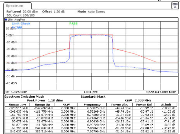
802.11ax160 / 6825MHz / Chain B - Beamforming
