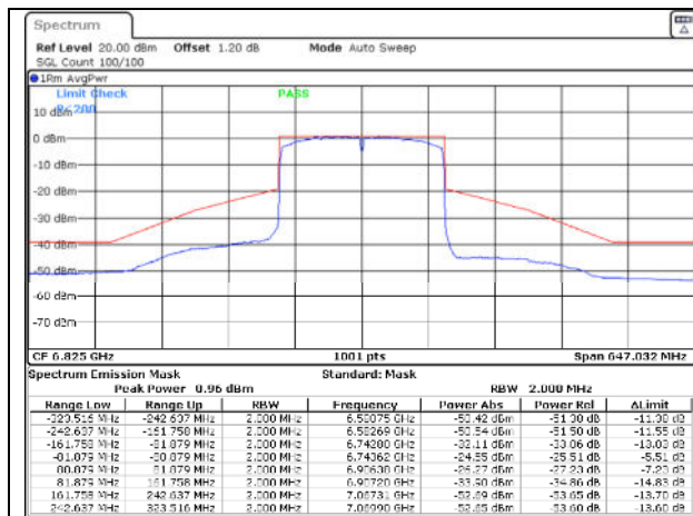
802.11ax160 / 6825MHz / Chain A - Beamforming
