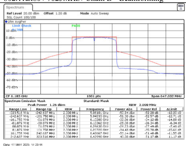
802.11ax160 / 6185MHz / Chain B - Beamforming
