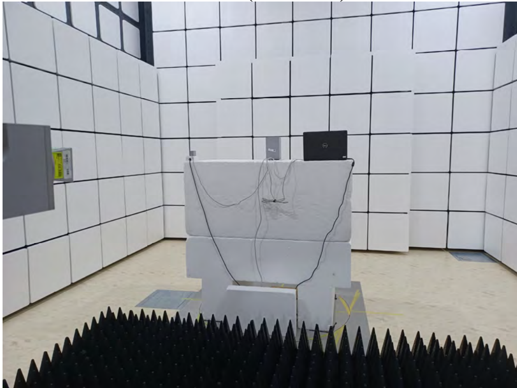
Radiated Test (Above 18GHz)
