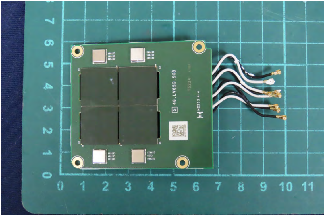
(26) EUT Photo_5G FR2 Array antenna
