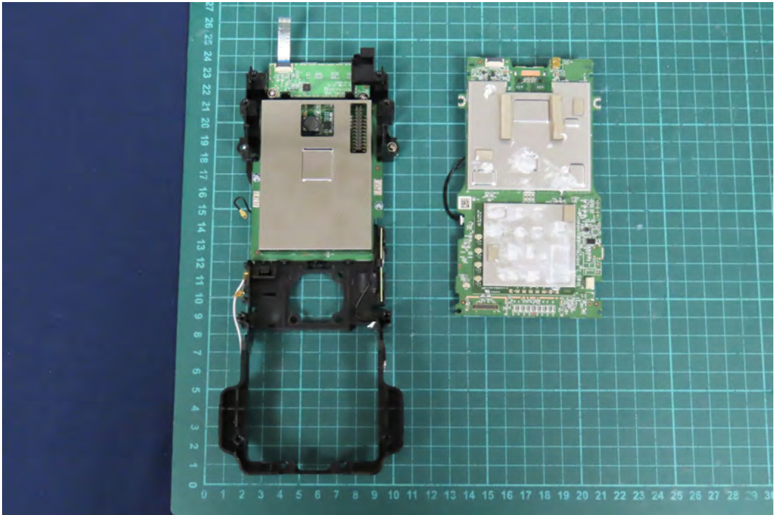
(28) EUT Photo
