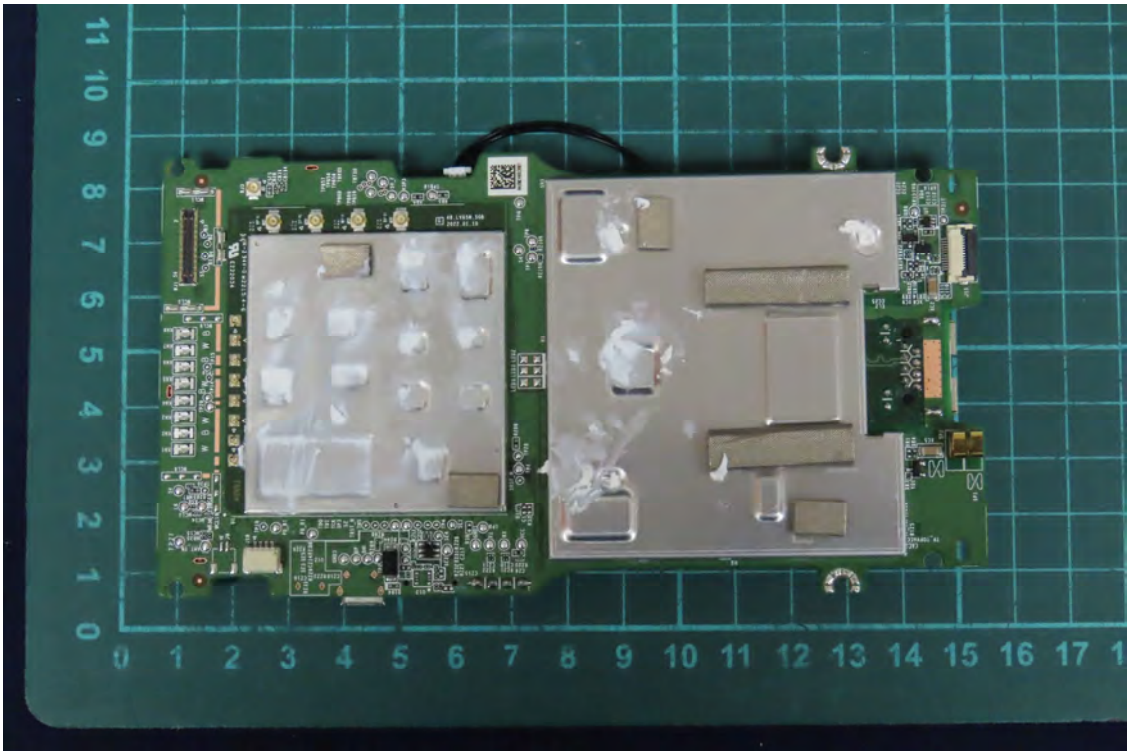
(29) EUT Photo
