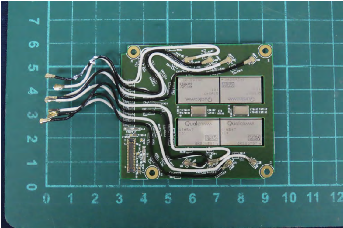
(25) EUT Photo_5G FR2 Chip
