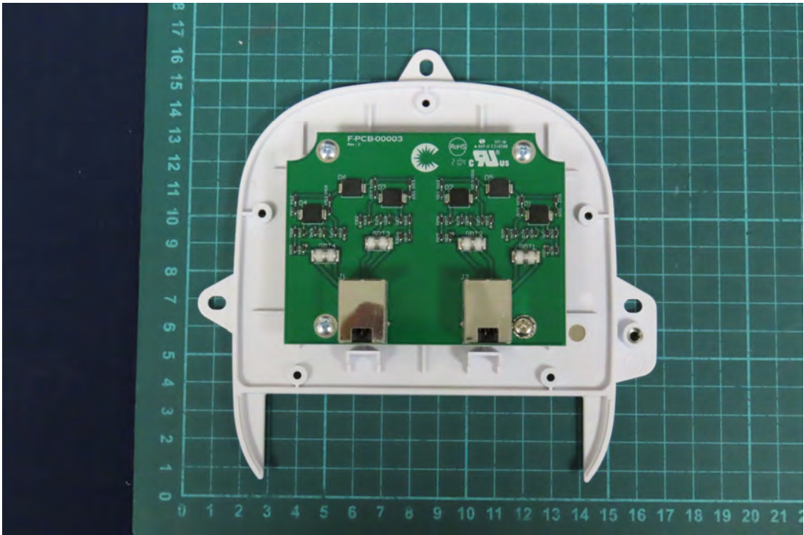
(73) EUT Photo
