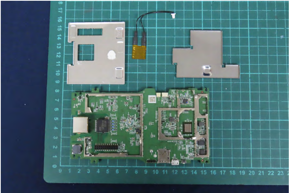
(34) EUT Photo
