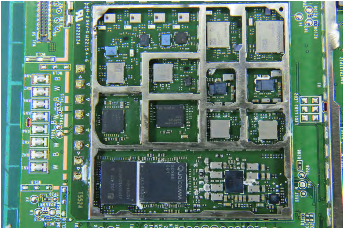
(32) EUT Photo
