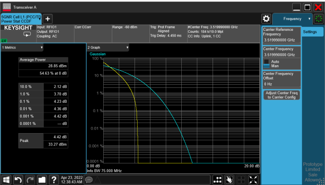
5G NR n77_CH634666_60M_1RB_16-QAM_Ratio
