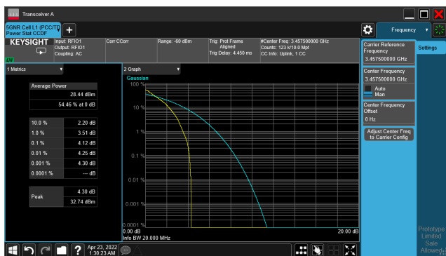
5G NR n77_CH630500_15M_1RB_16-QAM_Ratio
