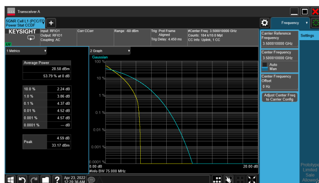
5G NR n77 CH633334 70M 1RB 16-QAM Ratio
