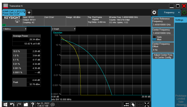
5G NR n77_CH630334_10M_1RB_16-QAM_Ratio
