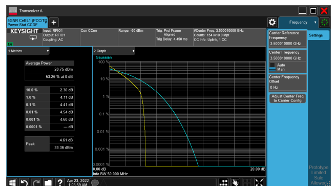
5G NR n77_CH633334_50M_1RB_16-QAM_Ratio
