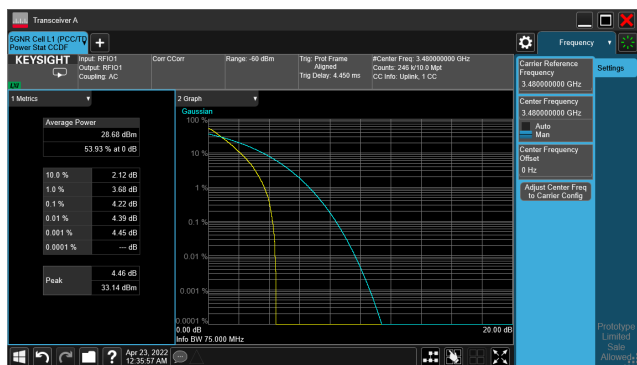
5G NR n77_CH632000_60M_1RB_16-QAM_Ratio
