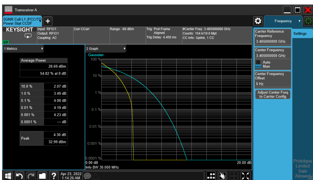
5G NR n77_CH631000_30M_1RB_16-QAM_Ratio
