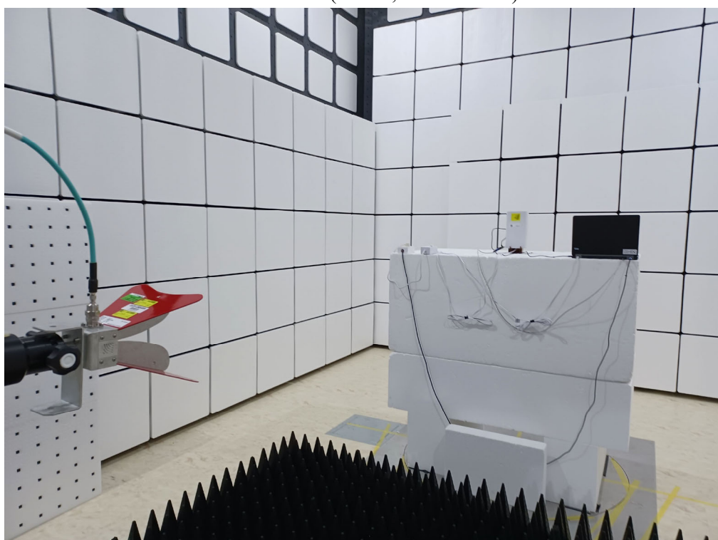
Radiated Test (Indoor, Above 1GHz)
