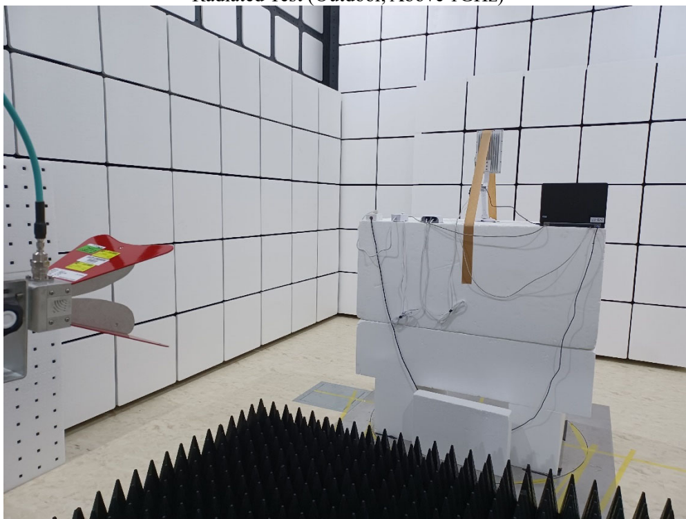
Radiated Test (Outdoor, Above 18GHz)
