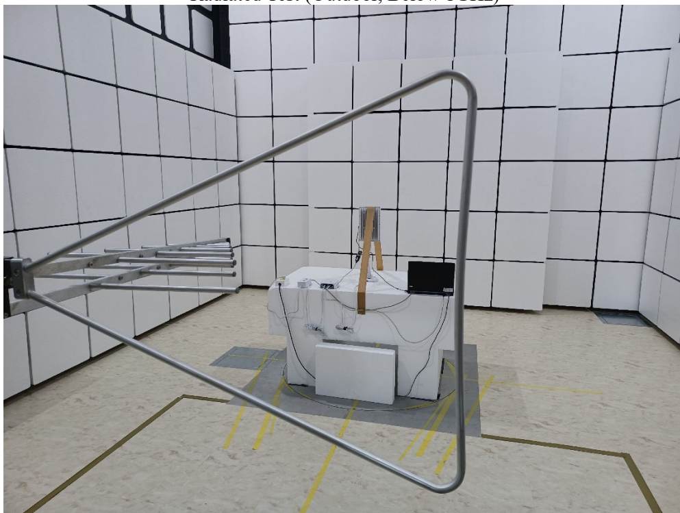
Radiated Test (Outdoor, Below 1GHz)
