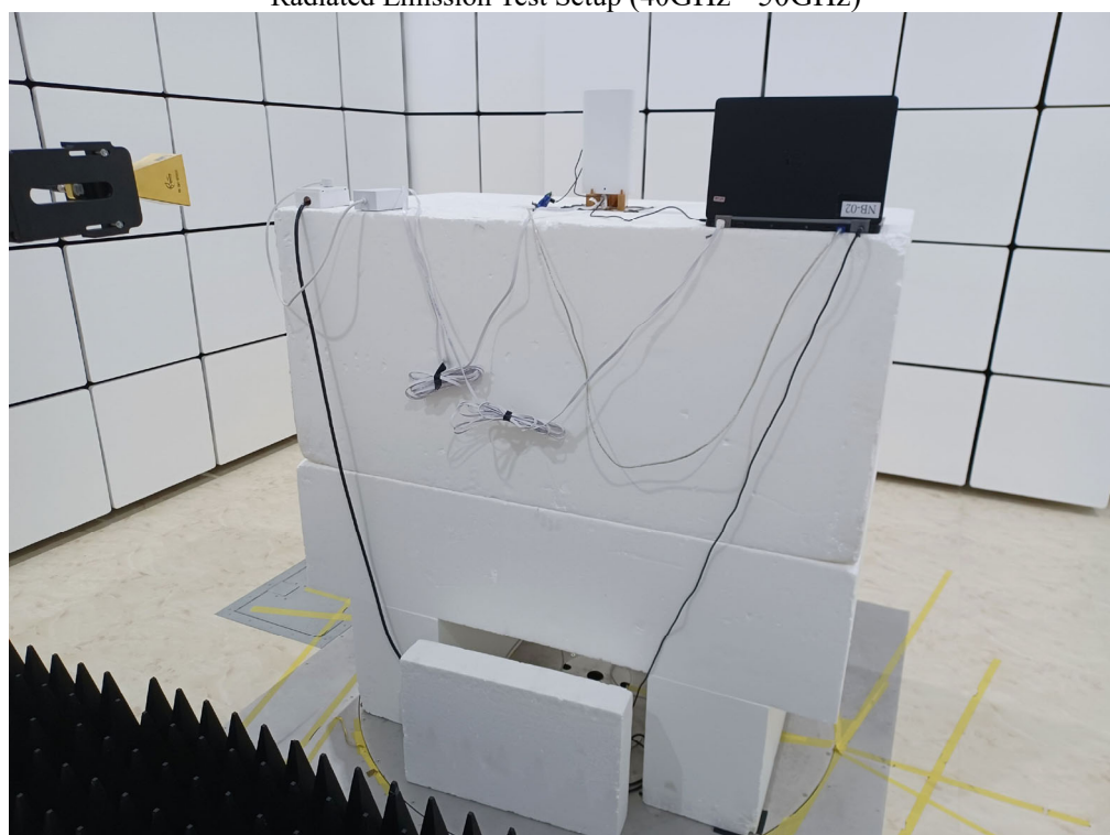
Radiated Emission Test Setup (40GHz - 50GHz)
