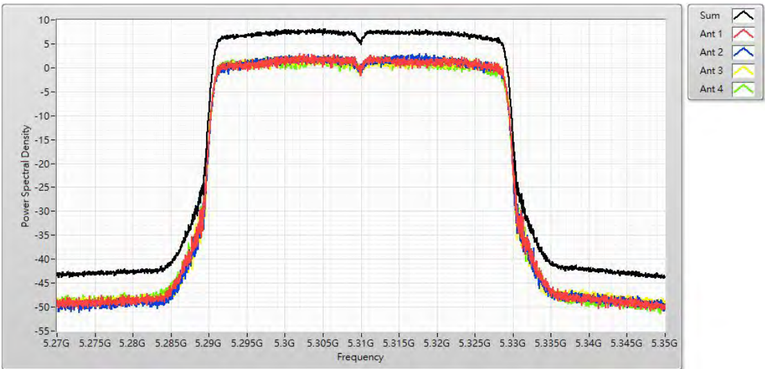
Channel 62 (5310MHz)
