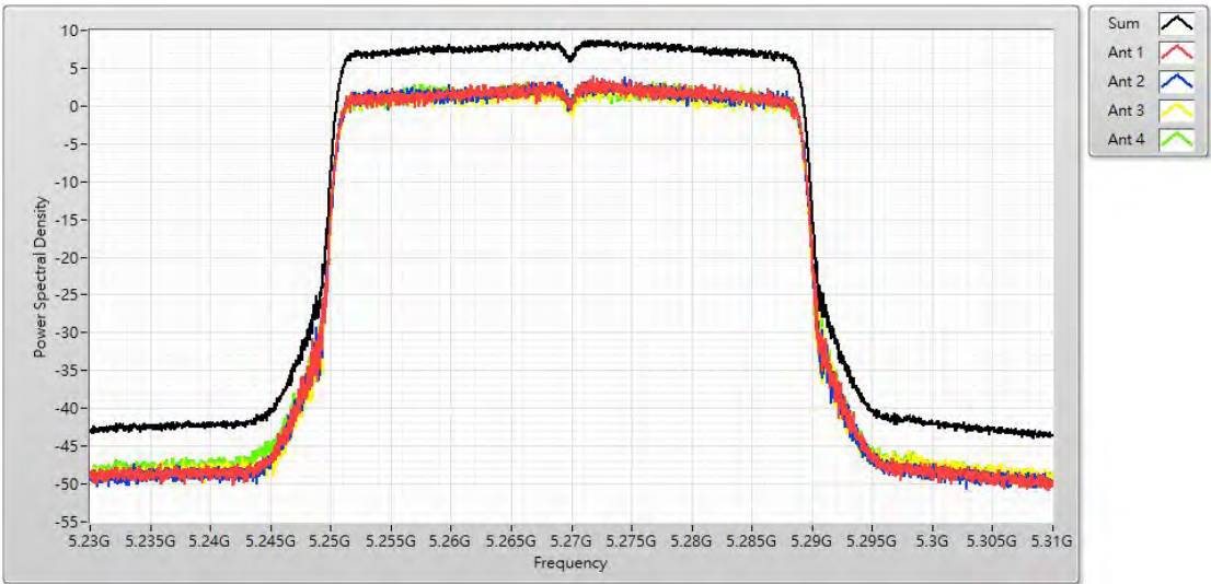
Channel 54 (5270MHz)
