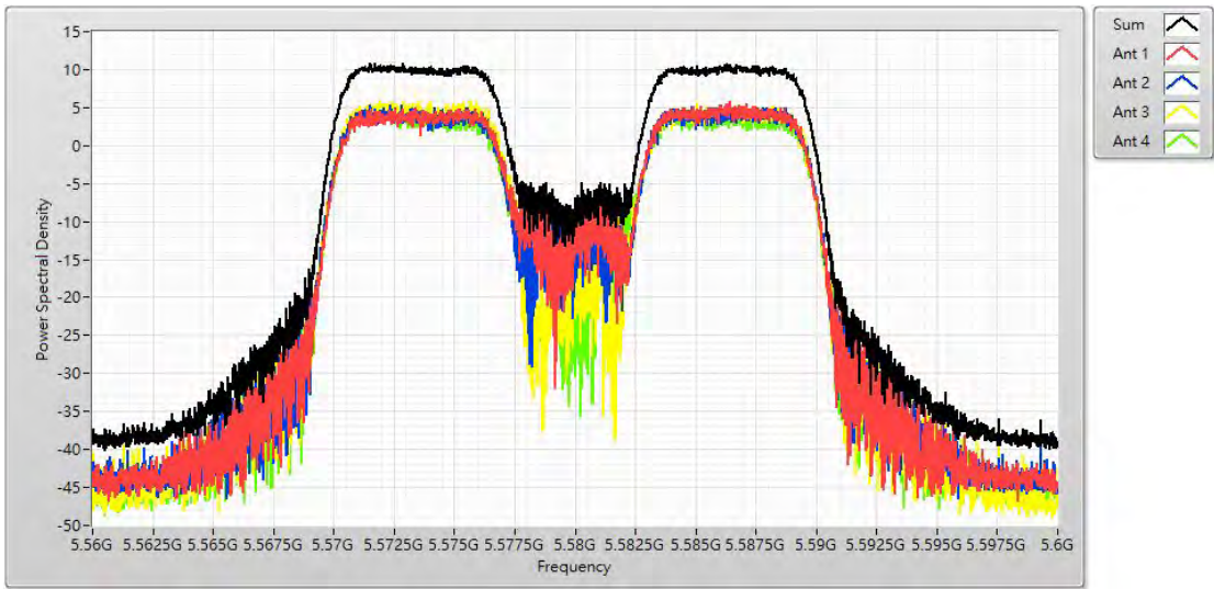
Channel 116 (5580MHz)
