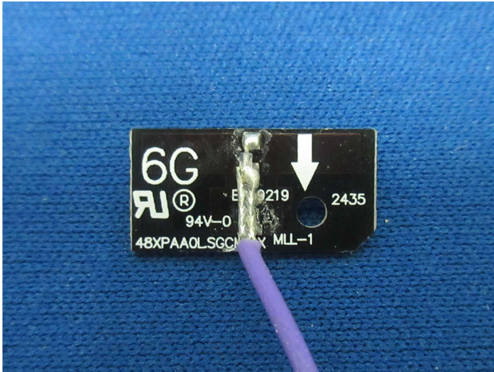
(18) EUT Photo (WiFi 6G Antenna)
