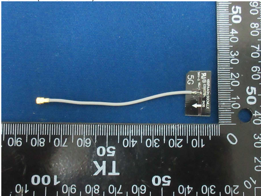
(30) EUT Photo (WiFi 5G Antenna)
