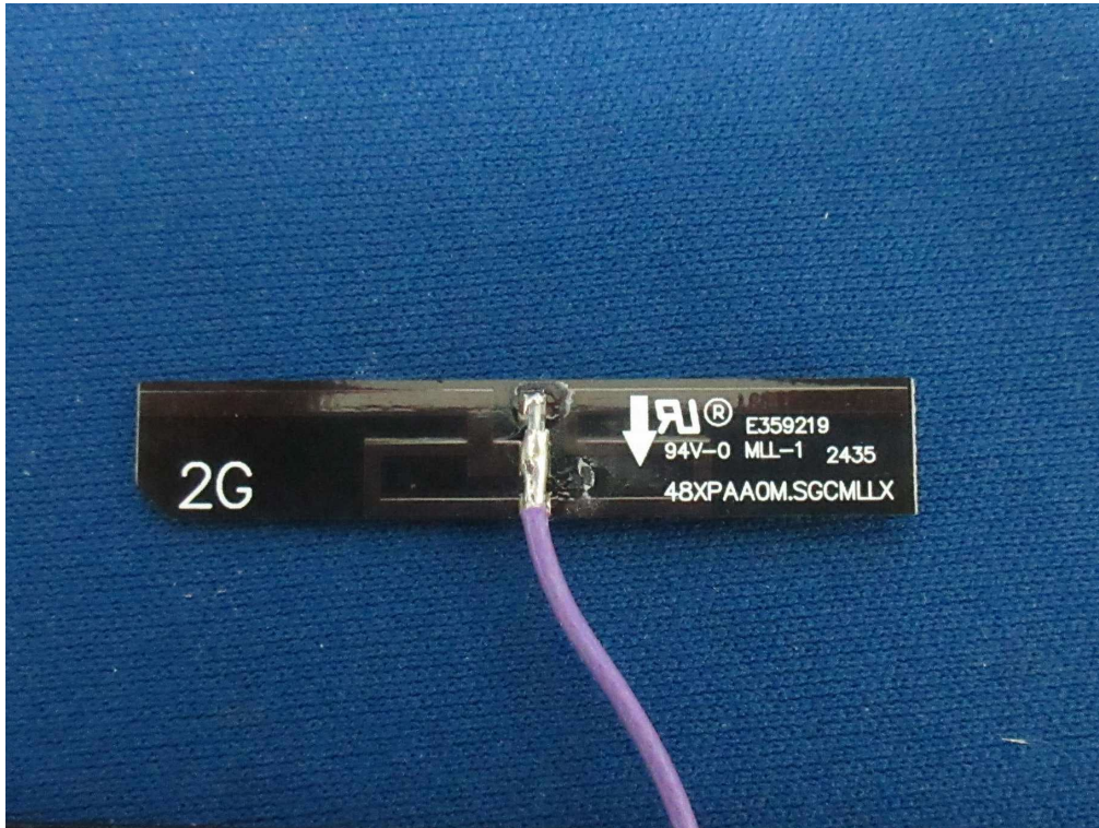
(48) EUT Photo (WiFi 2.4G Antenna)
