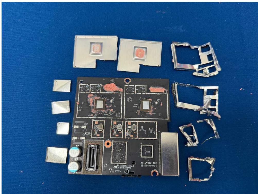
(90) EUT Photo
