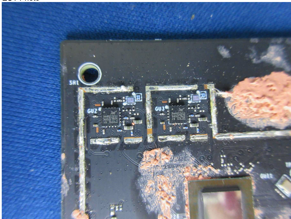
(90) EUT Photo
