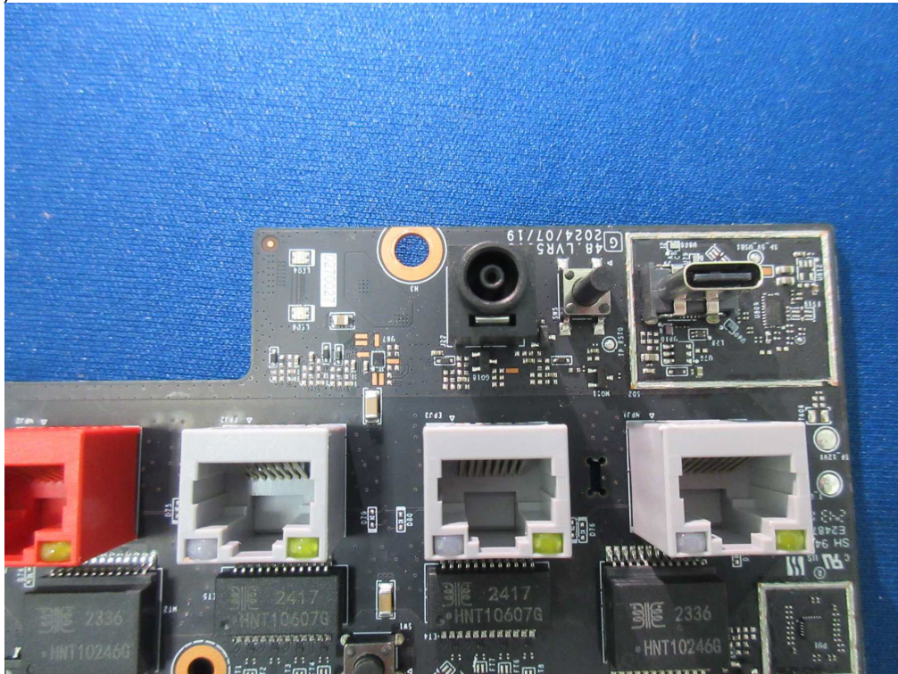
(112)EUT Photo
