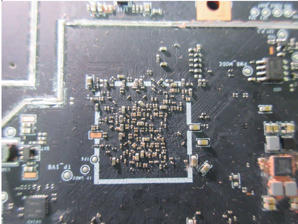
(134)EUT Photo
