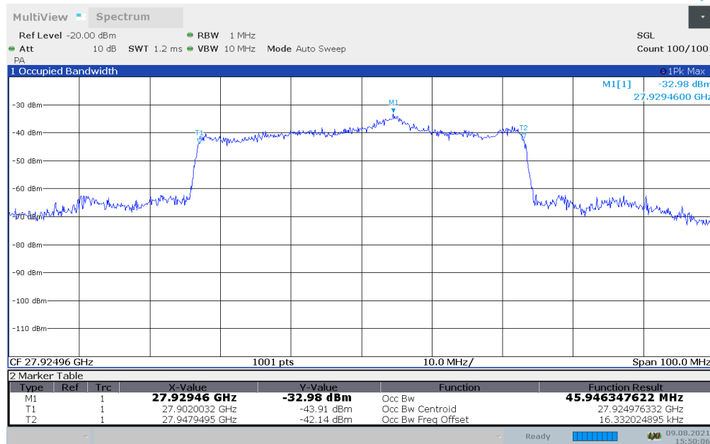
Plot 7-26. Occupied Bandwidth Plot - (n261 50MHz - QPSK - Mid Channel) – Relay Side – V Beam
