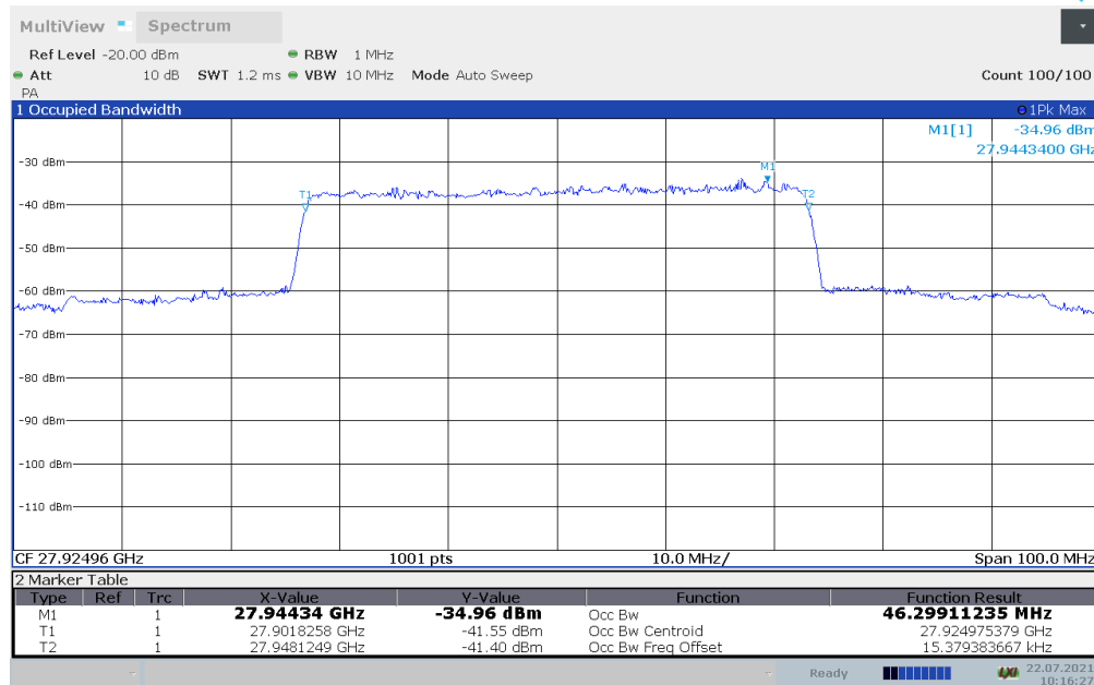
Plot 7-18. Occupied Bandwidth Plot - (n261 50MHz - QPSK - Mid Channel) – Relay Side – H Beam
