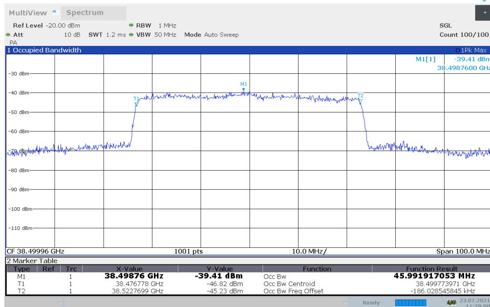
Plot 7-50. Occupied Bandwidth Plot - (n260 50MHz - QPSK - Mid Channel) – Relay Side – H Beam
