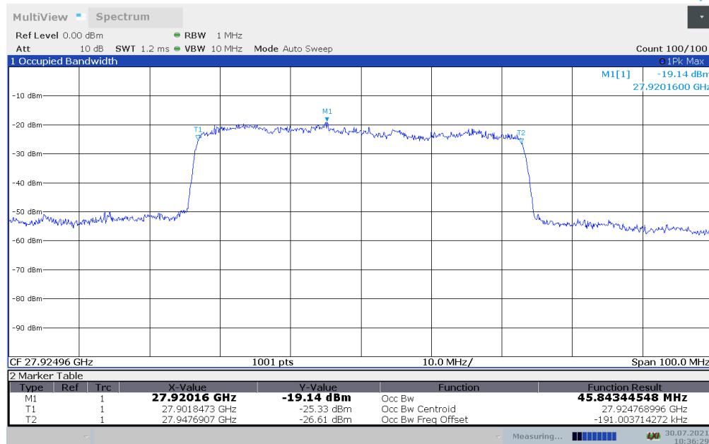
Plot 7-4. Occupied Bandwidth Plot - (n261 50MHz - 64QAM - Mid Channel) – Donor Side – H Beam
