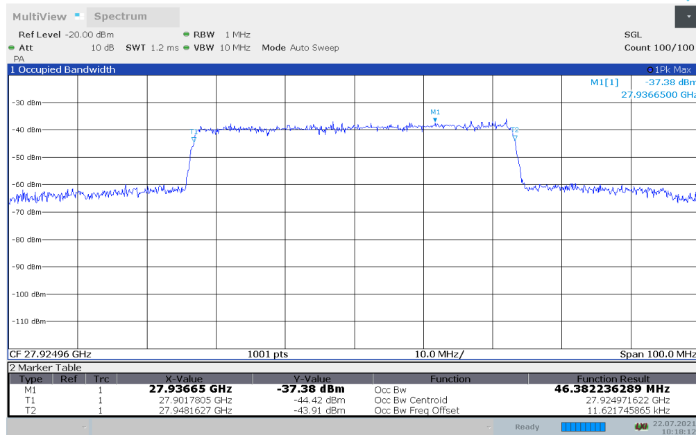
Plot 7-20. Occupied Bandwidth Plot - (n261 50MHz - 64QAM - Mid Channel) – Relay Side – H Beam
