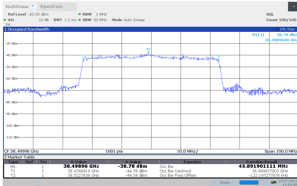
Plot 7-49. Occupied Bandwidth Plot - (n260 50MHz - \pi/2 BPSK - Mid Channel) – Relay Side – H Beam
