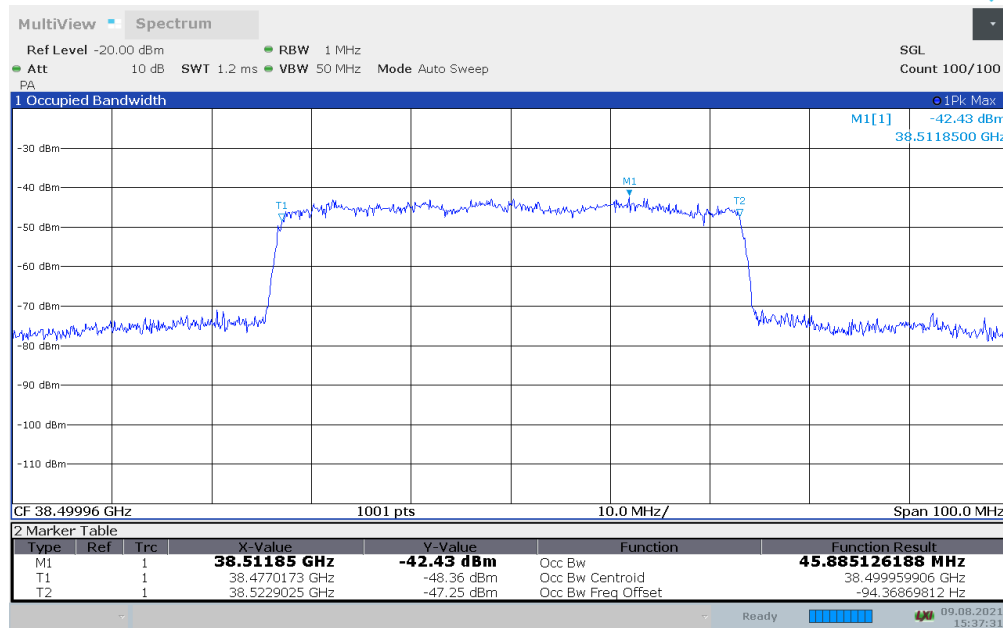
Plot 7-60. Occupied Bandwidth Plot - (n260 50MHz - 64QAM - Mid Channel) – Relay Side – V Beam
