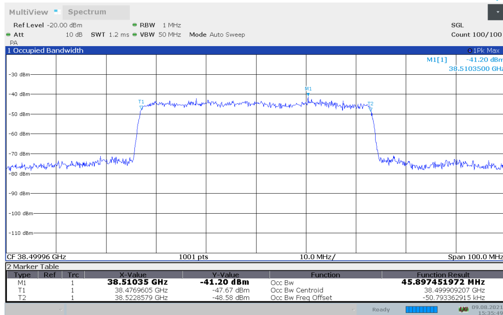
Plot 7-58. Occupied Bandwidth Plot - (n260 50MHz - QPSK - Mid Channel) – Relay Side – V Beam
