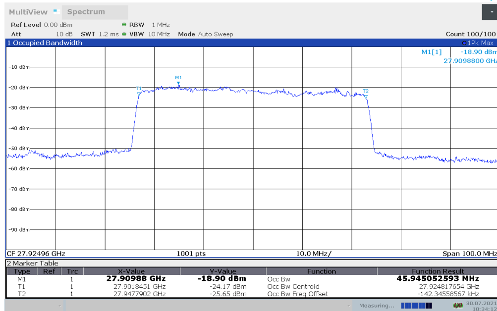
Plot 7-2. Occupied Bandwidth Plot - (n261 50MHz - QPSK - Mid Channel) – Donor Side – H Beam
