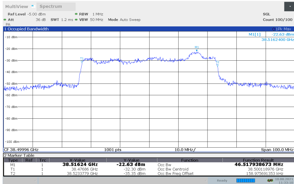
Plot 7-43. Occupied Bandwidth Plot - (n260 50MHz - 16QAM - Mid Channel) – Donor Side – V Beam
