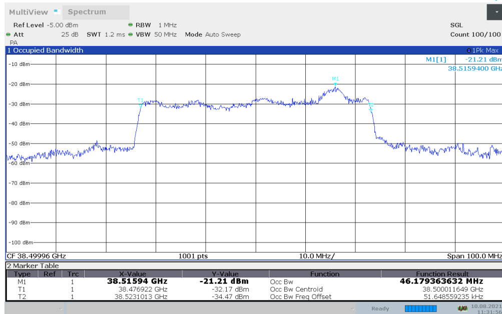
Plot 7-42. Occupied Bandwidth Plot - (n260 50MHz - QPSK - Mid Channel) – Donor Side – V Beam
