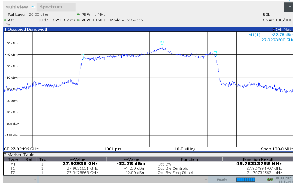
Plot 7-28. Occupied Bandwidth Plot - (n261 50MHz - 64QAM - Mid Channel) – Relay Side – V Beam
