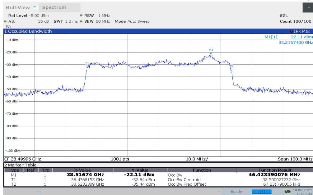
Plot 7-44. Occupied Bandwidth Plot - (n260 50MHz - 64QAM - Mid Channel) – Donor Side – V Beam
