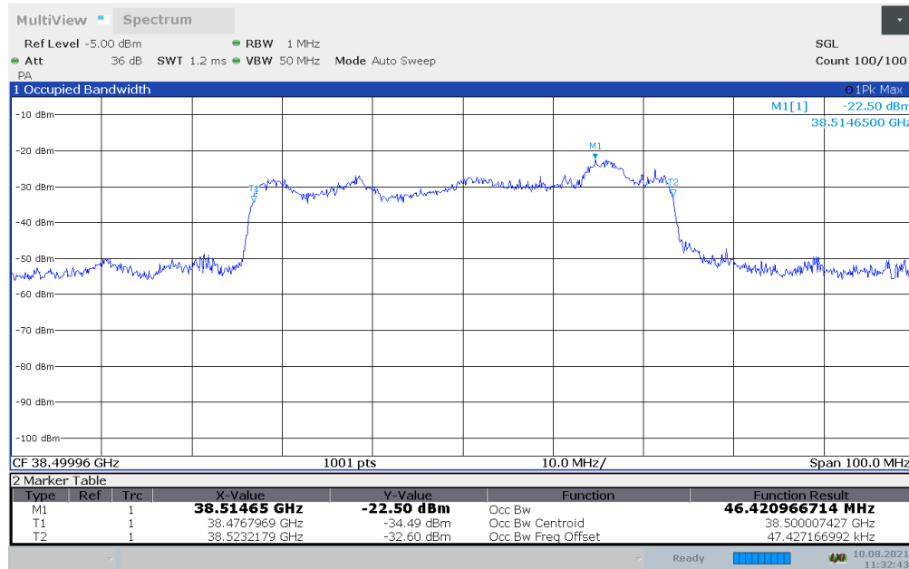
Plot 7-41. Occupied Bandwidth Plot - (n260 50MHz - \pi/2 BPSK - Mid Channel) – Donor Side – V Beam
