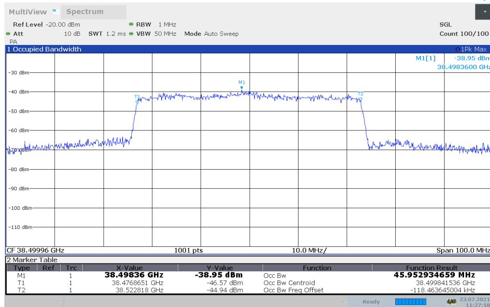
Plot 7-52. Occupied Bandwidth Plot - (n260 50MHz - 64QAM - Mid Channel) – Relay Side – H Beam
