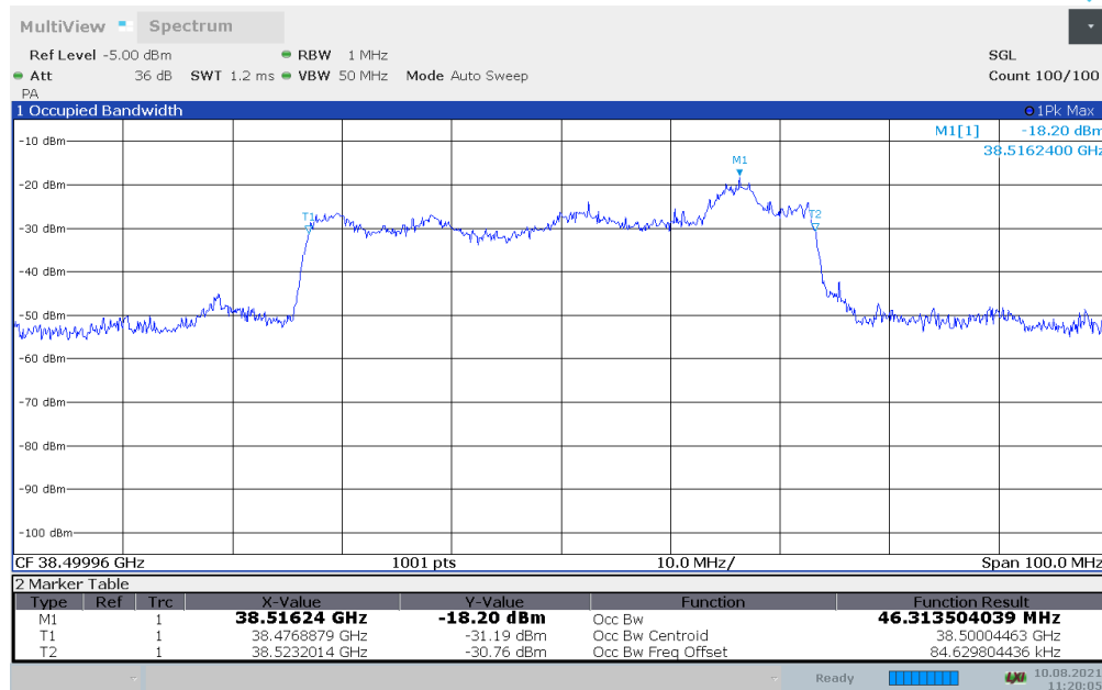
Plot 7-34. Occupied Bandwidth Plot - (n260 50MHz - QPSK - Mid Channel) – Donor Side – H Beam
