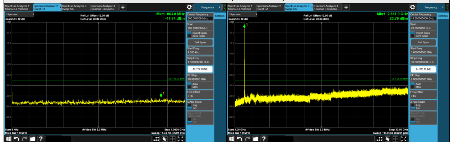
Channel 529998 (2649.99 MHz)
