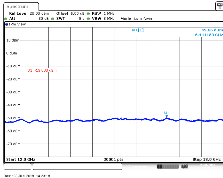
BAND 12_10MHz_64QAM_23060_1RB#0
