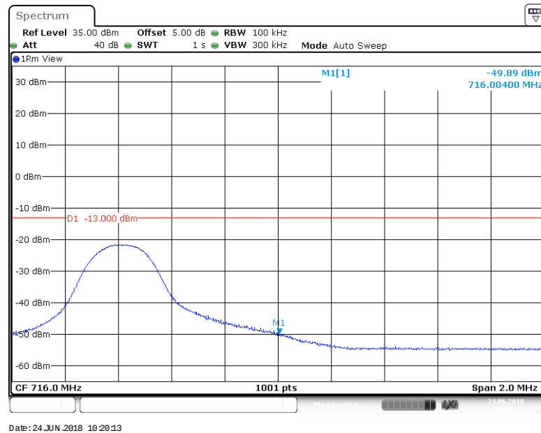
BAND 12_10MHz_64QAM_23130_1RB#49
