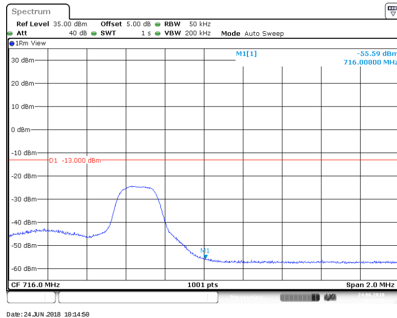
BAND 12_5MHz_64QAM_23155_1RB#24
