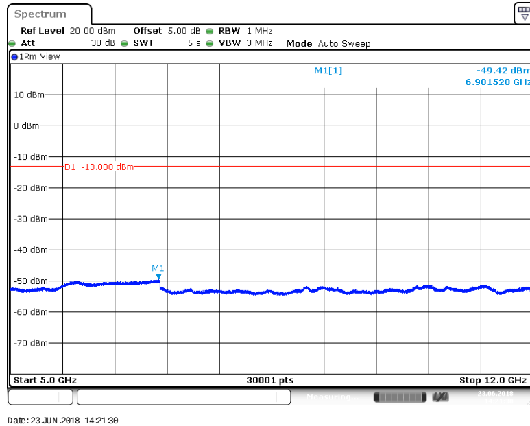
BAND 12_10MHz_16QAM_23095_1RB#0
