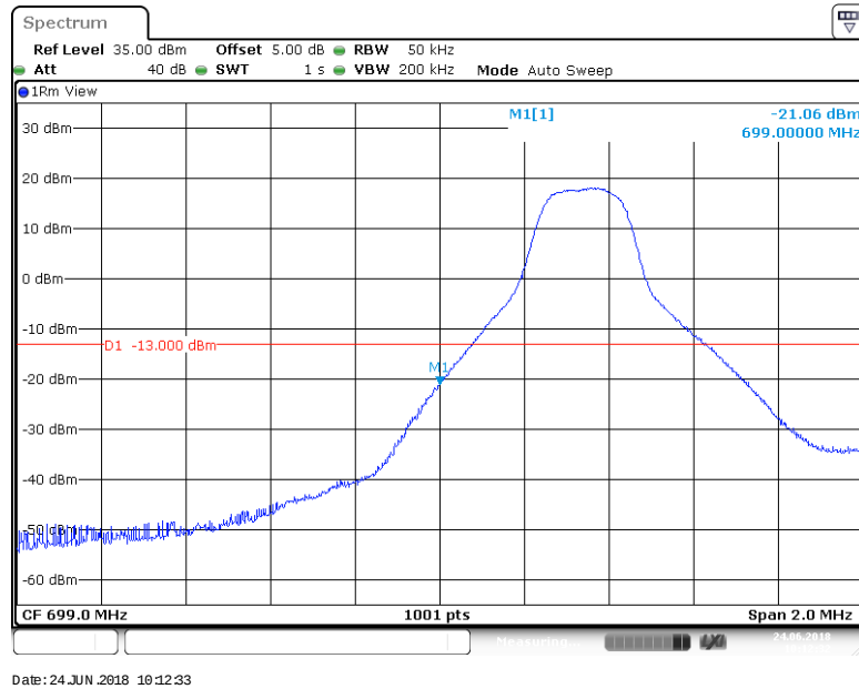
BAND 12_5MHz_64QAM_23035_1RB#24
