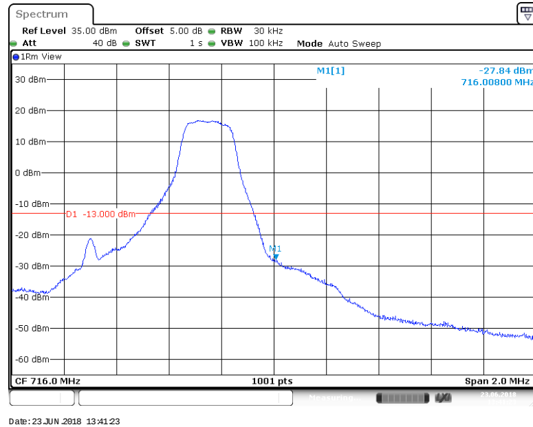
BAND 12_1.4MHz_QPSK_23173_6RB#0
