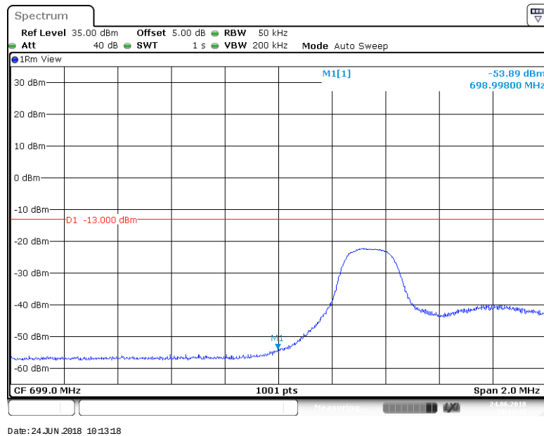
BAND 12_5MHz_64QAM_23035_25RB#0
