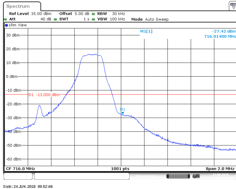
BAND 12_1.4MHz_64QAM_23173_6RB#0
