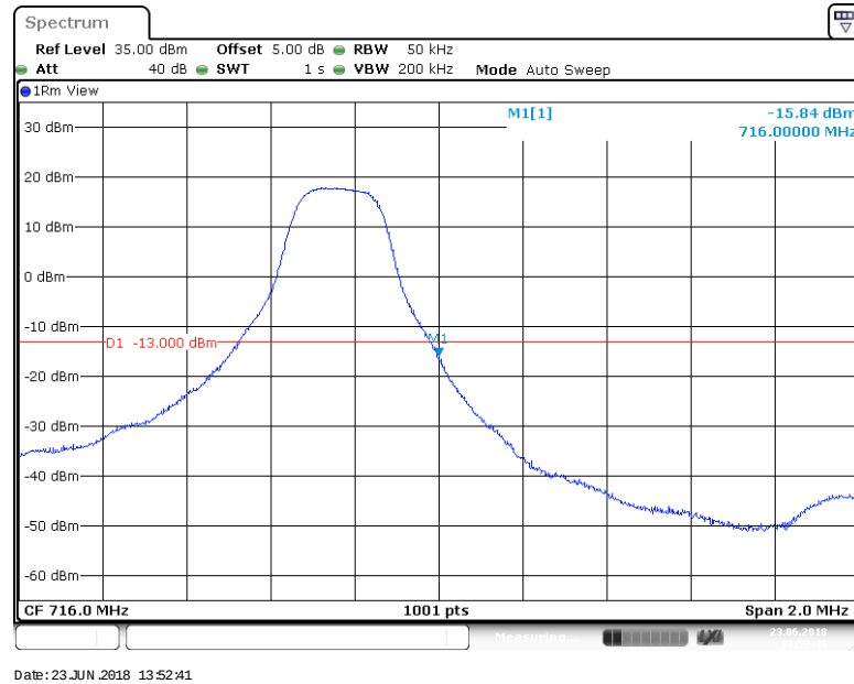
BAND 12_3MHz_16QAM_23165_15RB#0
