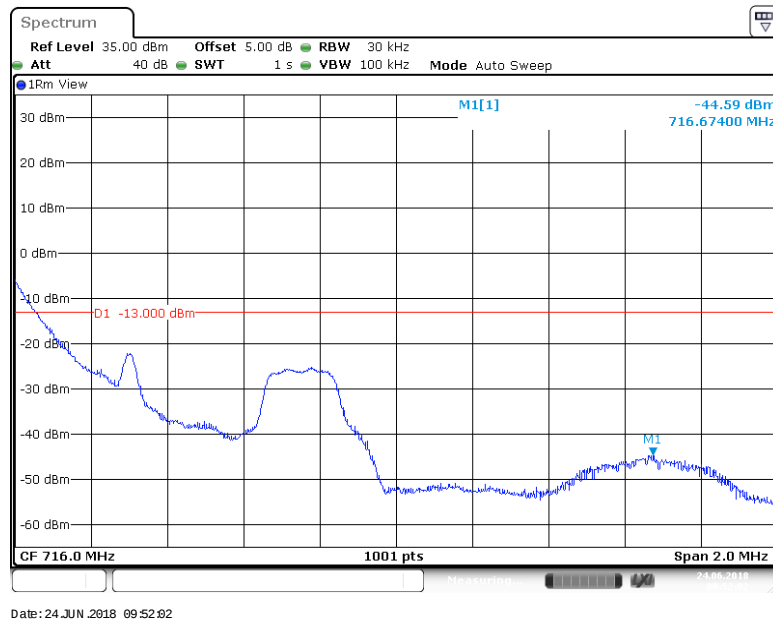
BAND 12_1.4MHz_64QAM_23173_1RB#5
