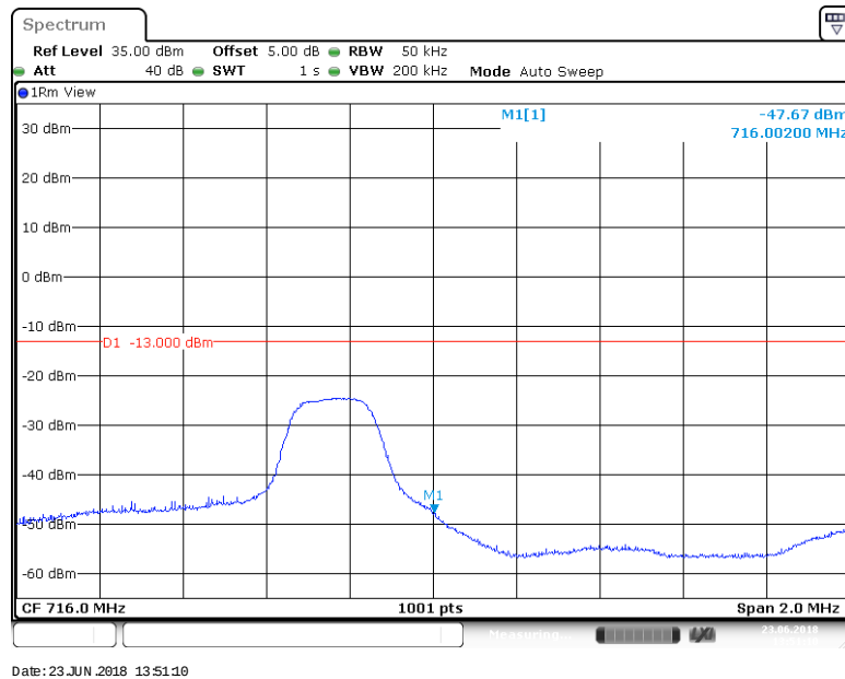
BAND 12_3MHz_16QAM_23165_1RB#14
