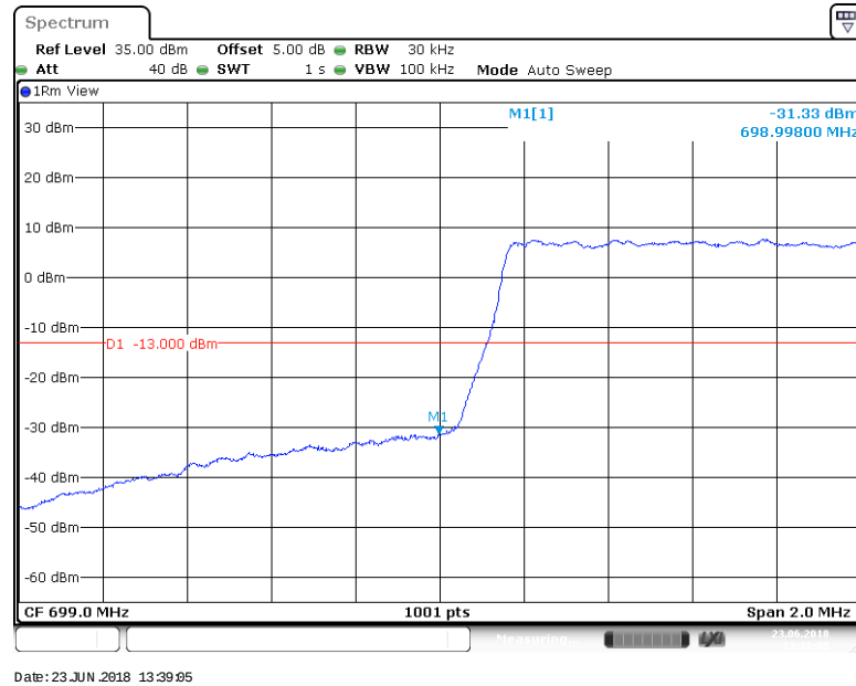
BAND 12_1.4MHz_16QAM_23173_1RB#0
