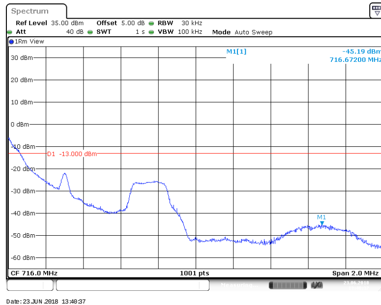
BAND 12_1.4MHz_16QAM_23173_1RB#5
