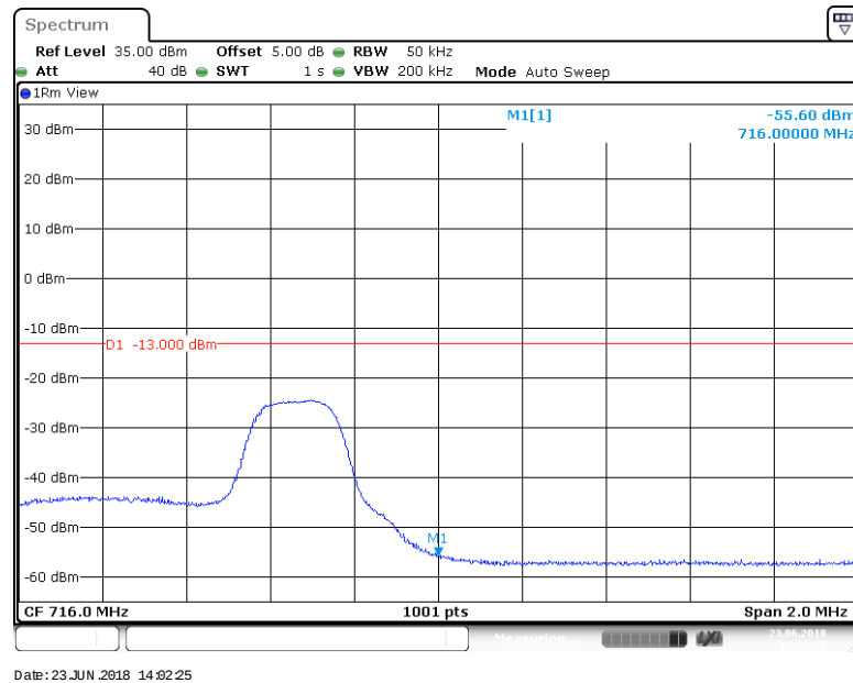
BAND 12_5MHz_16QAM_23155_1RB#24
