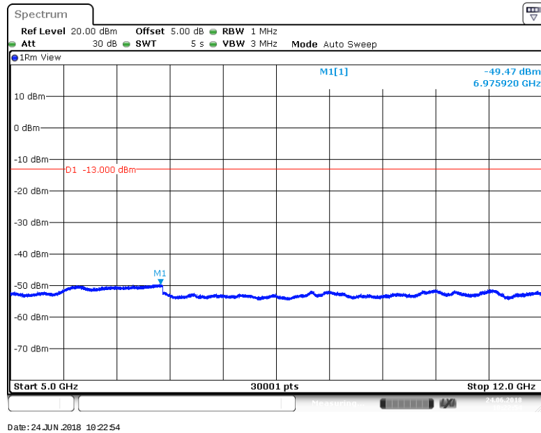
BAND 12_10MHz_64QAM_23060_1RB#0
