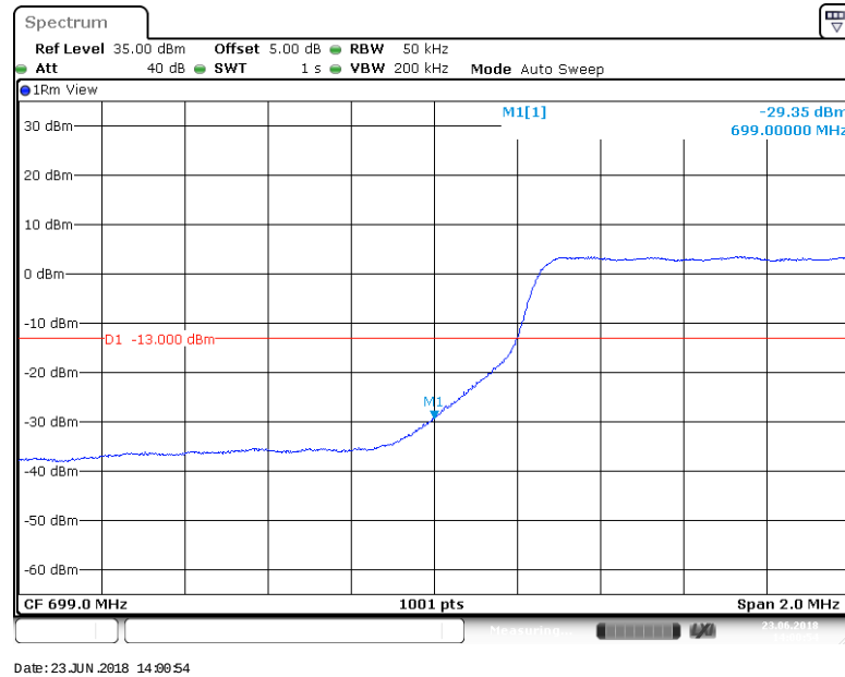
BAND 12_5MHz_16QAM_23155_1RB#0
