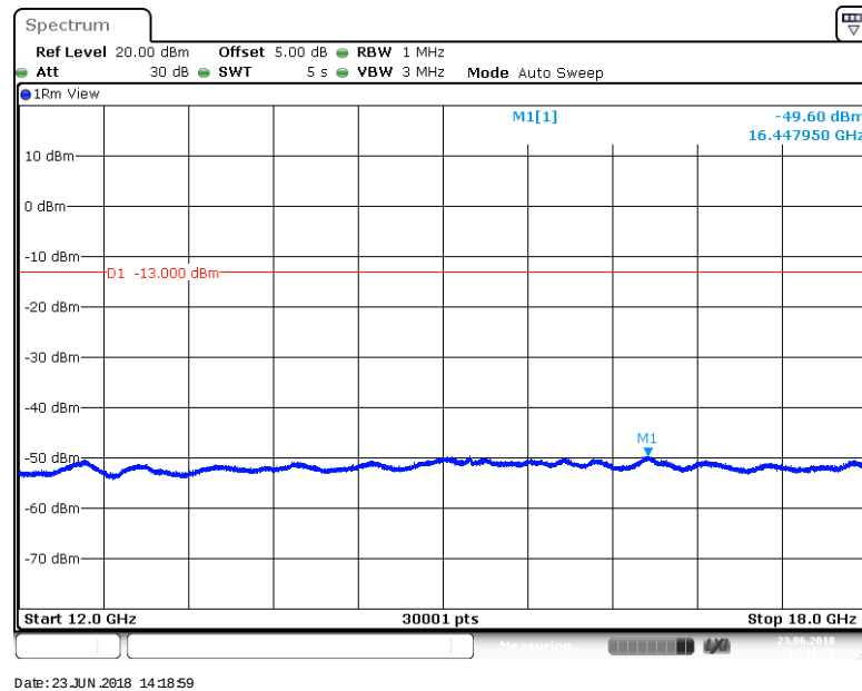
BAND 12_10MHz_16QAM_23095_1RB#0
