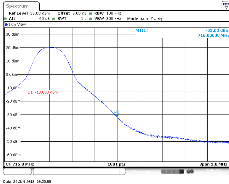
BAND 12_10MHz_64QAM_23130_50RB#0
