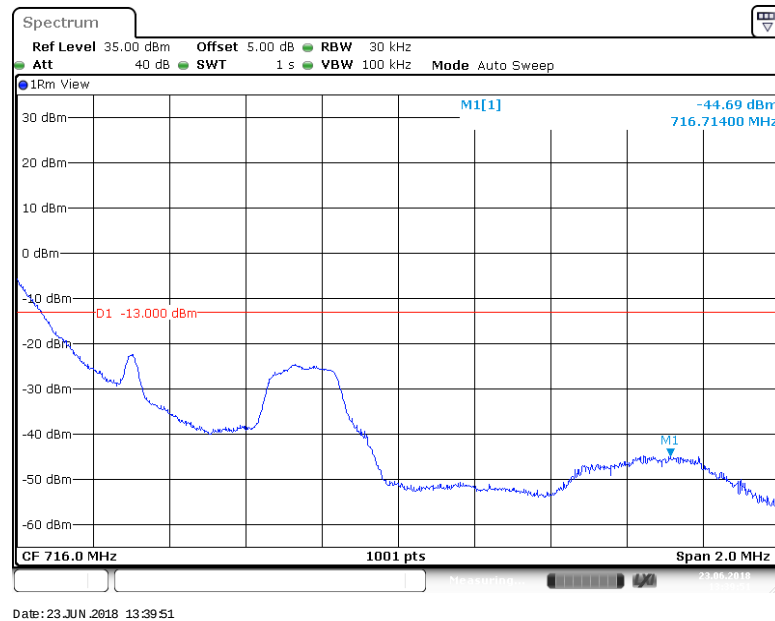
BAND 12_1.4MHz_QPSK_23173_1RB#5
