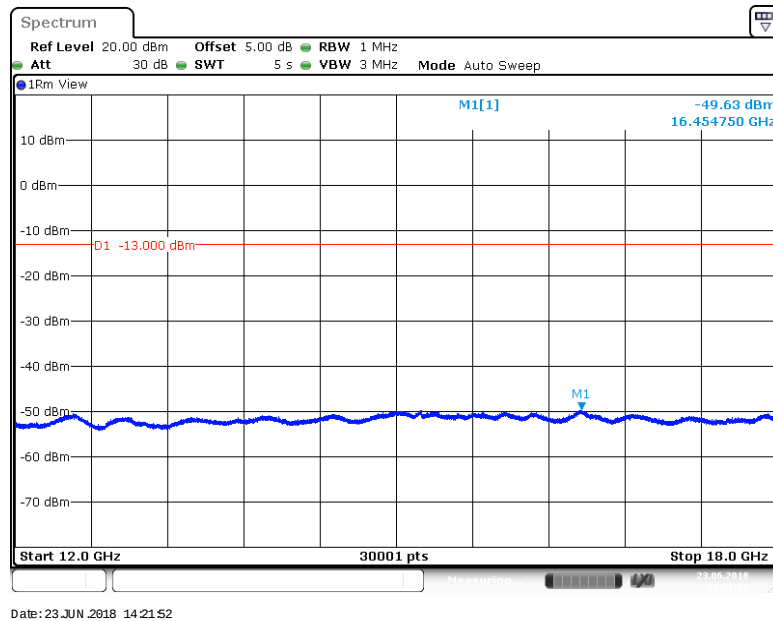
BAND 12_10MHz_16QAM_23130_1RB#0
