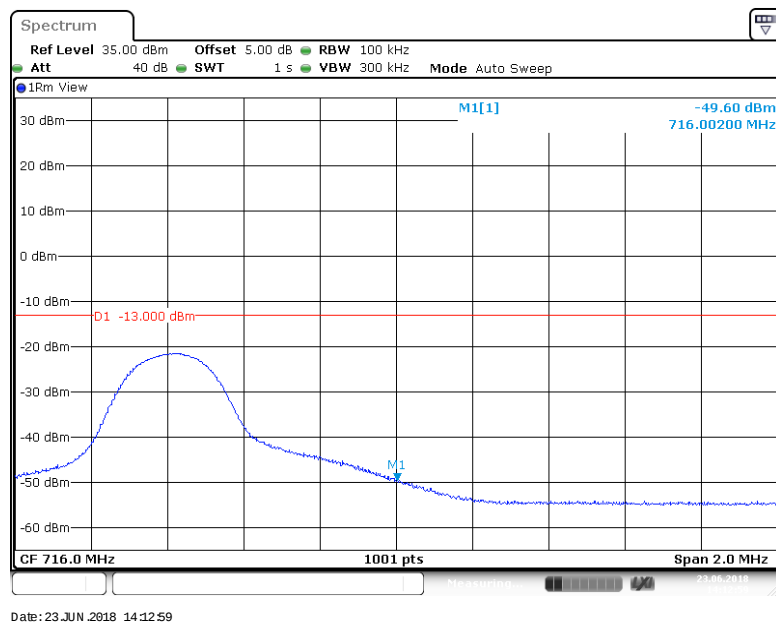
BAND 12_10MHz_16QAM_23130_1RB#49
