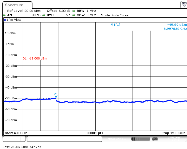
BAND 12_10MHz_QPSK_23060_1RB#0
