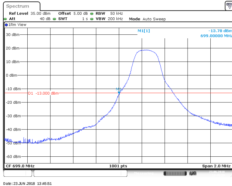
BAND 12_3MHz_QPSK_23025_1RB#14
