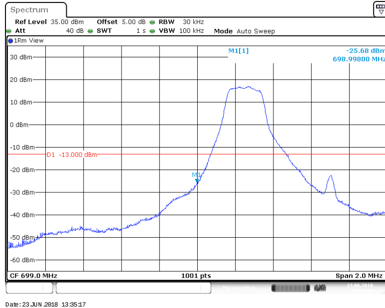
BAND 12_1.4MHz_QPSK_23017_1RB#5
