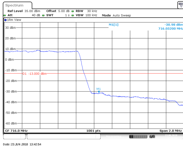
BAND 12_1.4MHz_64QAM_23017_1RB#0
