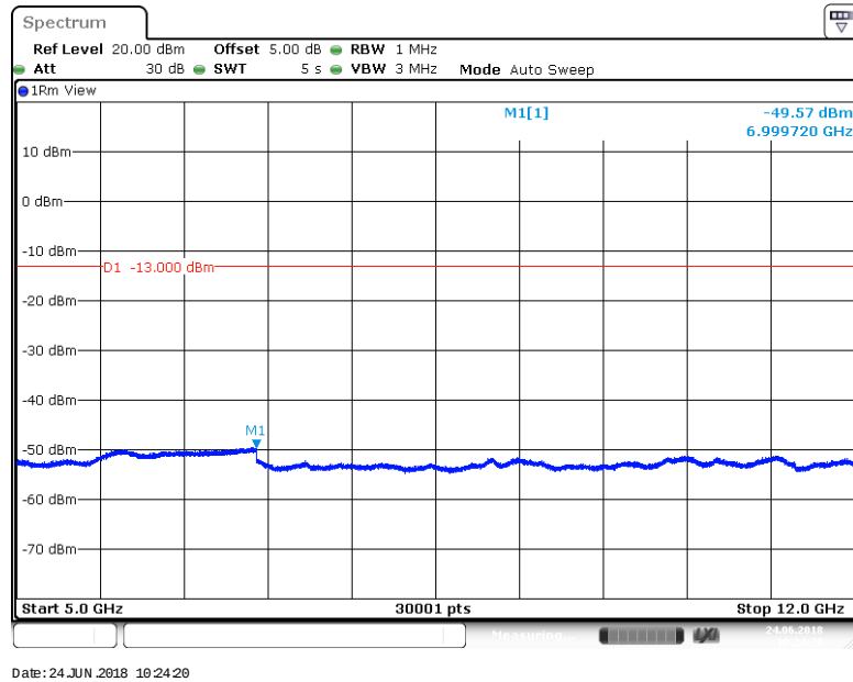
BAND 12_10MHz_64QAM_23095_1RB#0
