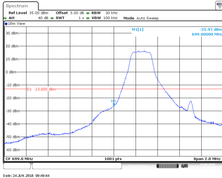
BAND 12_1.4MHz_64QAM_23017_1RB#5
