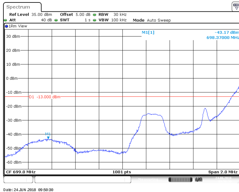
BAND 12_1.4MHz_64QAM_23017_6RB#0
