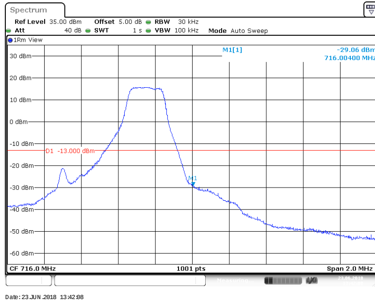
BAND 12_1.4MHz_16QAM_23173_6RB#0
