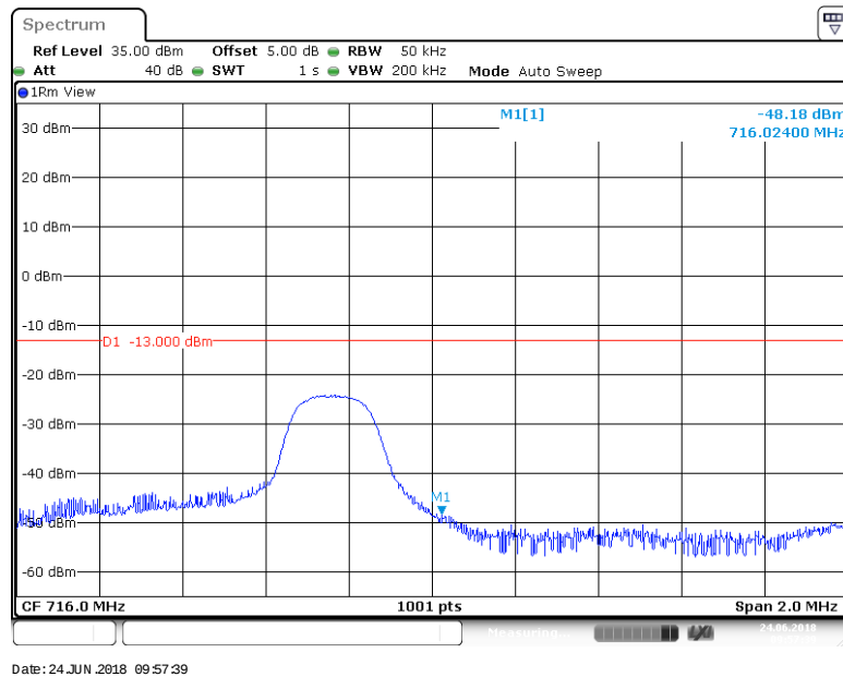
BAND 12_3MHz_64QAM_23165_1RB#14
