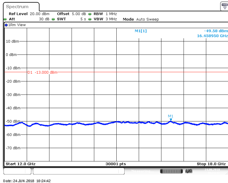
BAND 12_10MHz_64QAM_23130_1RB#0
