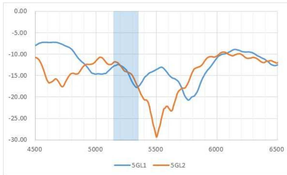
Return Loss
