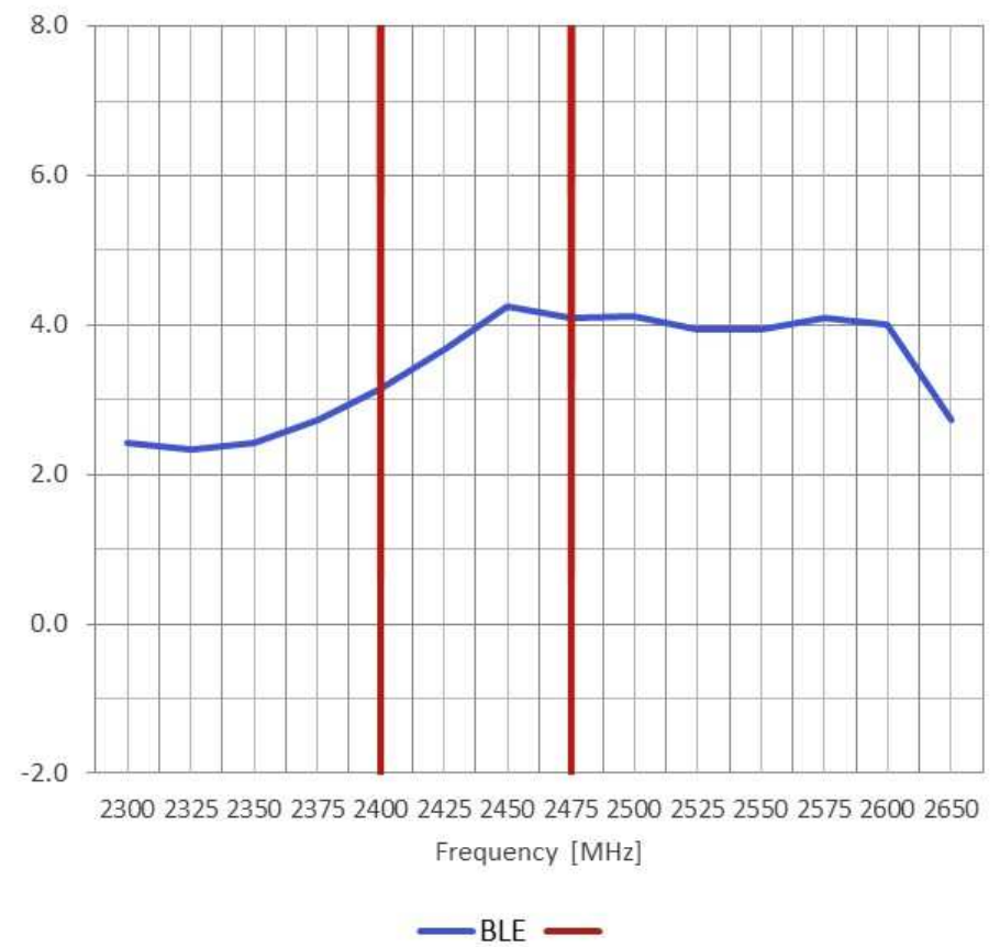
Peak Gain
