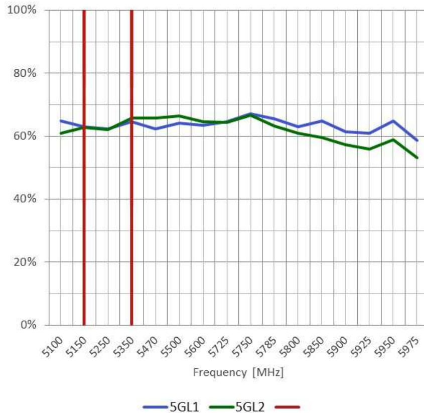
Efficiency
