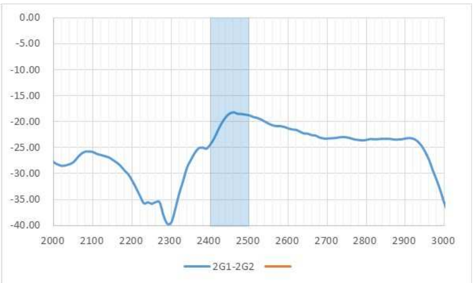
Isolation
