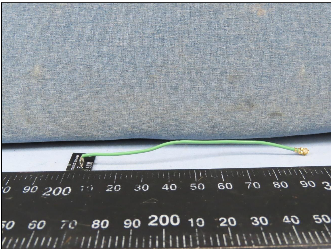
WiFi 6 Antenna
