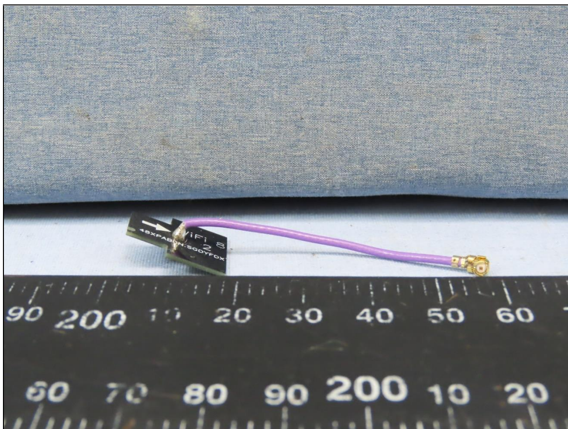
WiFi 8 Antenna
