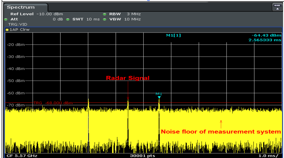
Radar Signal 5 (Single Burst)
