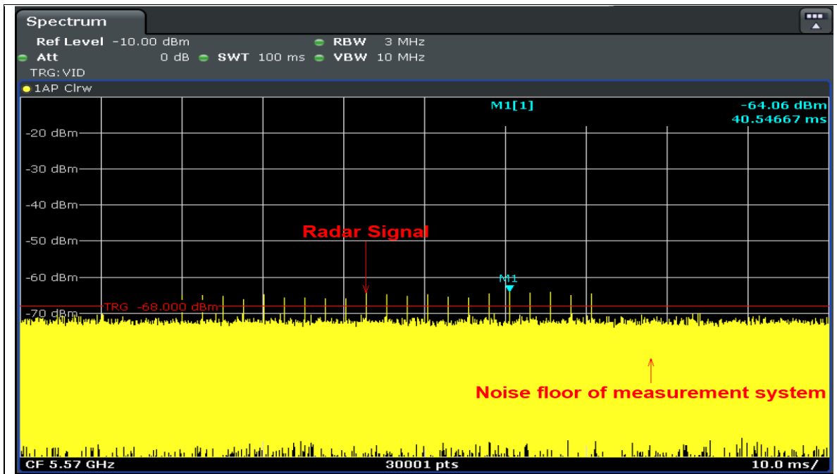
Radar Signal 1 (Test B)
