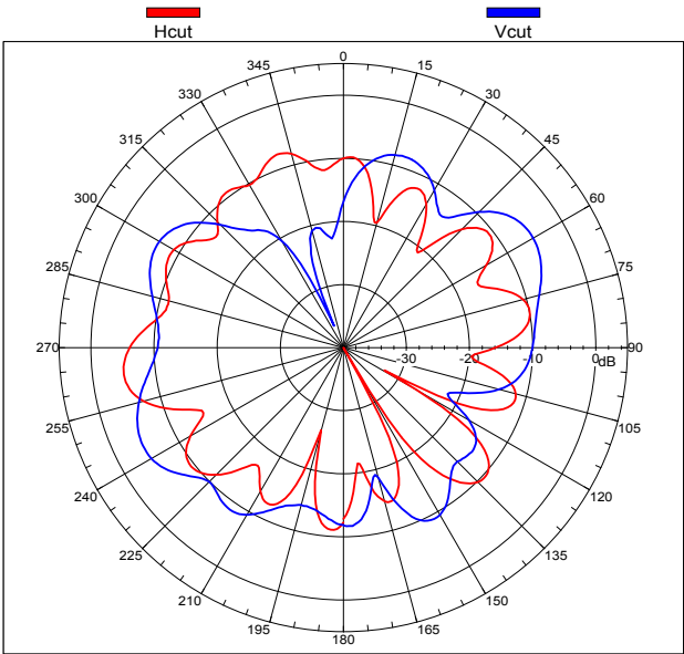
Far-field amplitude of XZ-2.45 H&V
