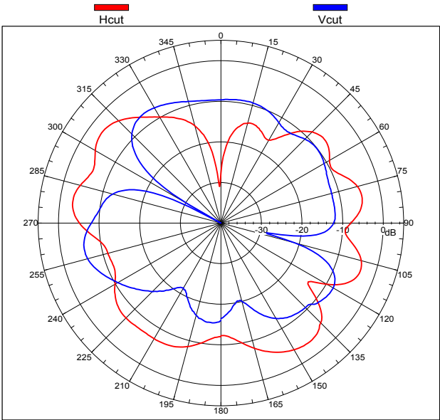
Far-field amplitude of YZ-2.45 H&V
