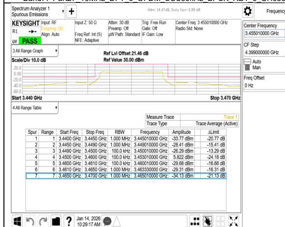
Band77-Part27 10MHz DFT s OFDM SCS30kHz BPSK RB24_0 CH630334
