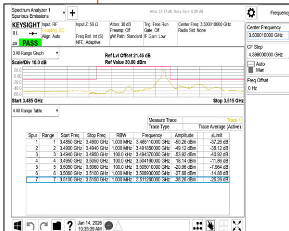
Band77-Part27 10MHz DFT s OFDM SCS30kHz BPSK RB1 23 CH633334
