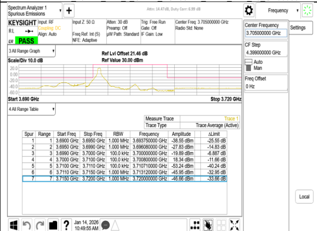
Band77-Part27 10MHz DFT s OFDM SCS30kHz BPSK RB1 0 CH647000
