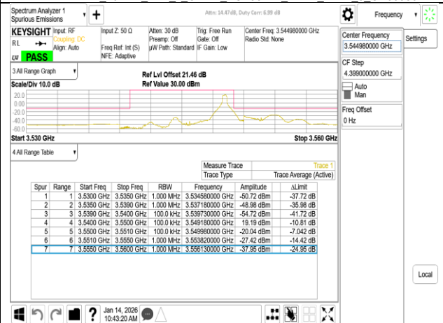
Band77-Part27 10MHz DFT s OFDM SCS30kHz BPSK RB1 23 CH636332
