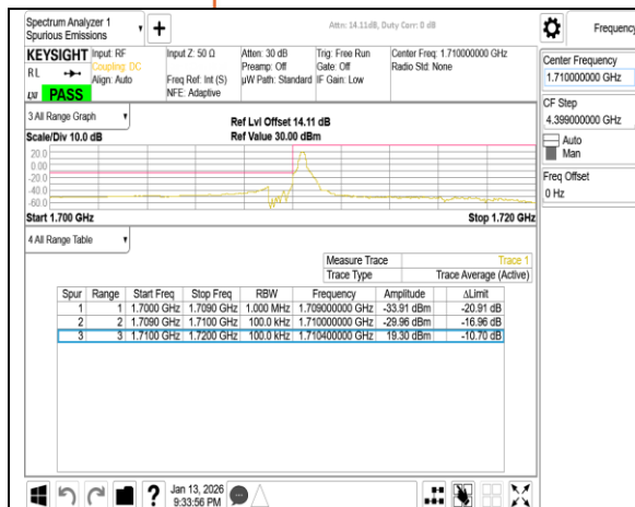
Band66 10MHz CP OFDM SCS15kHz QPSK RB1_0 CH343000
