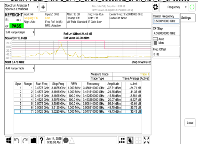
Band77-Part27 15MHz DFT s OFDM SCS30kHz BPSK RB1_0 CH633334
