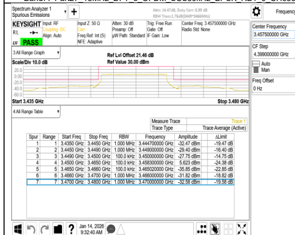
Band77-Part27 15MHz DFT s OFDM SCS30kHz BPSK RB36_0 CH630500
