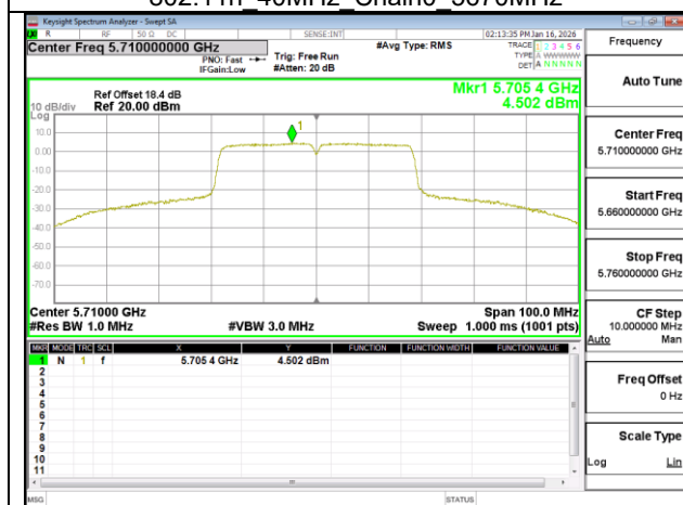
802.11n 40MHz Chain0 5710MHz UNII 2C
