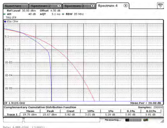
LTE Band 25_16-QAM_1912.5M_5M_1RB0
