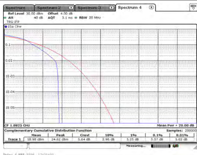
LTE Band 25_16-QAM_1882.5M_15M_1RB0
