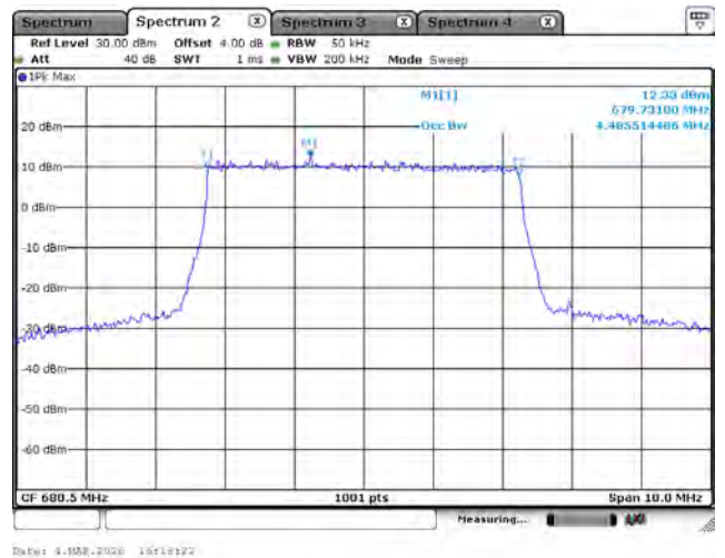
LTE Band 71_QPSK_680.5M_5M_FRB
