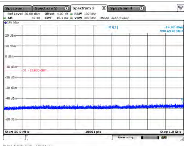
LTE Band 66_QPSK_1777.5M_5M_1RB0_Below 1GHz
