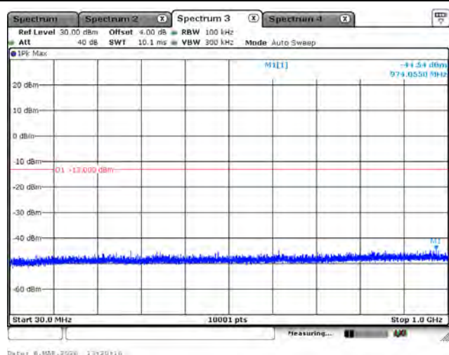
LTE Band 66_QPSK_1745M_5M_1RB0_Below 1GHz
