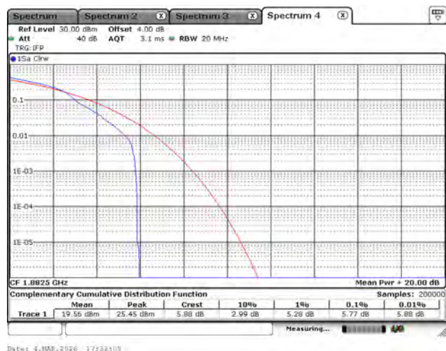
LTE Band 25_16-QAM_1882.5M_5M_1RB0
