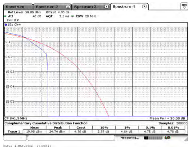
LTE Band 26 (Part 22)_16-QAM_841.5M_15M_1RB0
