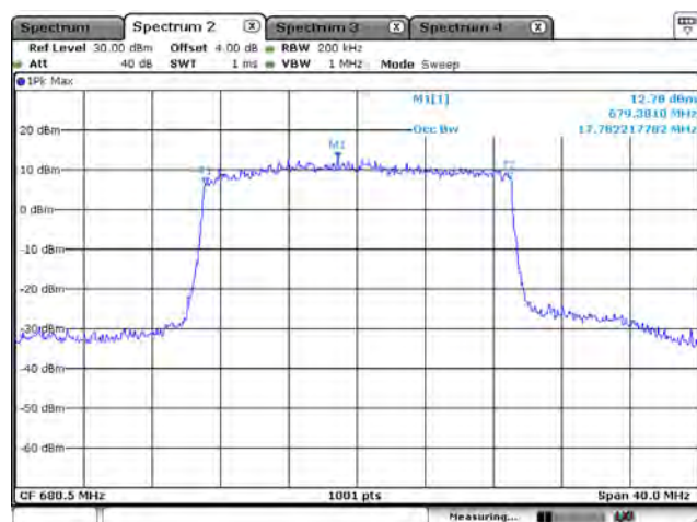
LTE Band 71_QPSK_680.5M_20M_FRB
