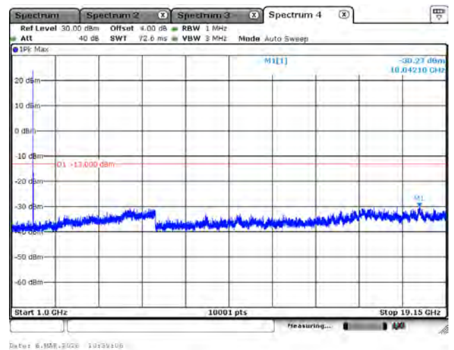
LTE Band 25_QPSK_1912.5M_5M_1RB0_Above 1GHz
