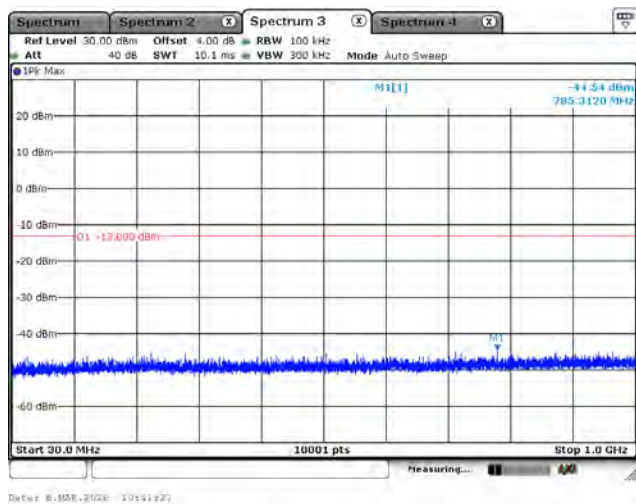
LTE Band 25_QPSK_1912.5M_5M_1RB0_Below 1GHz
