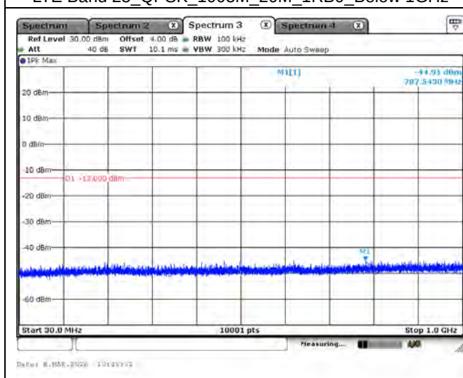
LTE Band 25_QPSK_1905M_20M_1RB0_Below 1GHz
