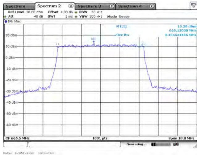
LTE Band 71_QPSK_665.5M_5M_FRB
