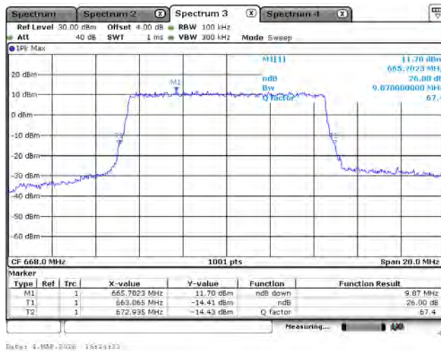
LTE Band 71_QPSK_668M_10M_FRB
