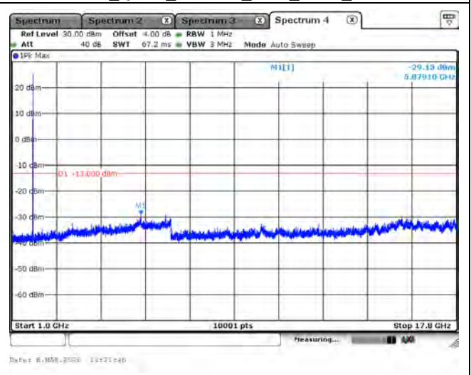
LTE Band 66_QPSK_1779.3M_1.4M_1RB0_Above 1GHz
