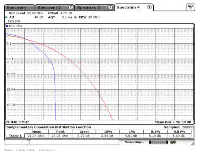
LTE Band 26 (Part 22)_16-QAM_848.3M_1.4M_1RB0
