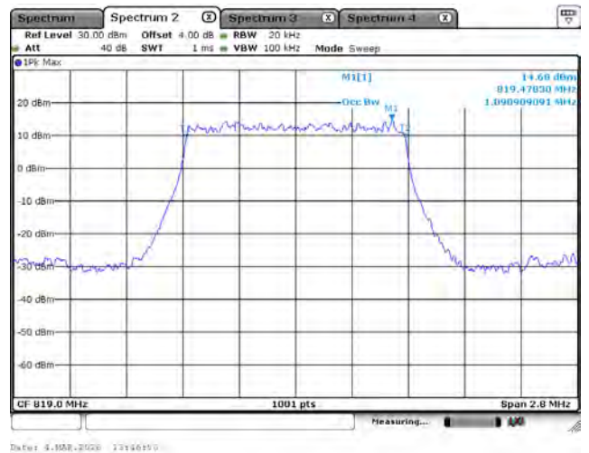
LTE Band 26 (Part 90)_QPSK_819M_1.4M_FRB
