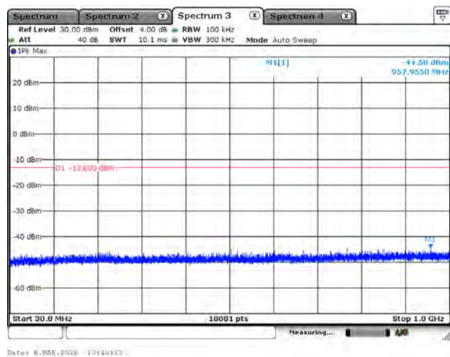
LTE Band 25_QPSK_1882.5M_3M_1RB0_Below 1GHz
