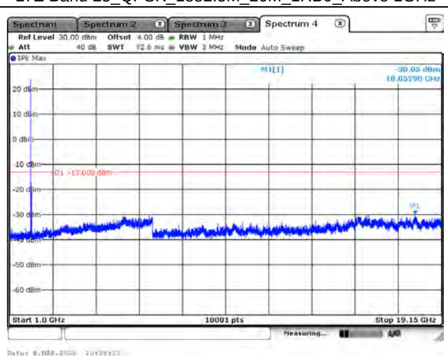
LTE Band 25_QPSK_1905M_20M_1RB0_Above 1GHz
