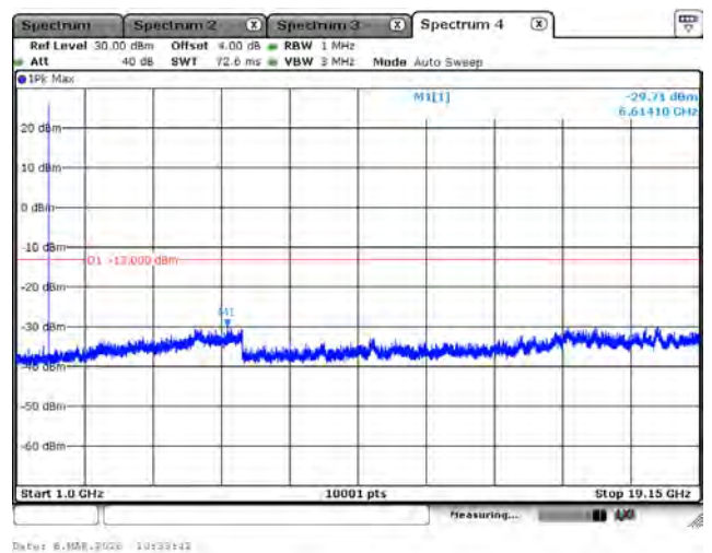
LTE Band 25_QPSK_1882.5M_3M_1RB0_Above 1GHz
