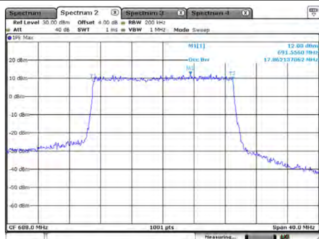
LTE Band 71_QPSK_688M_20M_FRB
