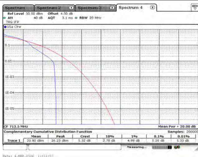
LTE Band 12_16-QAM_713.5M_5M_1RB0
