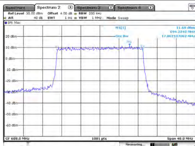
LTE Band 71_16-QAM_688M_20M_FRB
