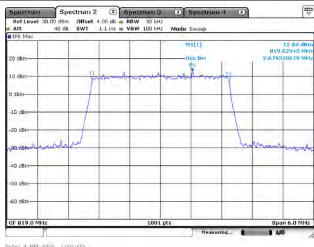
LTE Band 26 (Part 90)_16-QAM_819M_3M_FRB
