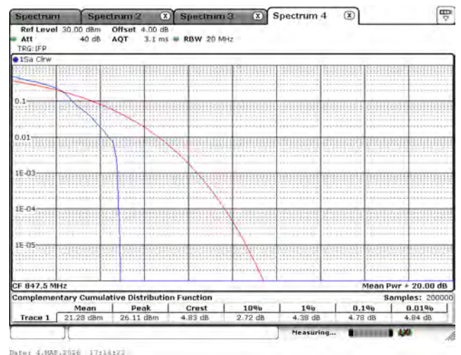
LTE Band 26 (Part 22)_16-QAM_847.5M_3M_1RB0
