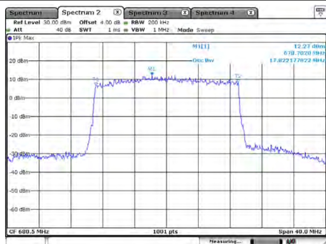
LTE Band 71_16-QAM_680.5M_20M_FRB
