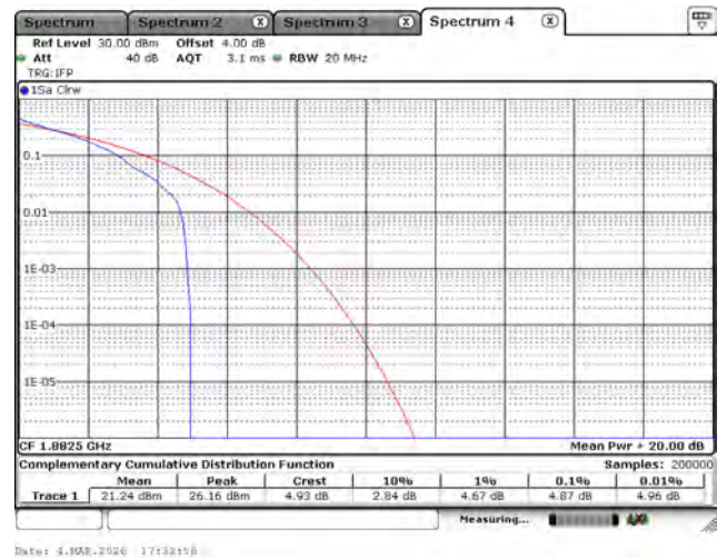
LTE Band 25_QPSK_1882.5M_3M_1RB0
