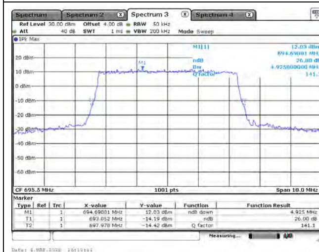
LTE Band 71_QPSK_695.5M_5M_FRB
