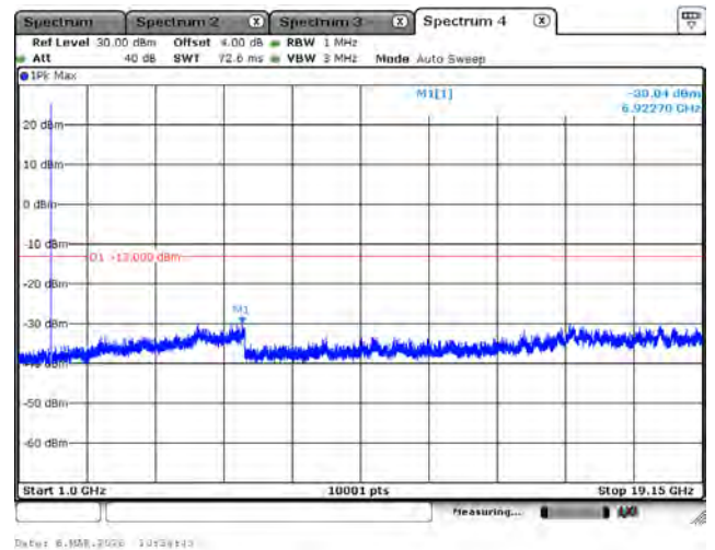
LTE Band 25_QPSK_1882.5M_5M_1RB0_Above 1GHz
