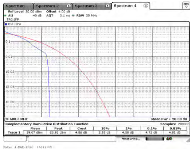
LTE Band 71_QPSK_680.5M_20M_1RB0
