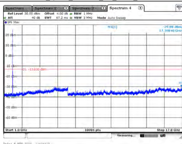
LTE Band 66_QPSK_1777.5M_5M_1RB0_Above 1GHz
