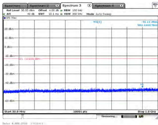
LTE Band 66_QPSK_1745M_3M_1RB0_Below 1GHz
