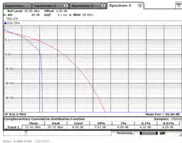
LTE Band 26 (Part 90)_QPSK_816.5M_5M_1RB0
