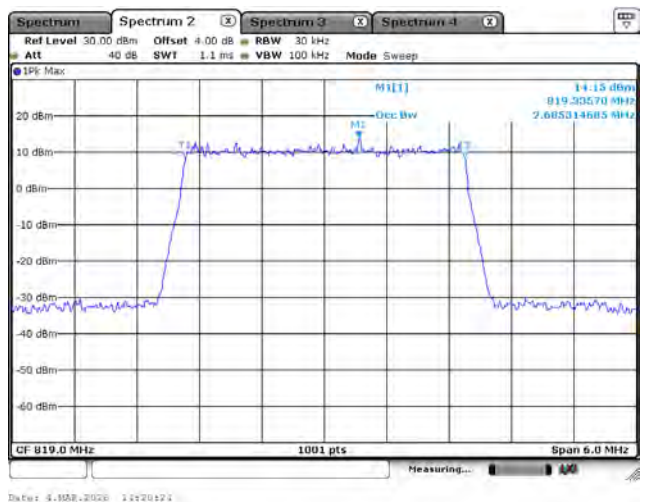
LTE Band 26 (Part 90)_QPSK_819M_3M_FRB
