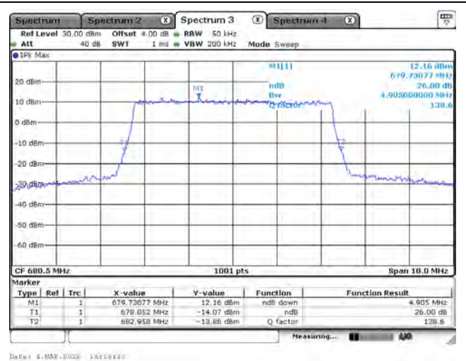
LTE Band 71_QPSK_680.5M_5M_FRB
