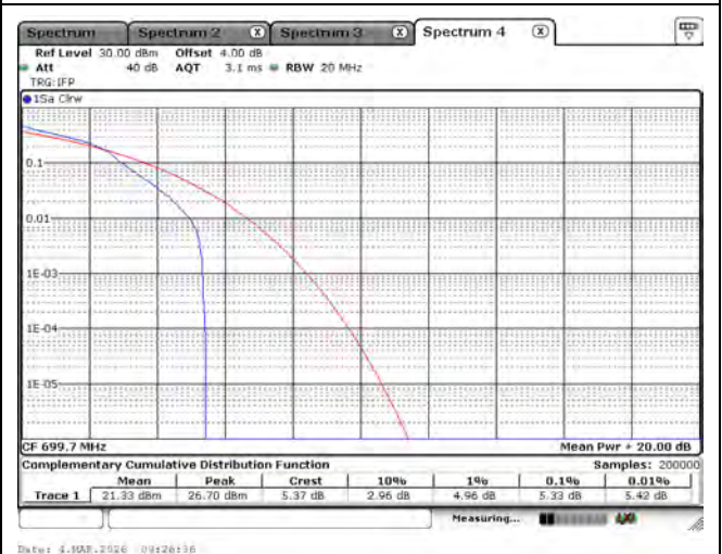
LTE Band 12_16-QAM_699.7M_1.4M_1RB0
