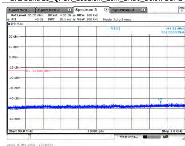
LTE Band 25_QPSK_1905M_20M_1RB0_Below 1GHz
