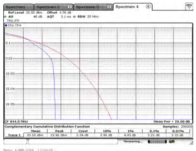
LTE Band 26 (Part 22)_16-QAM_844M_10M_1RB0
