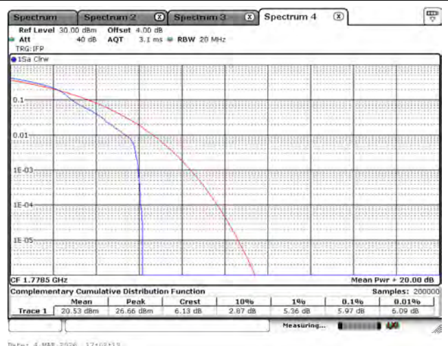
LTE Band 66_16-QAM_1778.5M_3M_1RB0
