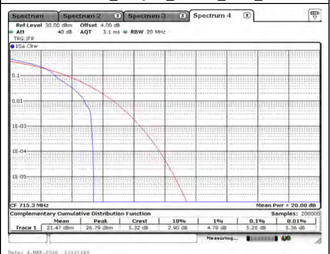
LTE Band 12_16-QAM_715.3M_1.4M_1RB0
