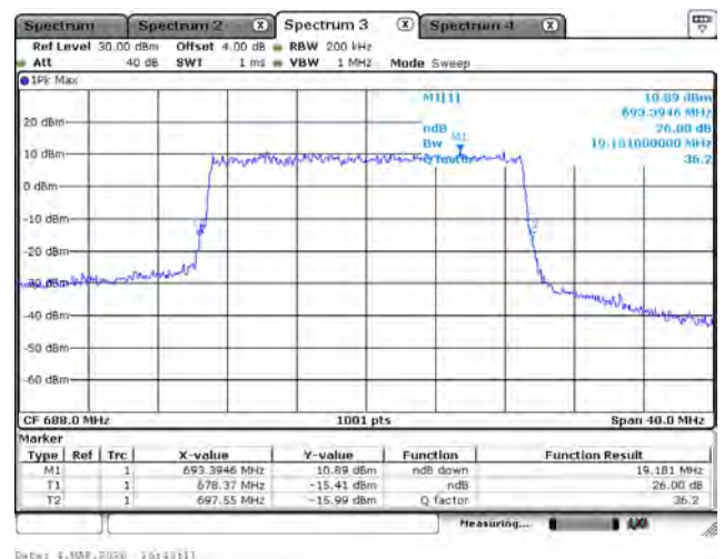
LTE Band 71_16-QAM_688M_20M_FRB
