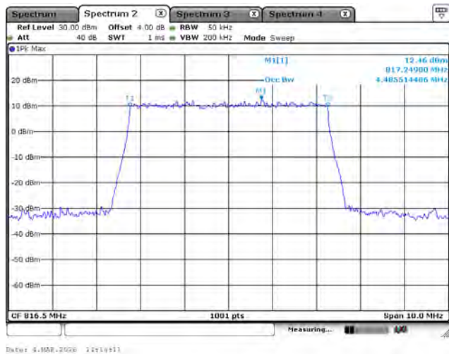
LTE Band 26 (Part 90)_QPSK_816.5M_5M_FRB
