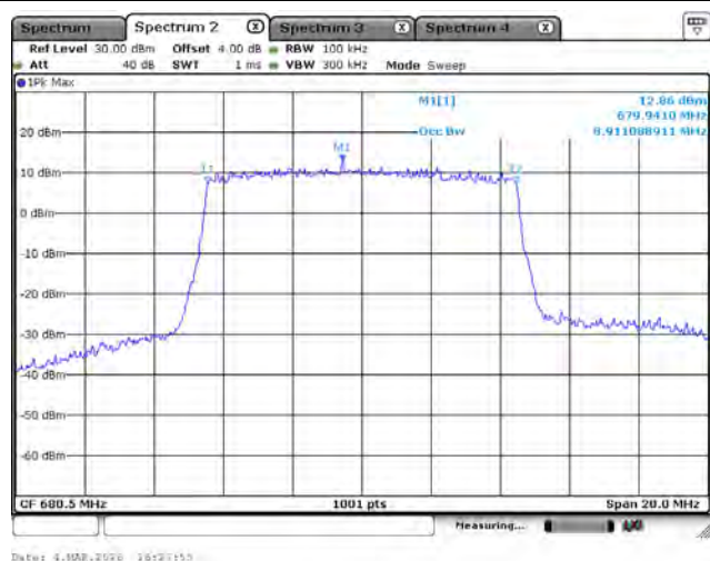
LTE Band 71_16-QAM_680.5M_10M_FRB
