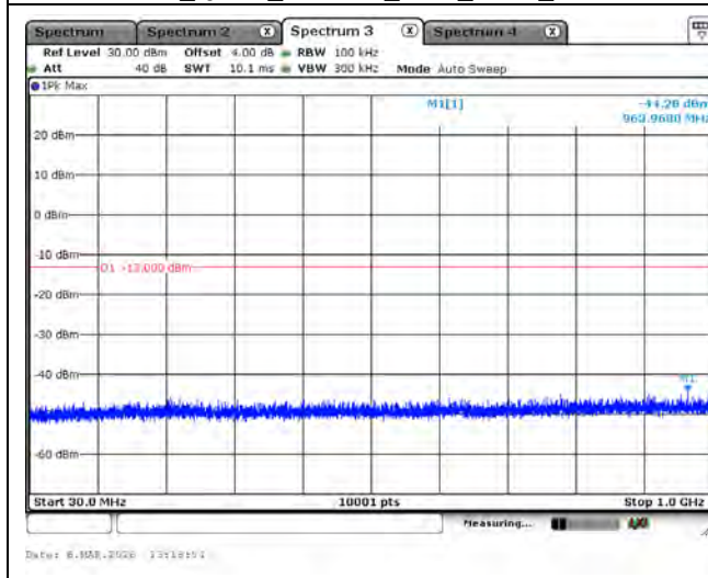
LTE Band 66_QPSK_1779.3M_1.4M_1RB0_Below 1GHz
