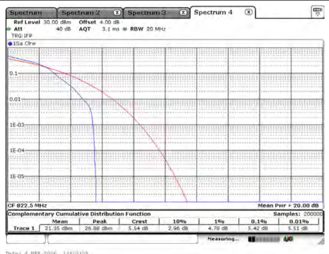
LTE Band 26 (Part 90)_16-QAM_822.5M_3M_1RB0
