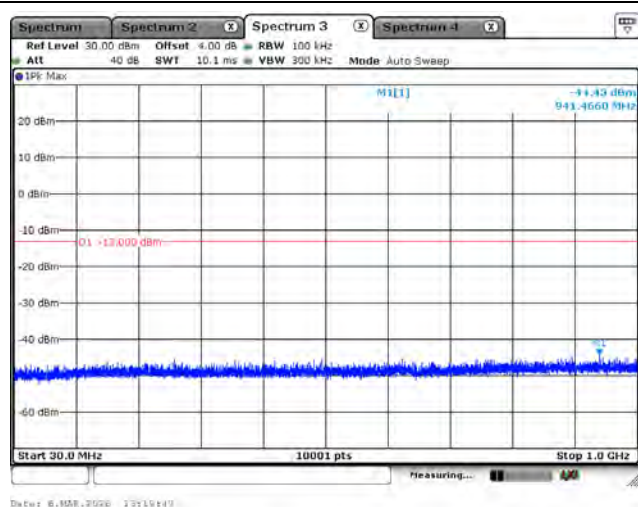
LTE Band 66_QPSK_1778.5M_3M_1RB0_Below 1GHz
