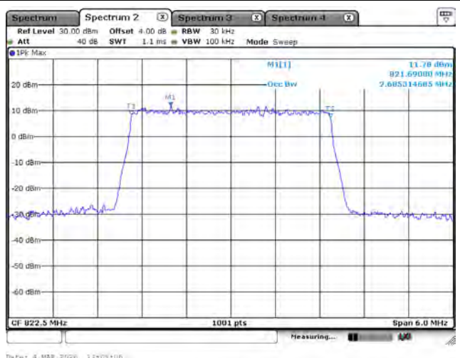
LTE Band 26 (Part 90)_16-QAM_822.5M_3M_FRB
