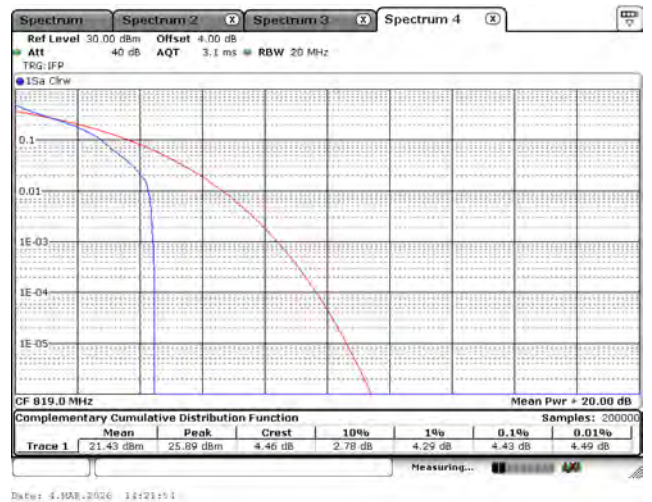
LTE Band 26 (Part 90)_QPSK_819M_5M_1RB0
