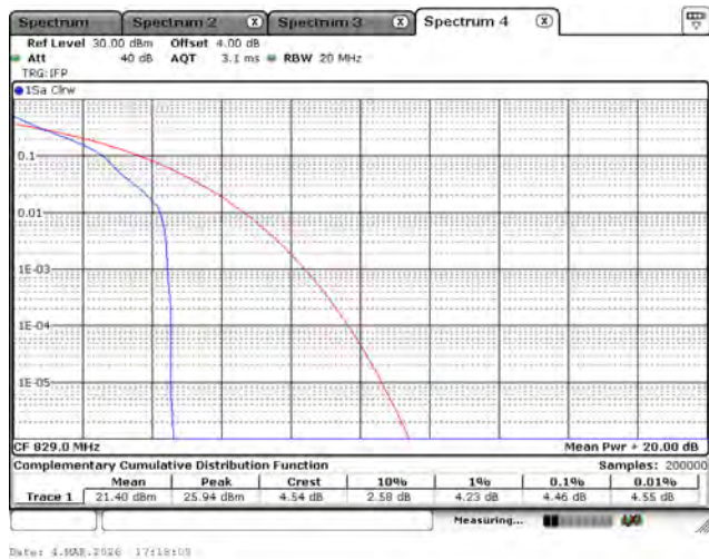
LTE Band 26 (Part 22)_QPSK_829M_10M_1RB0
