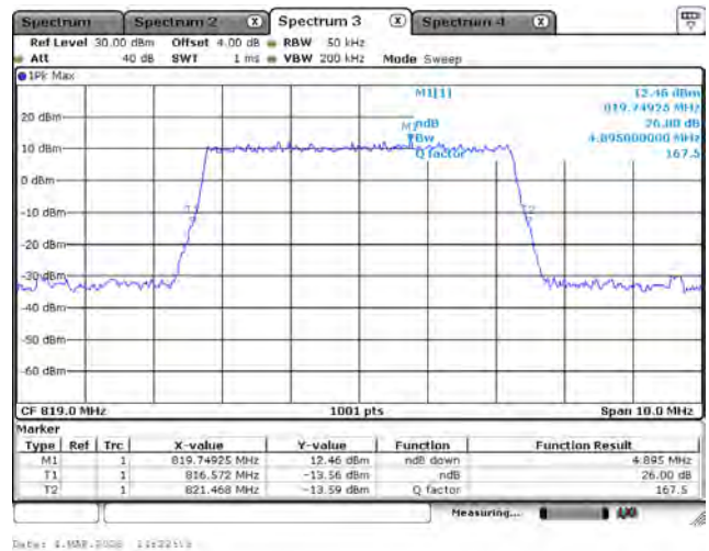
LTE Band 26 (Part 90)_QPSK_819M_5M_FRB
