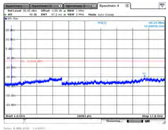
LTE Band 66_QPSK_1745M_3M_1RB0_Above 1GHz
