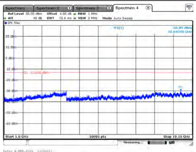
LTE Band 25_QPSK_1913.5M_3M_1RB0_Above 1GHz
