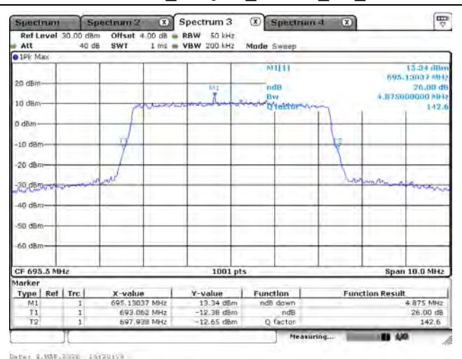
LTE Band 71_16-QAM_695.5M_5M_FRB
