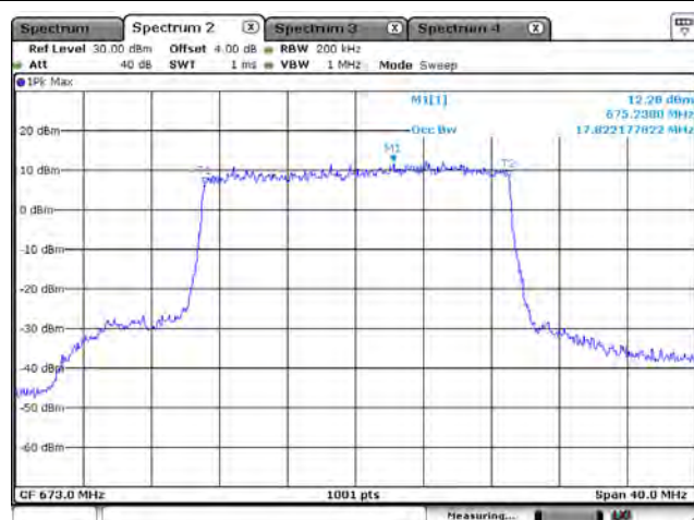
LTE Band 71_16-QAM_673M_20M_FRB
