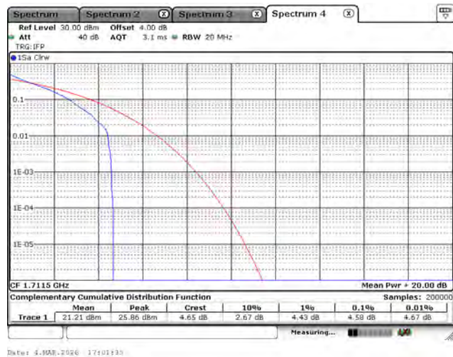
LTE Band 66_QPSK_1711.5M_3M_1RB0
