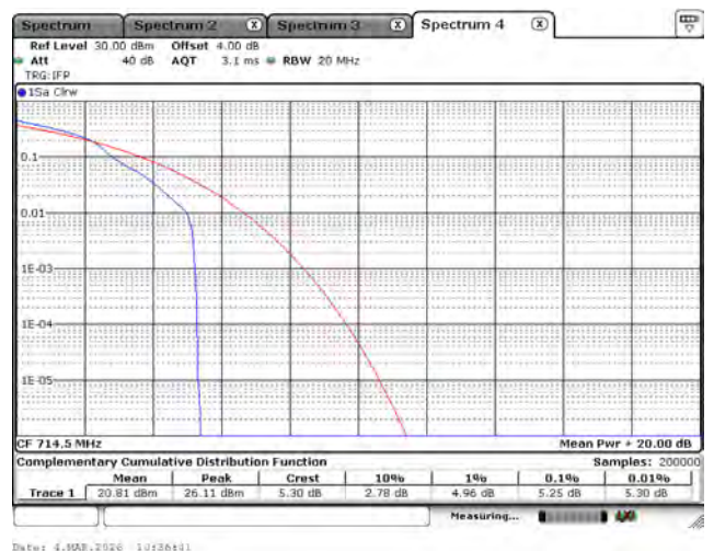
LTE Band 12_16-QAM_714.5M_3M_1RB0
