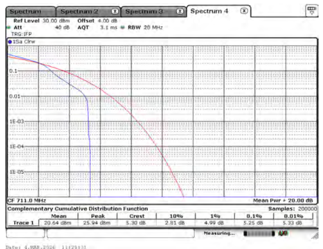
LTE Band 12_16-QAM_711M_10M_1RB0
