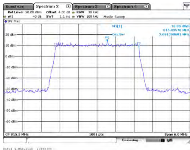
LTE Band 26 (Part 90)_QPSK_815.5M_3M_FRB
