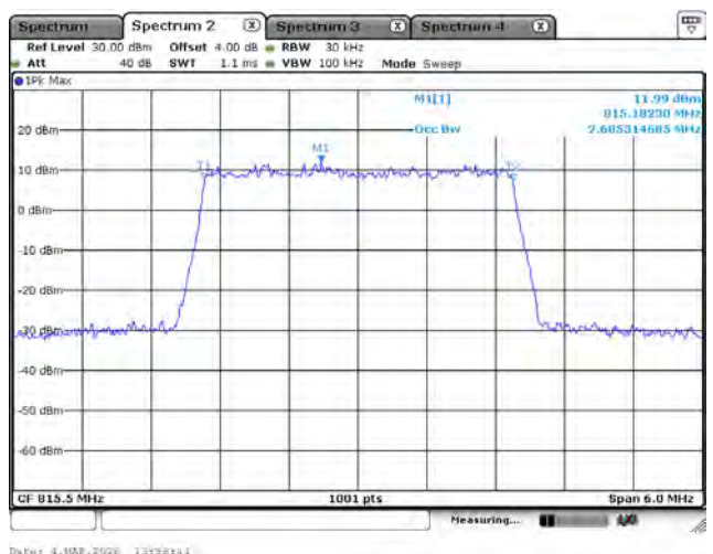
LTE Band 26 (Part 90)_16-QAM_815.5M_3M_FRB
