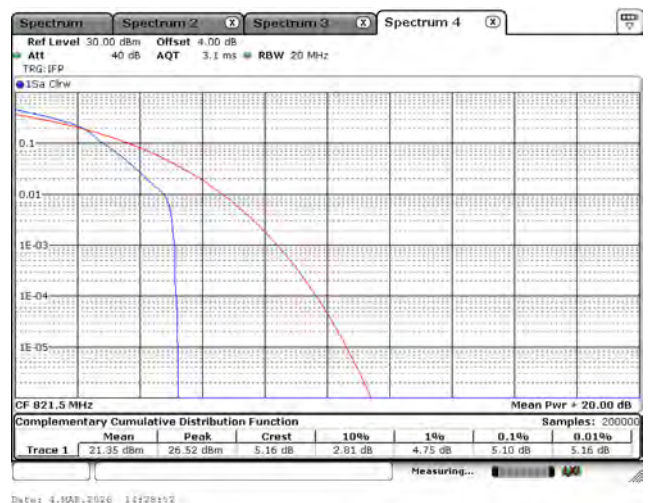
LTE Band 26 (Part 90)_16-QAM_821.5M_5M_1RB0
