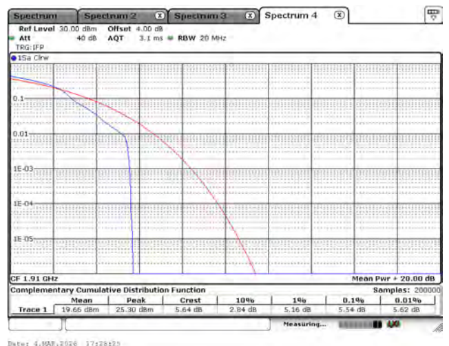
LTE Band 25_16-QAM_1910M_10M_1RB0
