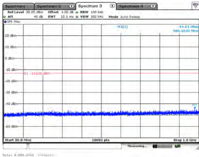
LTE Band 25_QPSK_1882.5M_5M_1RB0_Below 1GHz
