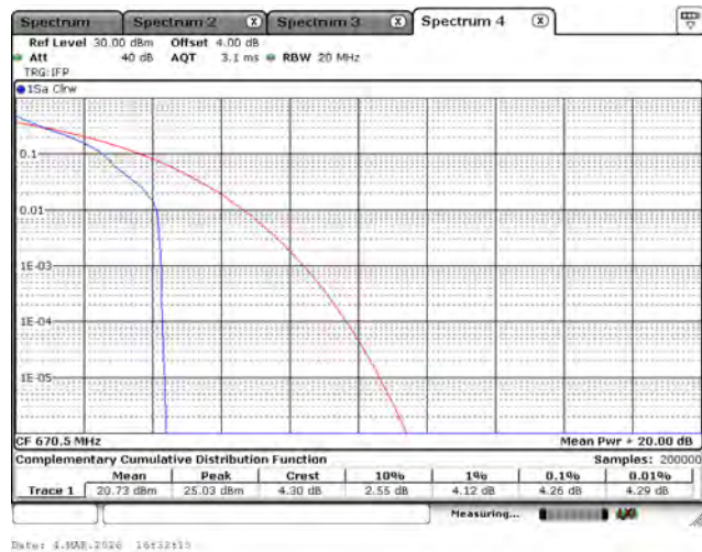
LTE Band 71_QPSK_670.5M_15M_1RB0
