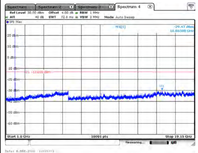
LTE Band 25_QPSK_1882.5M_10M_1RB0_Above 1GHz
