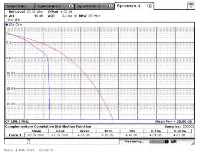
LTE Band 71_QPSK_680.5M_15M_1RB0
