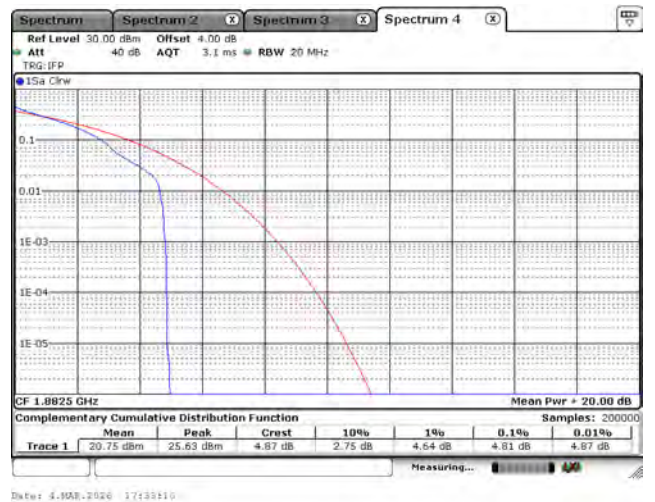
LTE Band 25_QPSK_1882.5M_5M_1RB0
