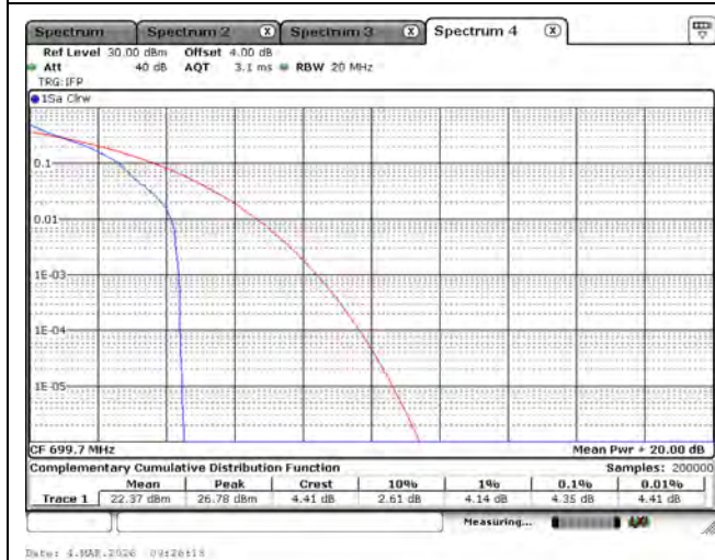
LTE Band 12_QPSK_699.7M_1.4M_1RB0
