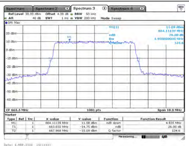
LTE Band 71_16-QAM_665.5M_5M_FRB
