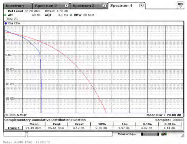
LTE Band 26 (Part 22)_QPSK_836.5M_10M_1RB0
