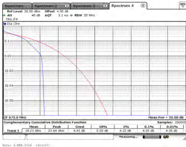
LTE Band 71_QPSK_673M_20M_1RB0
