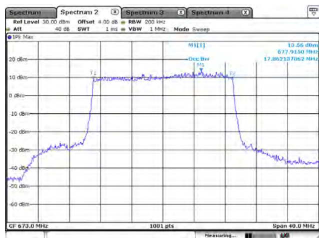
LTE Band 71_QPSK_673M_20M_FRB
