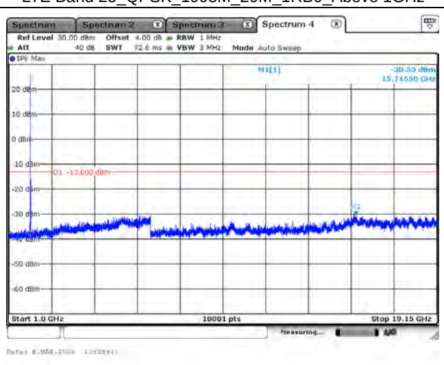
LTE Band 25_QPSK_1905M_20M_1RB0_Above 1GHz
