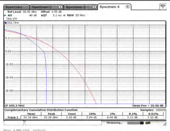
LTE Band 71_16-QAM_695.5M_5M_1RB0
