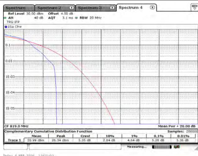
LTE Band 26 (Part 90)_16-QAM_819M_3M_1RB0
