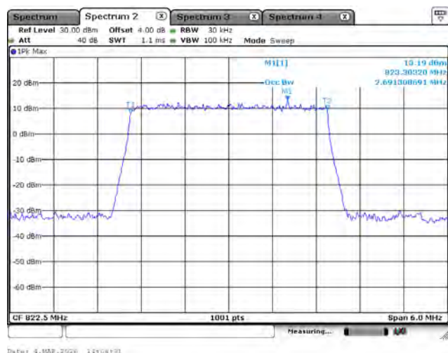
LTE Band 26 (Part 90)_QPSK_822.5M_3M_FRB
