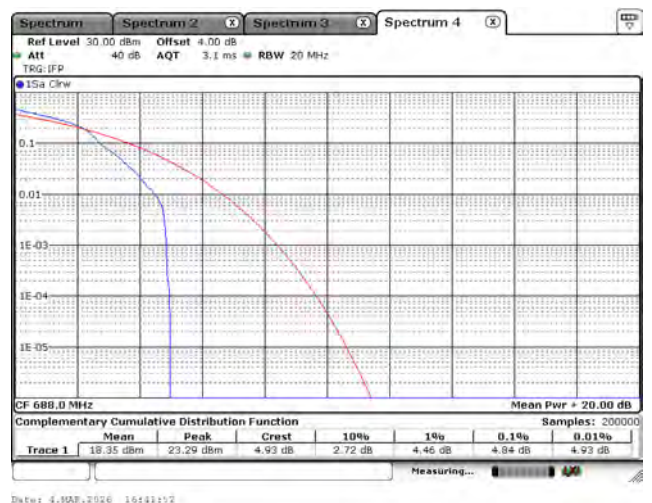
LTE Band 71_16-QAM_688M_20M_1RB0
