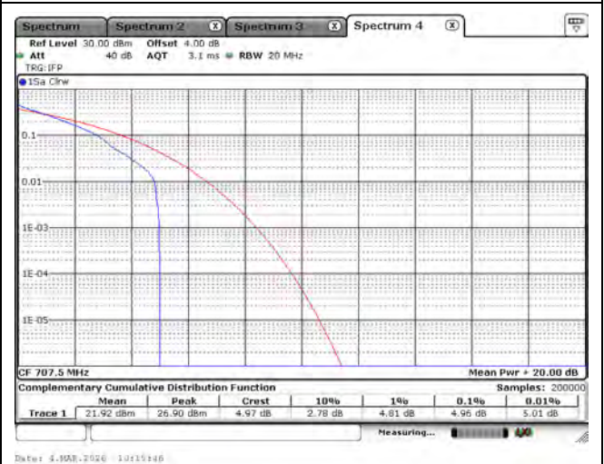
LTE Band 12_QPSK_707.5M_1.4M_1RB0
