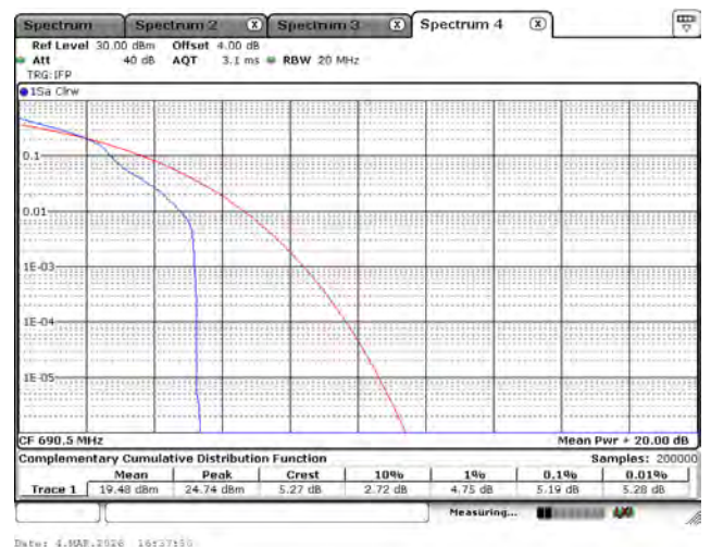
LTE Band 71_16-QAM_690.5M_15M_1RB0
