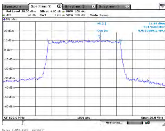
LTE Band 71_16-QAM_693M_10M_FRB
