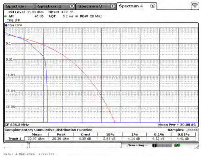
LTE Band 26 (Part 22)_QPSK_836.5M_15M_1RB0
