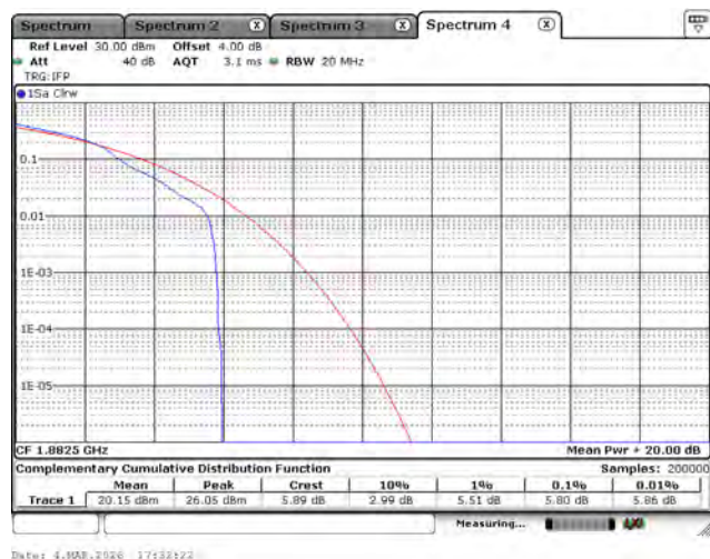
LTE Band 25_16-QAM_1882.5M_3M_1RB0
