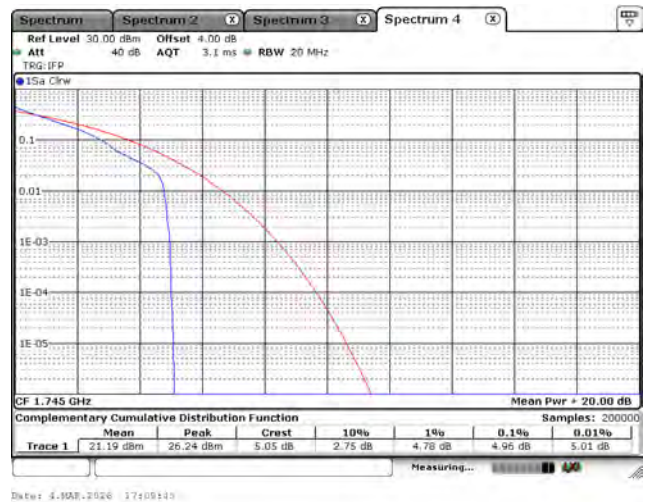
LTE Band 66_QPSK_1745M_5M_1RB0
