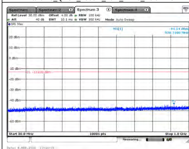
LTE Band 25_QPSK_1882.5M_20M_1RB0_Below 1GHz
