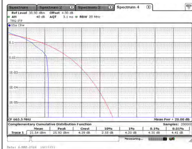
LTE Band 71_QPSK_665.5M_5M_1RB0
