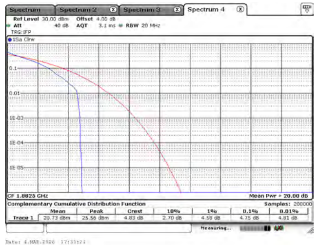
LTE Band 25_QPSK_1882.5M_10M_1RB0
