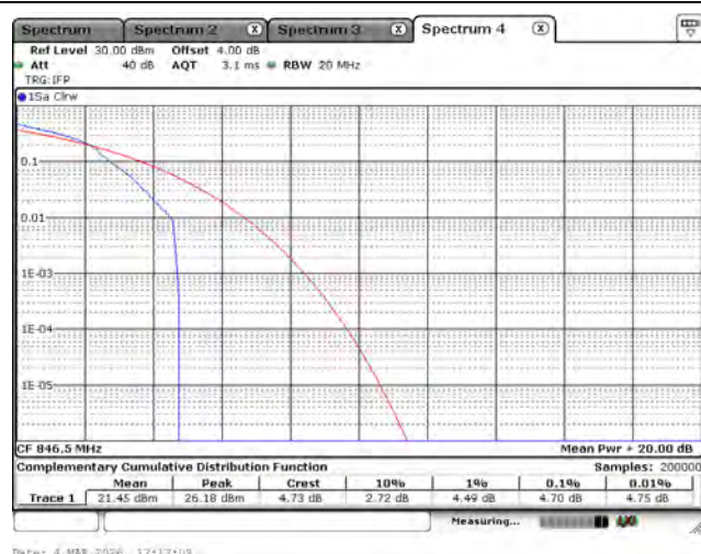
LTE Band 26 (Part 22)_16-QAM_846.5M_5M_1RB0
