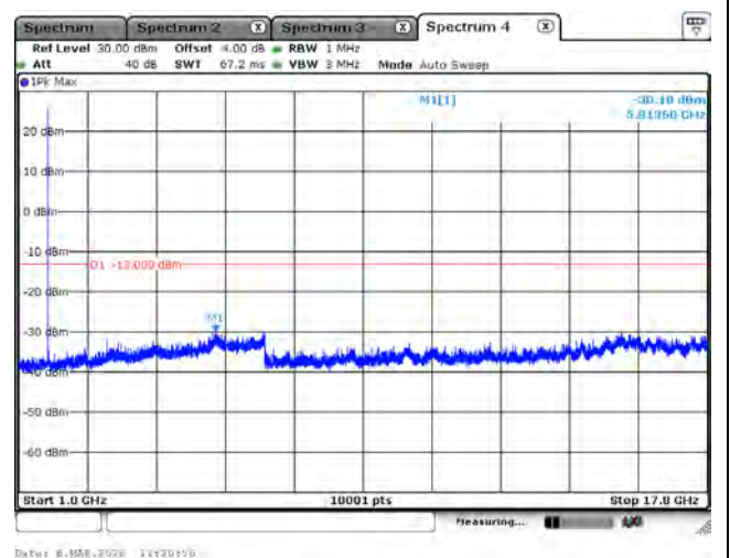
LTE Band 66_QPSK_1745M_1.4M_1RB0_Above 1GHz
