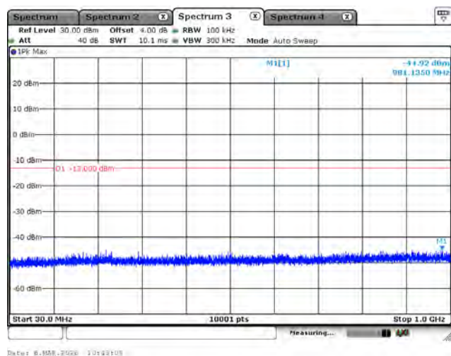
LTE Band 25_QPSK_1882.5M_10M_1RB0_Below 1GHz
