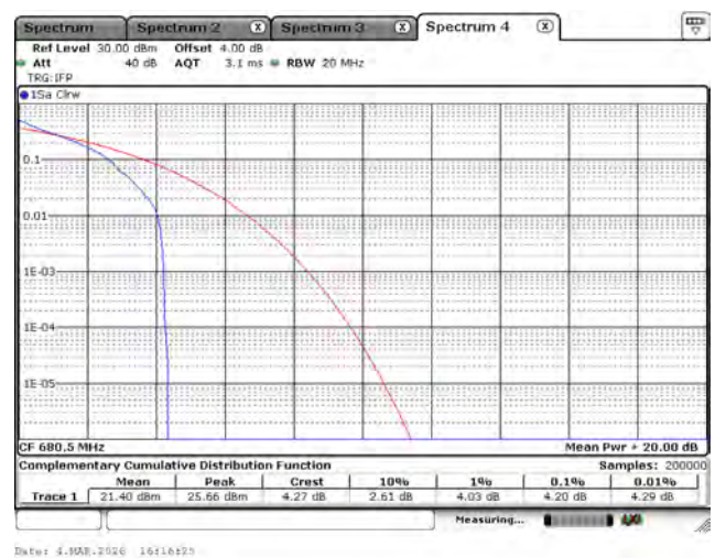
LTE Band 71_QPSK_680.5M_5M_1RB0
