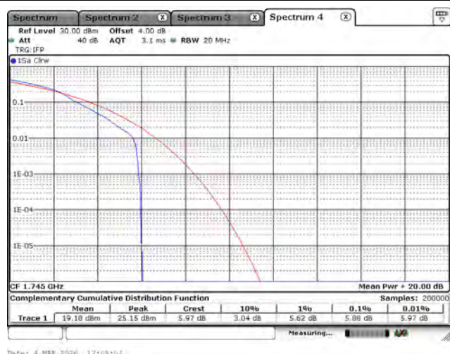
LTE Band 66_16-QAM_1745M_15M_1RB0
