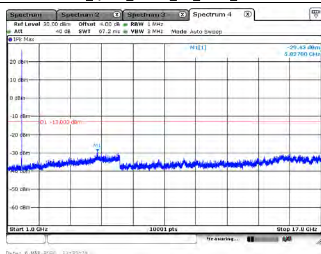
LTE Band 66_QPSK_1745M_5M_1RB0_Above 1GHz
