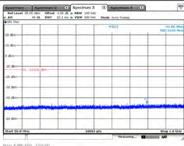
LTE Band 25_QPSK_1910M_10M_1RB0_Below 1GHz
