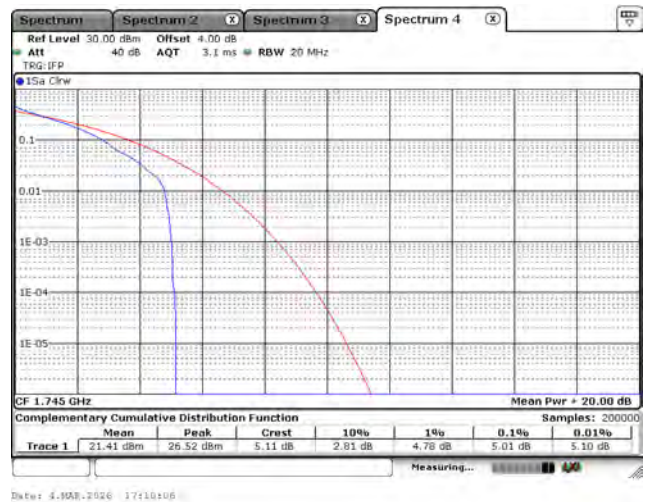
LTE Band 66_QPSK_1745M_3M_1RB0
