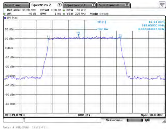
LTE Band 26 (Part 90)_QPSK_819M_5M_FRB
