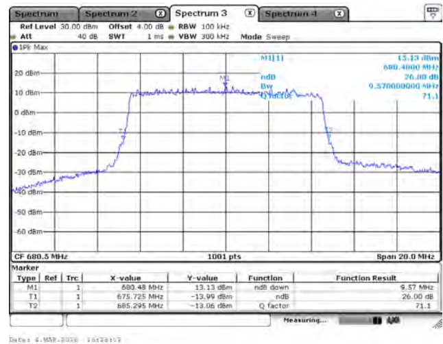
LTE Band 71_QPSK_680.5M_10M_FRB
