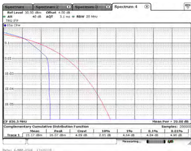
LTE Band 26 (Part 22)_16-QAM_836.5M_3M_1RB0
