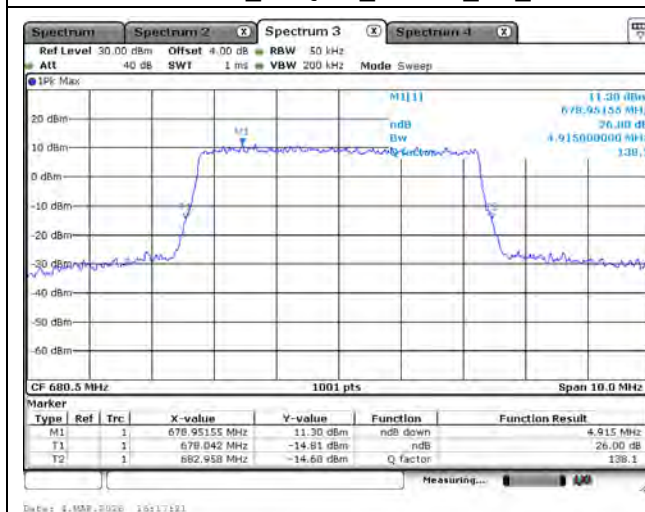
LTE Band 71_16-QAM_680.5M_5M_FRB
