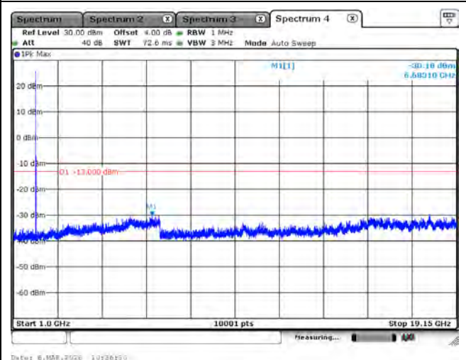
LTE Band 25_QPSK_1910M_10M_1RB0_Above 1GHz
