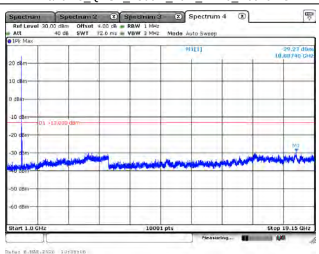
LTE Band 25_QPSK_1882.5M_20M_1RB0_Above 1GHz
