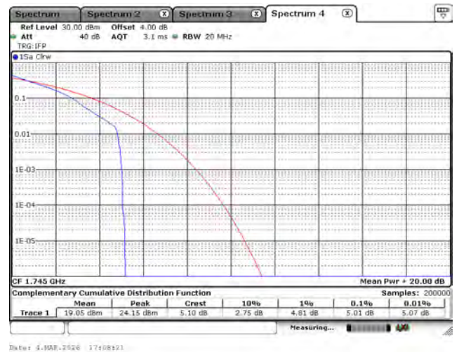
LTE Band 66_QPSK_1745M_20M_1RB0
