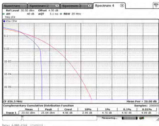
LTE Band 26 (Part 22)_16-QAM_836.5M_10M_1RB0
