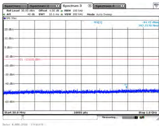
LTE Band 25_QPSK_1913.5M_3M_1RB0_Below 1GHz
