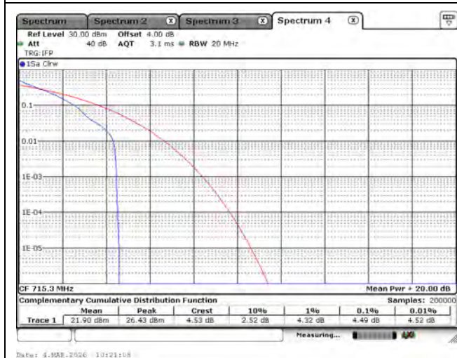
LTE Band 12_QPSK_715.3M_1.4M_1RB0
