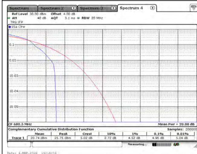
LTE Band 71_16-QAM_680.5M_5M_1RB0
