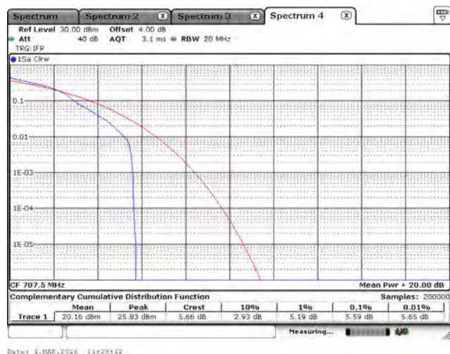
LTE Band 12_16-QAM_707.5M_10M_1RB0
