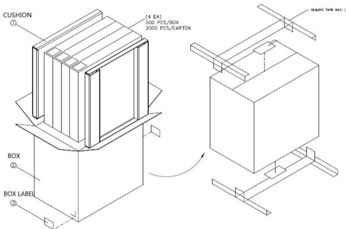
Figure 29. Packing—carton
