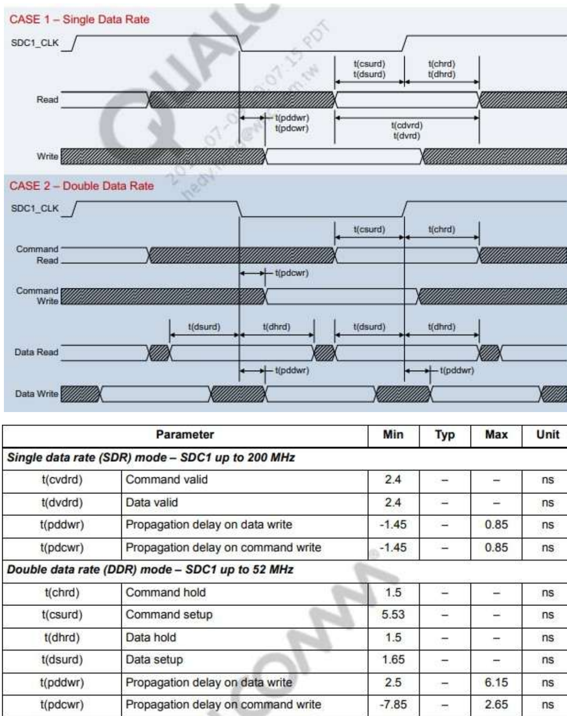
Figure 17. SDIO timing
