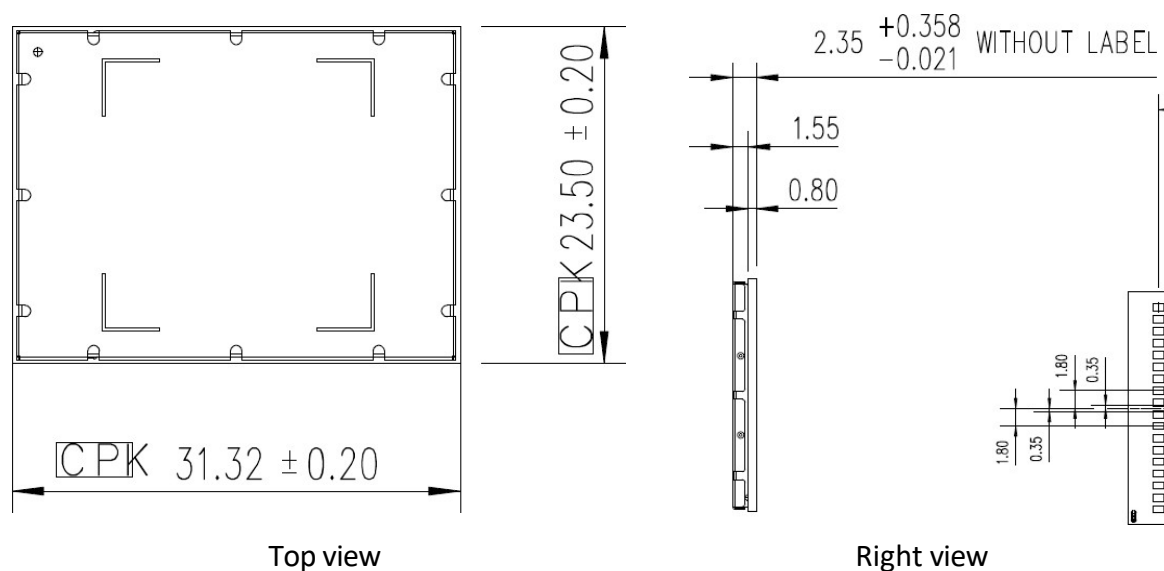
Figure 21. PCBA dimension
