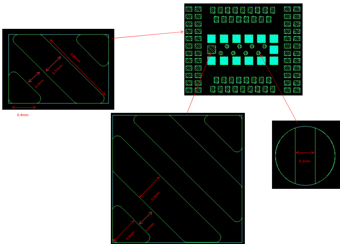
Figure 26. Stencil-foil drawing
