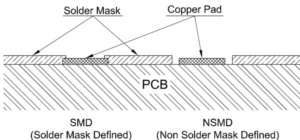
Figure 24. NSMD solder pad design
