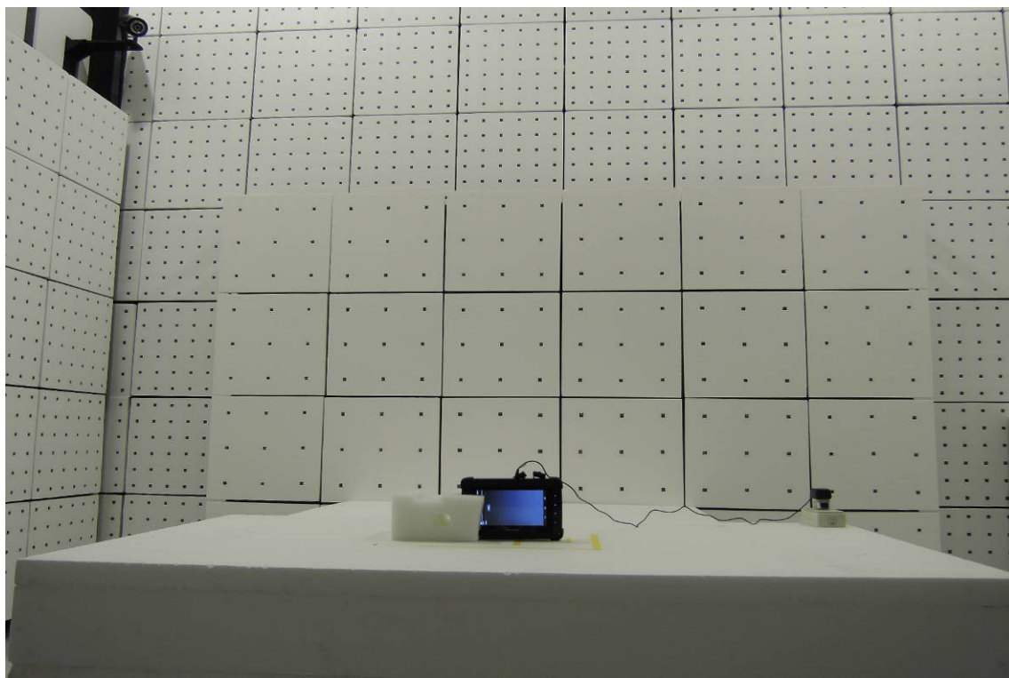
Radiated Emission Setup Photos (10~30MHz)
