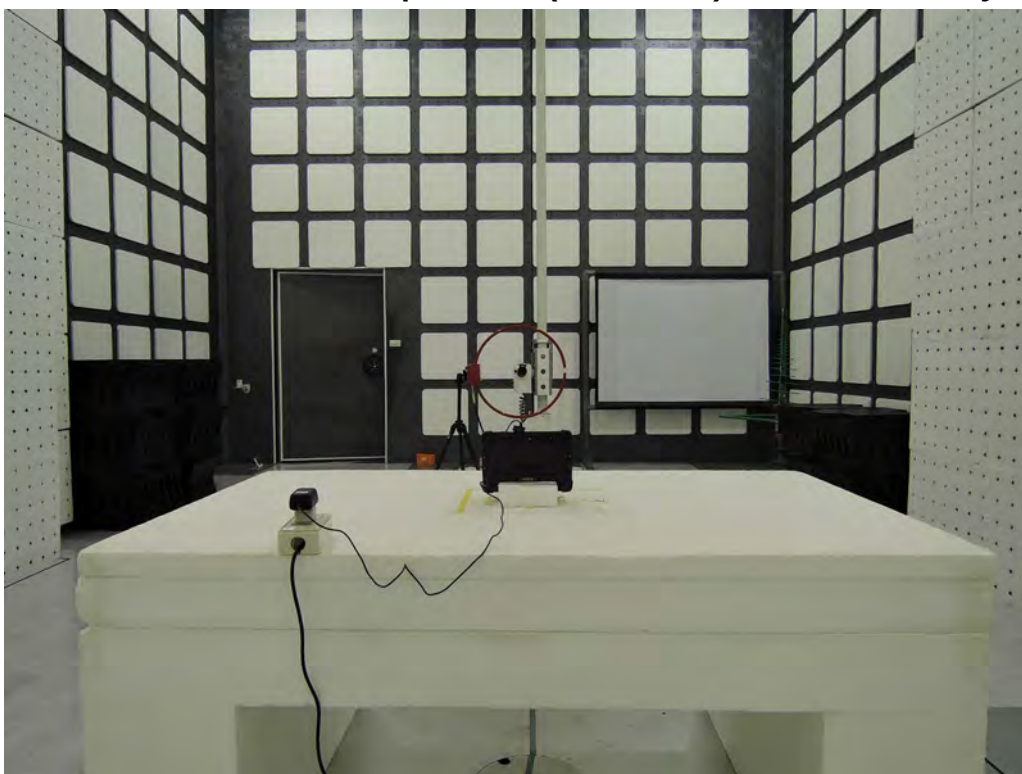
Radiated Emission Setup Photos (10~30MHz) Horizontal Plority
